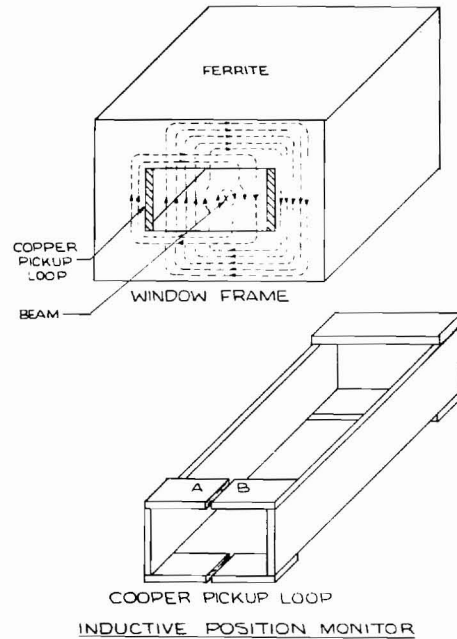
Fig. 11 Beam Position Monitor
