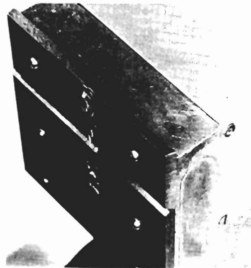
Fig. 9. 10 MeV Emittance Head.
