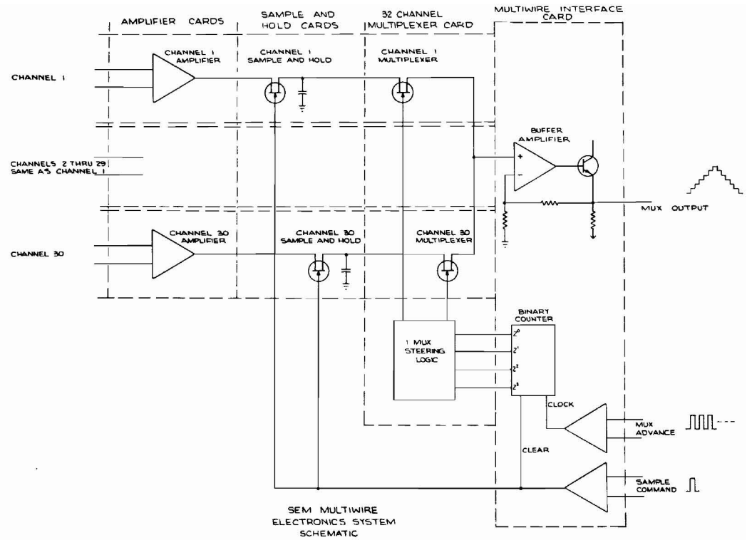
Fig. 8. Multiwire SEM/Electronics System Schematic
