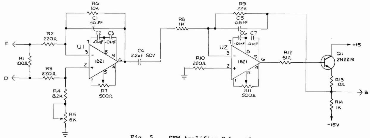
Fig. 5. SEM Amplifier Schematic
