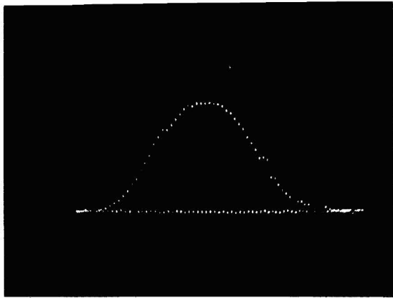
SINGLE WIRE SCAN. POSITION HEBT 6 2.6 CM FWHH (0.5 MM/STEP)
