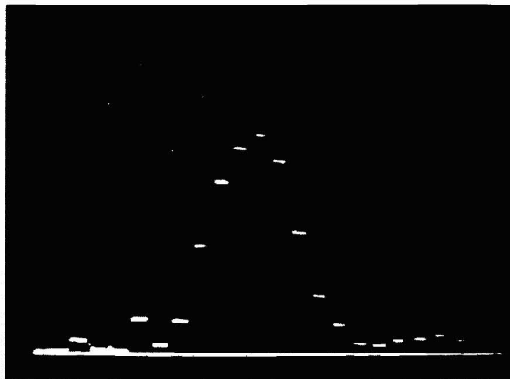
MULTI WIRE MONITOR POSITION HEBT 6 2.6 CM FWHH (5 MM/CHANNEL)
