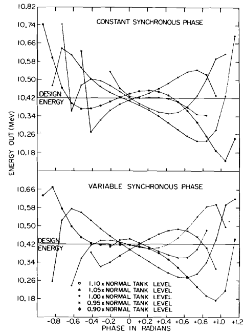
Fig. 6 Phase-amplitude plot for tank 1.
