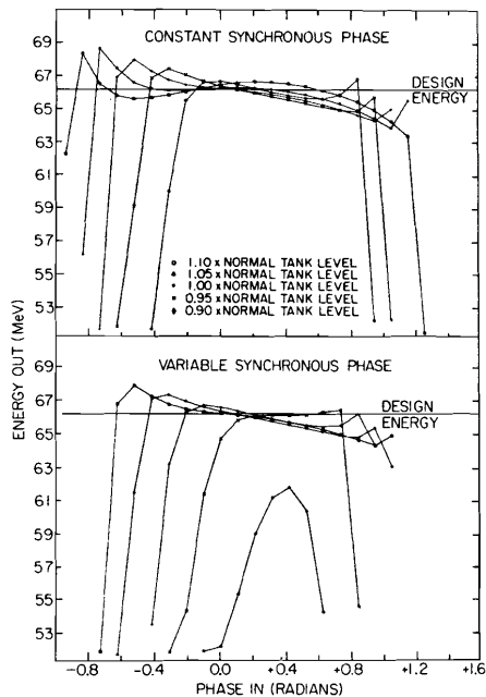
Fig. 8 Phase-amplitude plot for tank 3.
