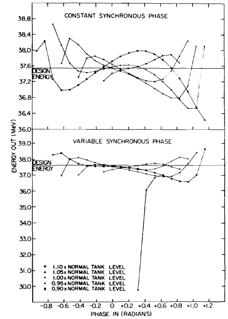
Fig. 7 Phase-amplitude plot for tank 2.
