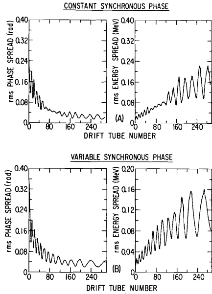
Fig. 5 Rms phase and energy spread as function of drift-tube number for 0 current, \pm 25 keV initial energy spread.
