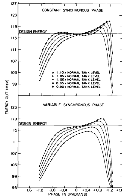
Fig. 9 Phase-amplitude plot for tank 5.
