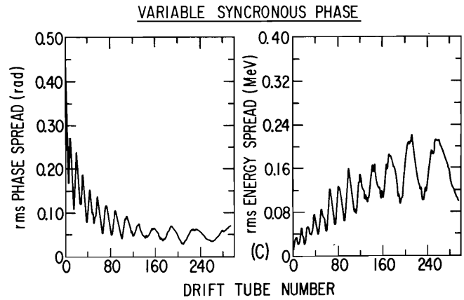
Figure 3. Rms phase and energy spread as function of drift-tube number for zero current and zero initial energy spread.
