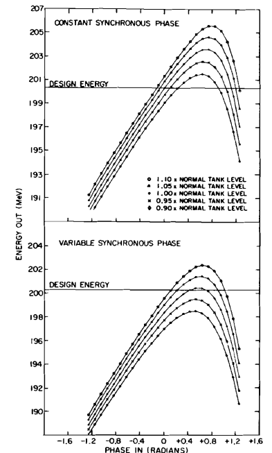
Fig. 10 Phase-amplitude plot for tank 9.
