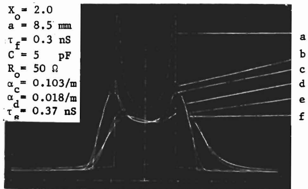
Fig. 5 Waveforms with Successive Attenuations
