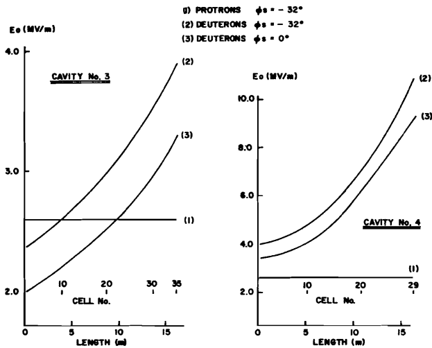
Fig. 4 Average electric field required in cavity Nos. 3 and 4 of BNL and NAL linacs.
