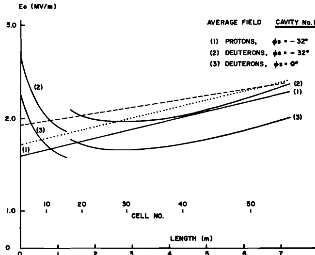
Fig. 2 Average electric field required in cavity No. 1 of BNL and NAL linacs. Broken line is suggested field variation for deuteron accelerations. Dotted line shows field level used at BNL.
