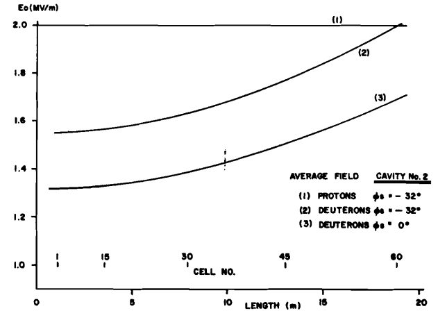
Fig. 3 Average electric field required in cavity No. 2 of BNL and NAL linacs.
