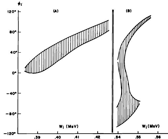
Fig. 5 Favorable range of the injection energy and the injection phase for a deuteron acceleration in BNL and NAL linacs. Average electric field assumed given by Fig. 2 broken line.
