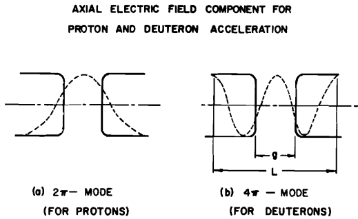
Fig. 1. Electric field for accelerating (a) protons and (b) deuterons.
