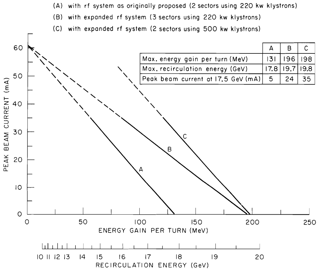
Figure 3. Load-line diagrams comparing three different RF systems. System parameters are similar to those given for Case 1 in Tables I and II at a phase angle of 30^\circ .
