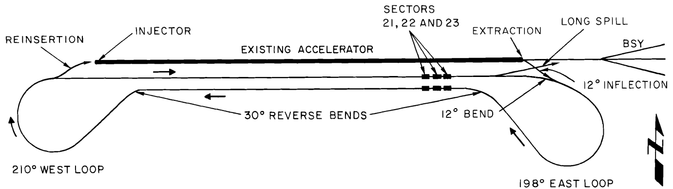
Figure 1. Schematic layout of the recirculating linear accelerator.
