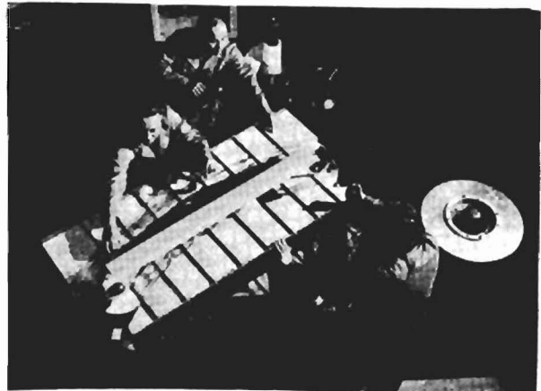
Fig. 2. 55° magnet coil forming operation.
