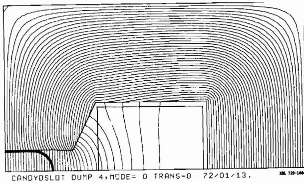
Fig. 6. 55° magnet flux plot.
