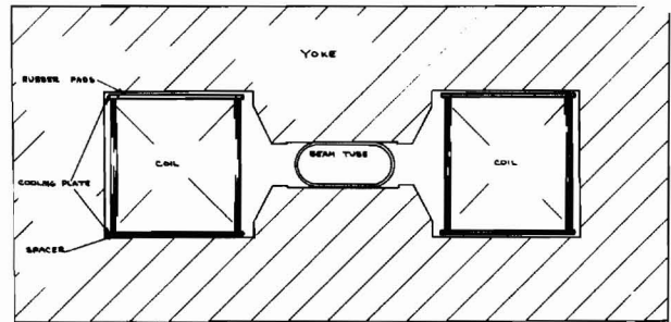
Fig. 7. Typical magnet cross section.
