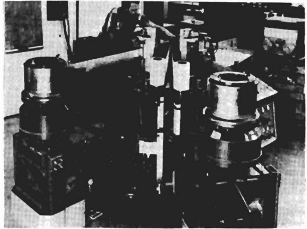
Fig. 1. Coil winder set-up for quadrupole coils.
