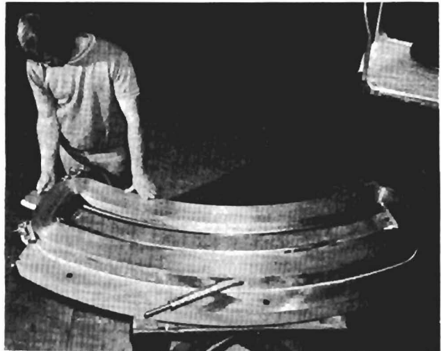
Fig. 3. 55° magnet subassembly.
