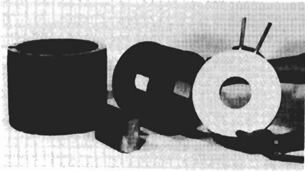
Fig. 4. Quadrupole components.
