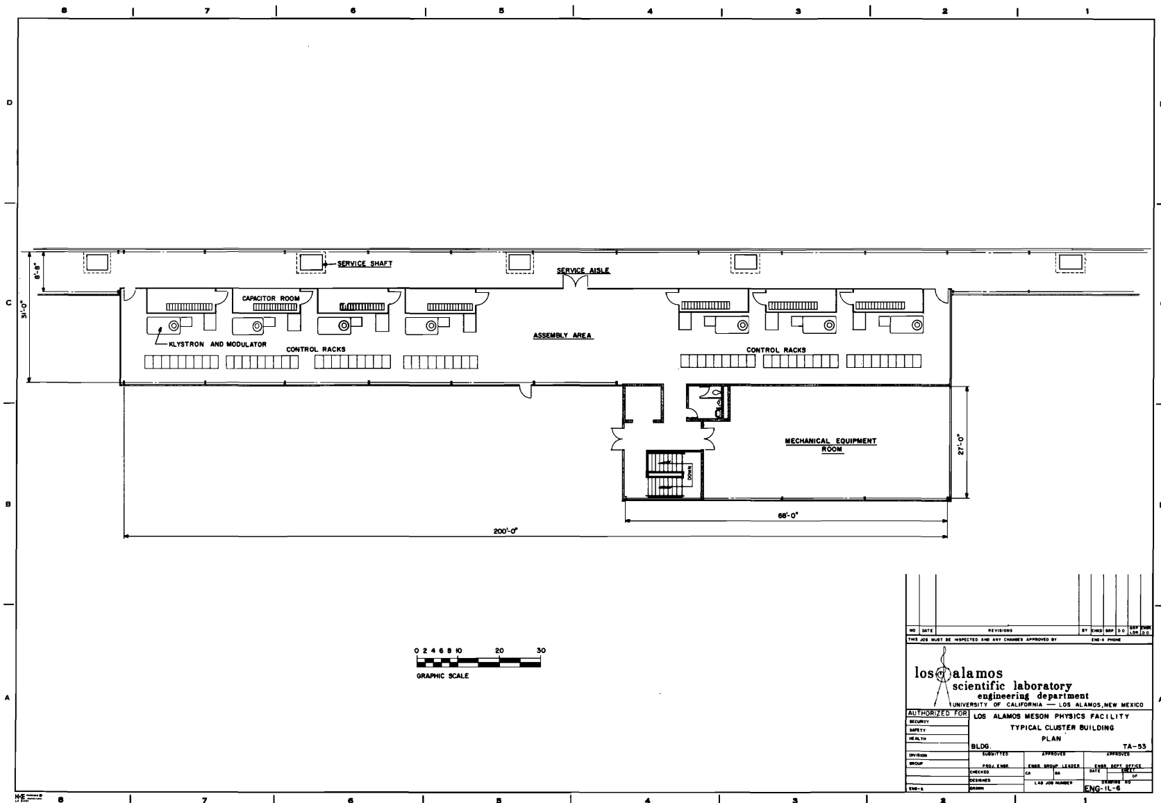
Figure 6 — Typical cluster building.
