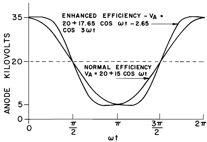
FIGURE 5: Gridded Power Tube Anode Voltage Waveforms
