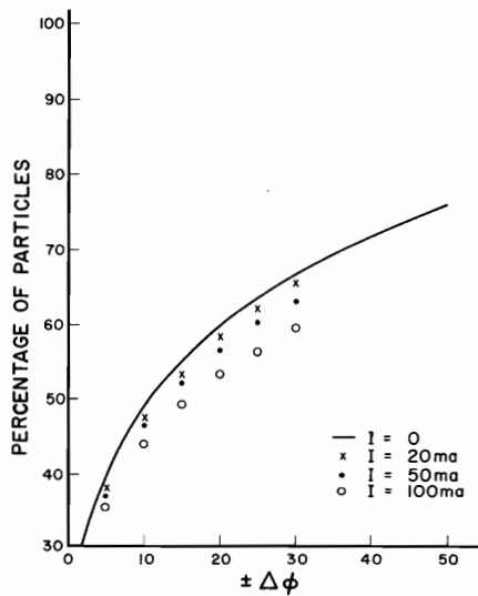
Fig. 7. Comparison of space-charge effects on the maximum percentage of particles that can be bunched within a phase of \pm \Delta\phi and for a voltage of 20 kV on the cavity, using a single-cavity buncher.
