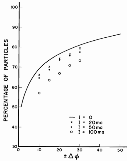
Fig. 6. Comparison of space-charge effects on the maximum percentage of particles that can be bunched within a phase of \pm \Delta\phi and for a voltage of 20 kV on the first cavity, using a two-gap harmonic buncher.
