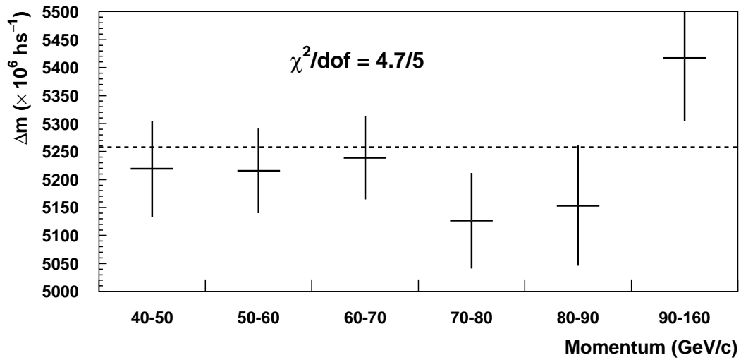
Figure A.15: \Delta m in momentum bins using the K \rightarrow \pi^0 \pi^0 sample. The first five data points are 10 GeV/c momentum bins. The last bin is 90-160 GeV/c. The dashed line indicates the value for the full data sample.
