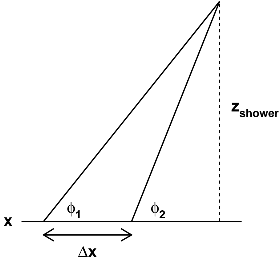
Figure 4.3: Cartoon of position shift to correct for differing incident angles. A shower with incident angle \phi_1 will reach shower maximum at the same position as a shower with angle \phi_2 shifted by \Delta x .
