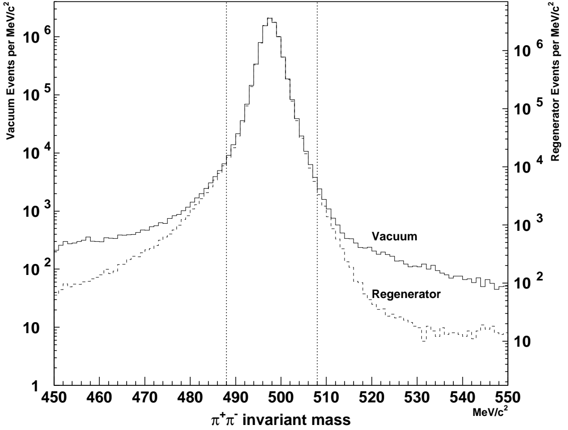
Figure 3.4: Invariant mass distributions for \pi^+\pi^- data for both beams after all other analysis cuts are applied. The dotted lines show where our cuts are made. Figure courtesy of J. Graham[2].
