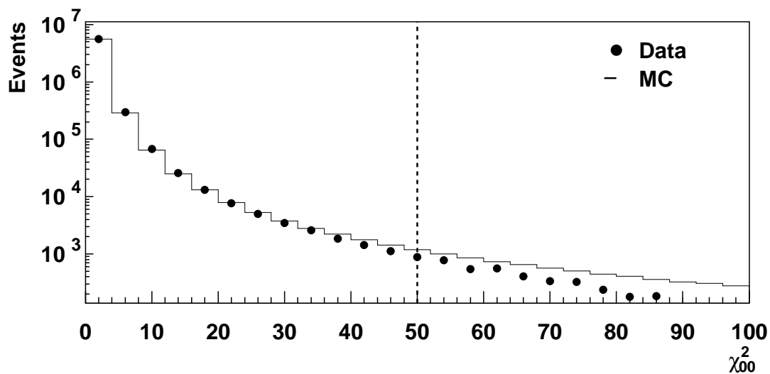
Figure 7.12: \chi_{\pi^0}^2 for vacuum beam K \rightarrow \pi^0 \pi^0 data and MC. The data is background subtracted. The dashed line indicates the value of our nominal cut.
