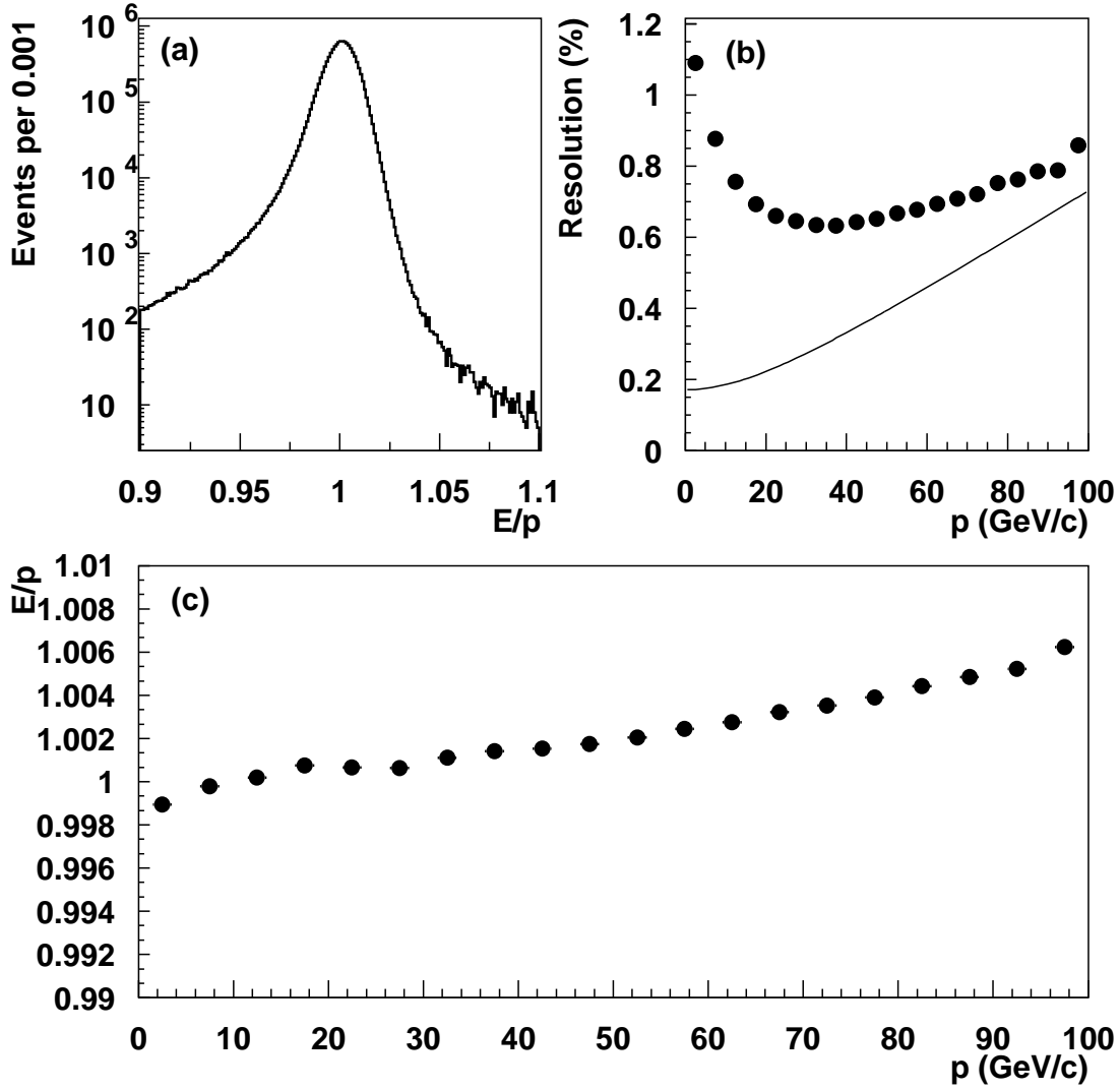
Figure 2.16: Electron calibration plots for all 3100 CsI channels for a sample calibration period from 1999. (a) E/p distribution. (b) E/p resolution as a function of momentum. The fine curve shows the contribution from momentum resolution. (c) E/p as a function of momentum.
