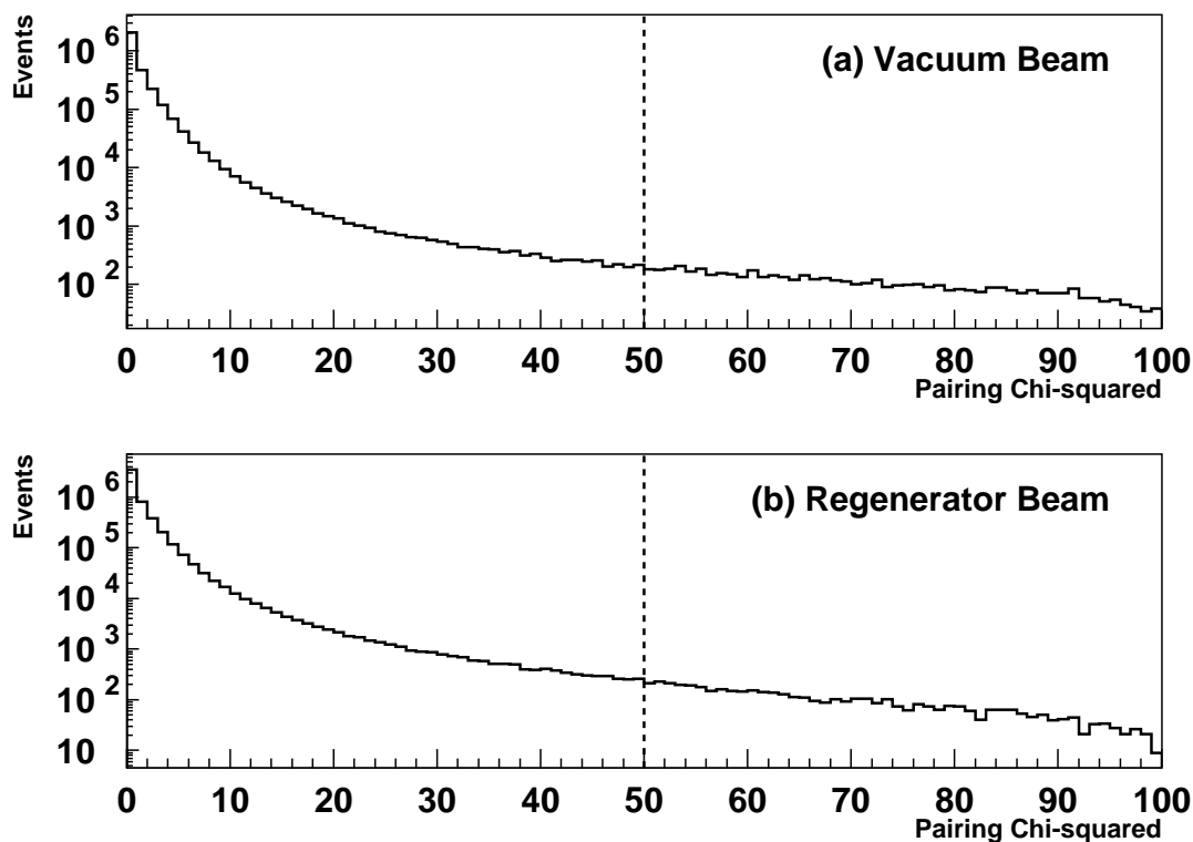
Figure 3.25: K \rightarrow \pi^0 \pi^0 \chi^2_{\pi^0} distributions for 1999. The dashed line indicates our cut.
