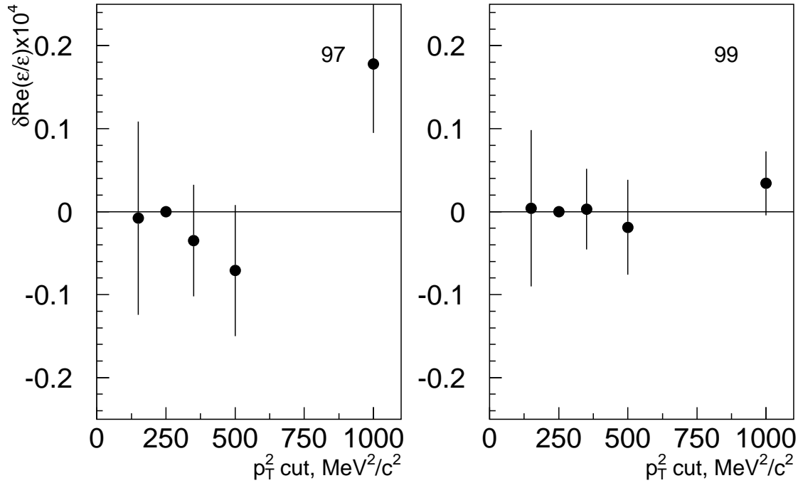
Figure 7.7: Change in Re(\epsilon'/\epsilon) with variation of p_T^2 cut for 1997 (left) and 1999 (right). The nominal requirement is p_T^2 < 250 \text{ MeV}^2/\text{c}^2 .
