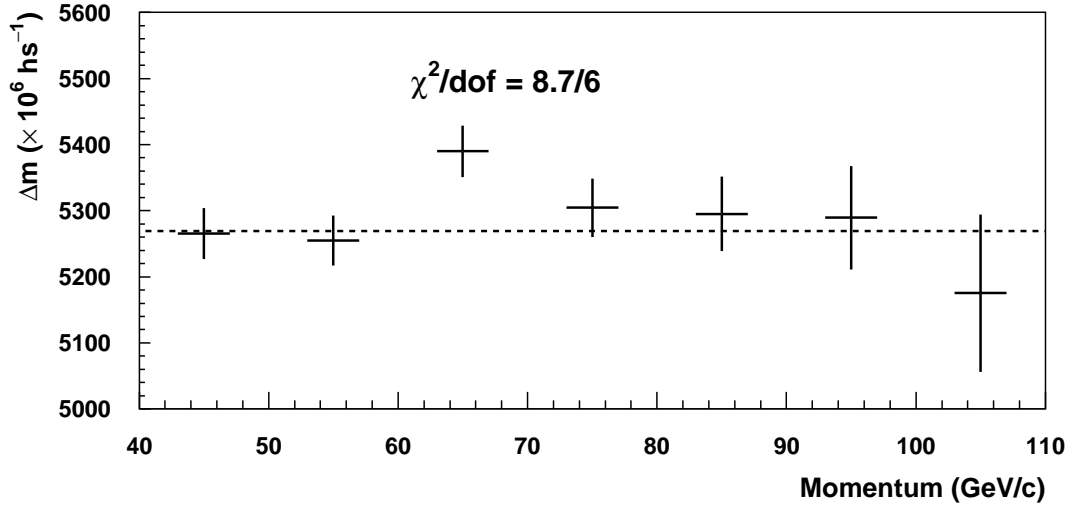
Figure A.13: \Delta m in 10 GeV/c momentum bins using the K \rightarrow \pi^+\pi^- sample. Note that there are no fits above 110 GeV/c. The dashed line indicates the value for the full data sample.
