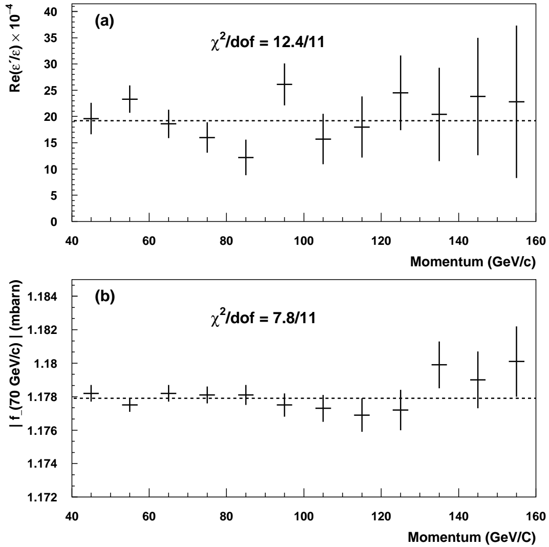
Figure 8.3: (a) \text{Re}(\epsilon'/\epsilon) and (b) |f_-(70 \text{ GeV}/c)| in 10 GeV/c momentum bins. The dashed line indicates the value for the full data sample.
