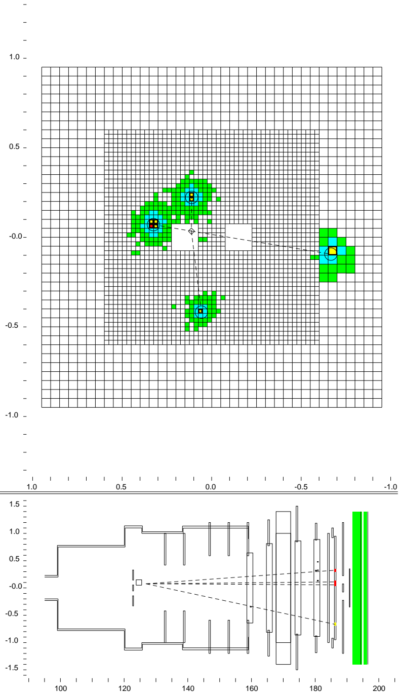
Figure 3.20: Event display for a sample K \rightarrow \pi^0 \pi^0 decay. The four clusters of energy in the CsI are shown. The cluster energies, reconstructed decay vertex, reconstructed m_{\pi^0 \pi^0} invariant mass, and \chi^2_{\pi^0} are shown on the left. The bottom panel shows the photon trajectories from the decay vertex to the CsI. The x-position of the vertex is in the same beam as the regenerator, so this event is consistent with a K_S decay.
