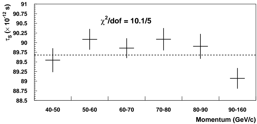
Figure A.16: \tau_S in momentum bins using the K \rightarrow \pi^0 \pi^0 sample. The first five data points are 10 GeV/c momentum bins. The last bin is 90-160 GeV/c. The dashed line indicates the value for the full data sample.
