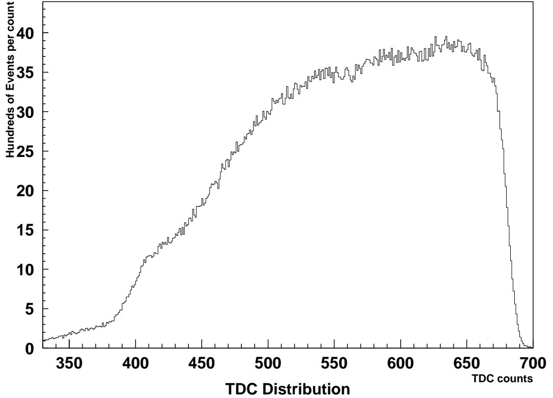
Figure 2.12: Sample drift chamber TDC distribution. The common-stop edge is seen at \sim 680 TDC counts and the plateau of the distribution is seen from 550-680 counts. Figure courtesy of J. Graham[2].
