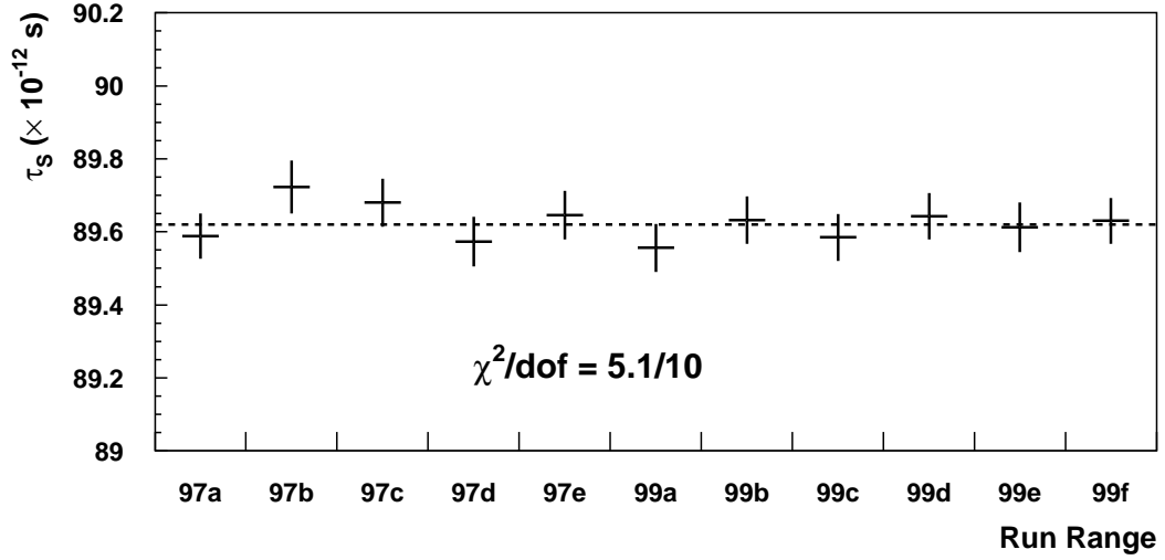
Figure A.2: \tau_S in subsets of the K \rightarrow \pi^+\pi^- data sample. Each point is statistically independent. The dashed line indicates the value of \tau_S for the full data sample.
