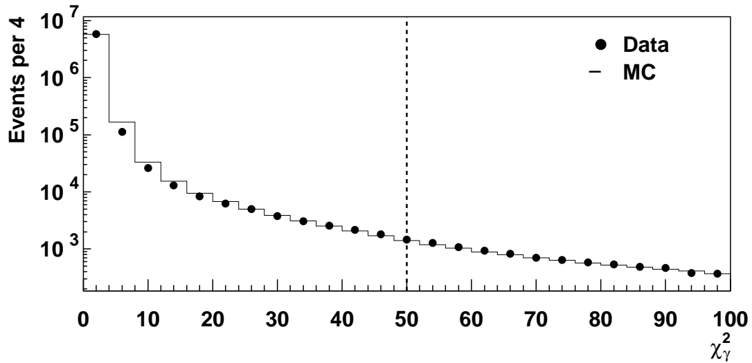
Figure 7.11: \chi^2_\gamma for vacuum beam K \rightarrow \pi^0 \pi^0 data and MC. The data is background subtracted. The dashed line indicates the value of our nominal cut.
