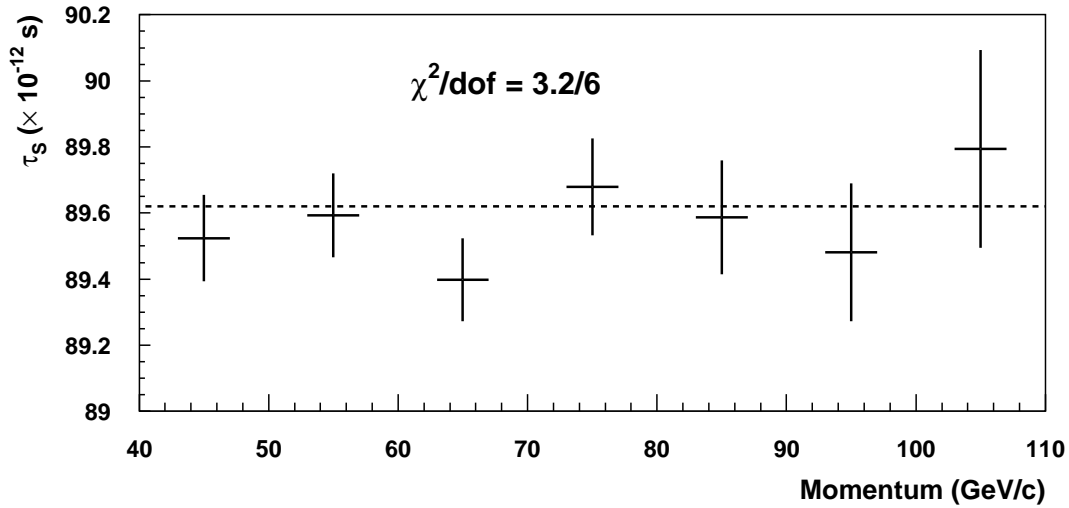
Figure A.14: \tau_S in 10 GeV/c momentum bins using the K \rightarrow \pi^+\pi^- sample. Note that there are no fits above 110 GeV/c. The dashed line indicates the value for the full data sample.
