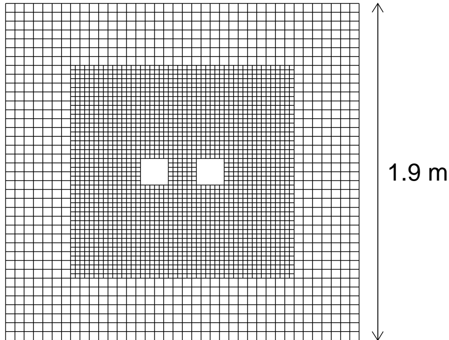
Figure 2.5: Transverse view of the KTeV CsI calorimeter, showing the small inner crystals, the large outer crystals, and the beam pipes.
