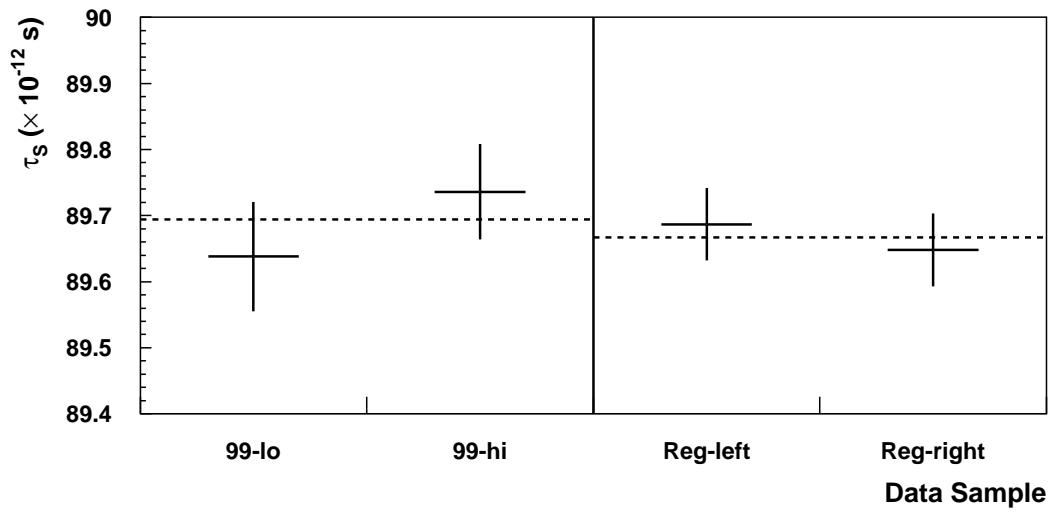
Figure A.10: \tau_S consistency with beam intensity and regenerator position for the K \rightarrow \pi^0 \pi^0 sample. The low intensity sample has an average SEM of 4 \times 10^{12} and the high intensity sample has an average SEM of 6.5 \times 10^{12} . These subsets are for the 1999 data only. Reg-left and reg-right refer to the position of the regenerator beam in the detector. These subsets are for the full data sample. The dashed lines indicate the value of \tau_S in the appropriate full data sample.
