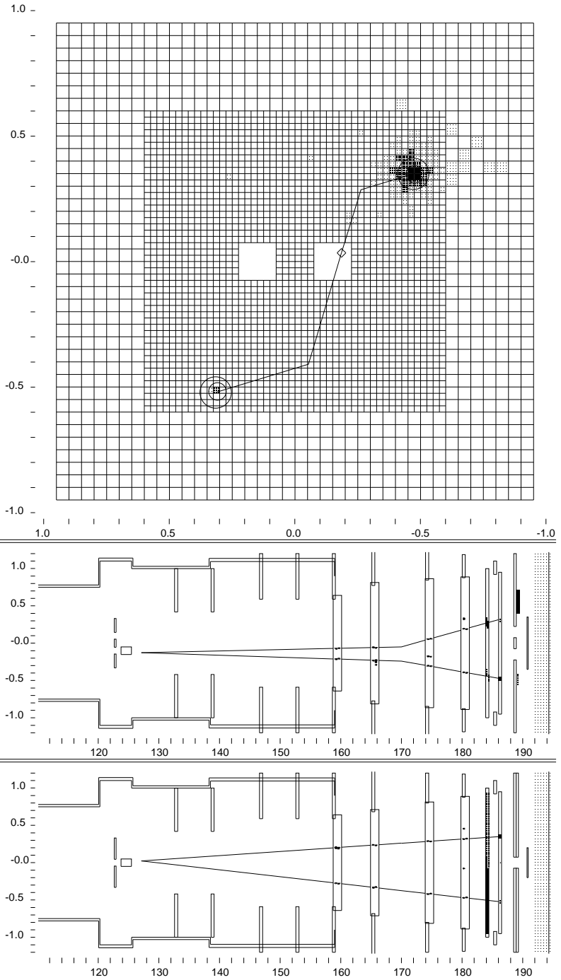
Figure 3.3: Event display for a K \rightarrow \pi^+ \pi^- event. The top panel shows the clusters of energy in the calorimeter with matching track projections. The middle panel shows the x view of the tracks with the bend at the analysis magnet. The bottom panel shows the straight y tracks. In the middle panel the decay vertex is seen to be within the regenerator beam. Figure courtesy of J. Graham[2].
