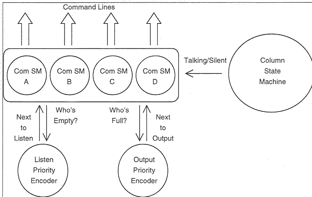
Figure 23: A Schematic Overview of the End-of-column Logic
