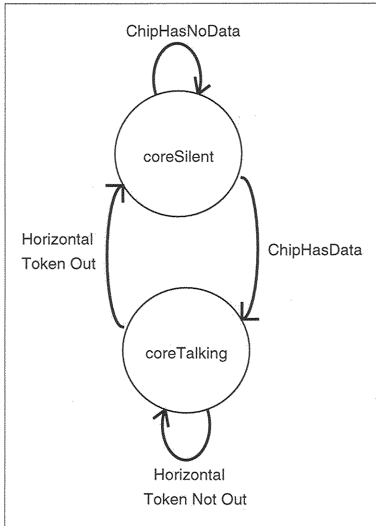
Figure 38: Core State Diagram
