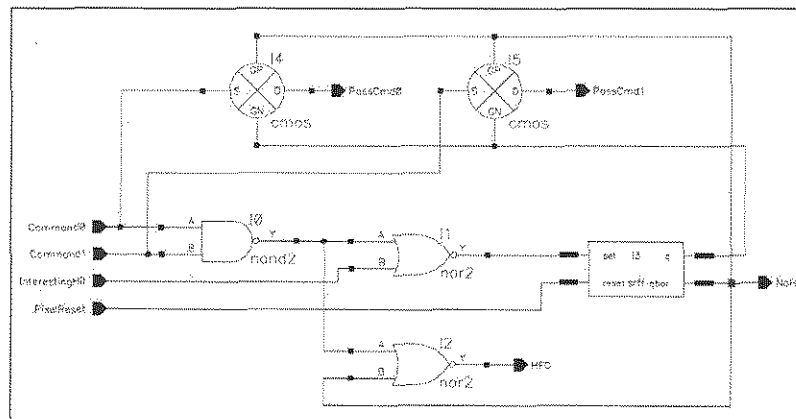
Figure 10: A Schematic of the Front Command Cell
