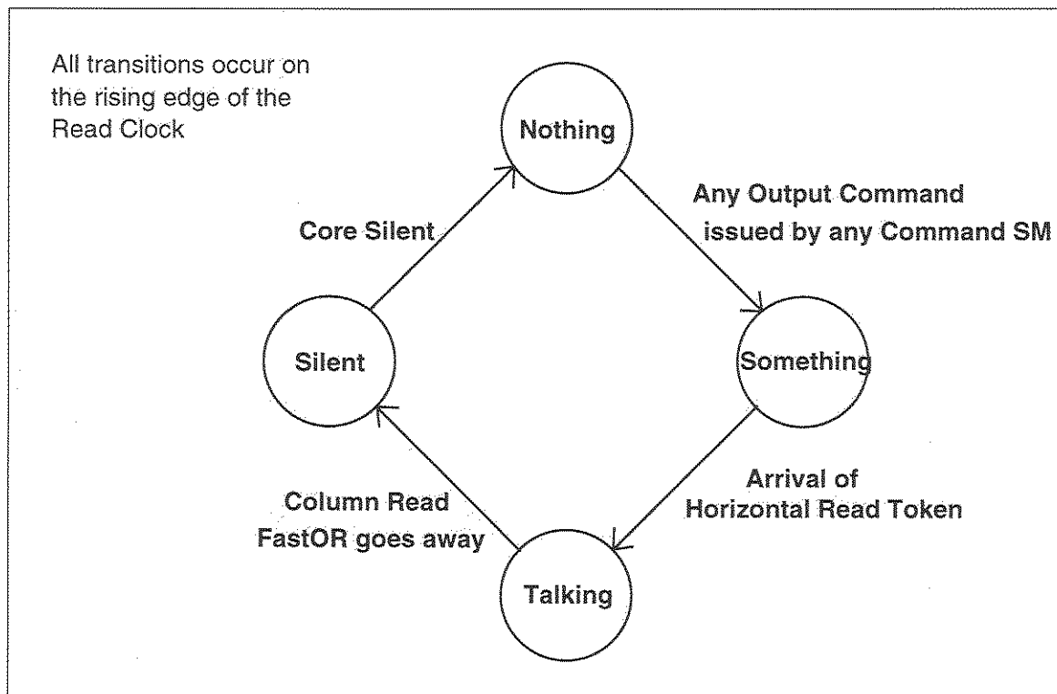
Figure 28: The Column State Machine State Diagram
