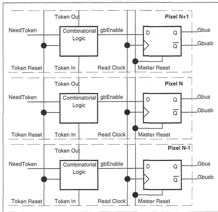
Figure 18: The Interactions of several Token Control Logic Cells
