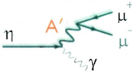
Figure 10. Feynman diagram of an \eta meson decaying to a photon ( \gamma ) and a dark photon, denoted by A' , with a probability governed by the square of the coupling constant between light and dark sectors, \epsilon^2 . The A' can subsequently decay into a \mu^+\mu^- pair with a decay lifetime proportional to \epsilon^{-2} .
