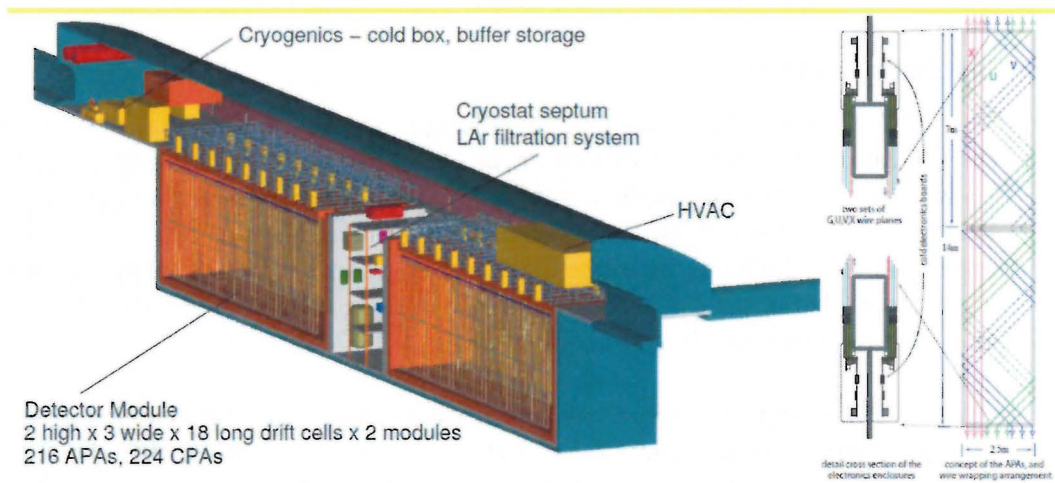
FIGURE 16. Schematic of a 34-kt fiducial mass LArTPC design (left). The detector comprises two 17-kt fiducial mass LArTPC detectors. The design of a pair of Anode Plane Assemblies is shown at right.
