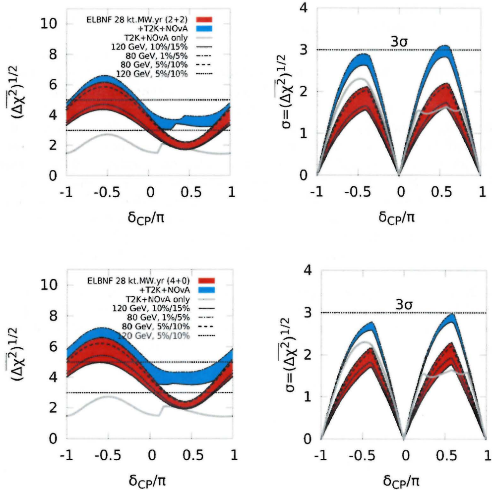
FIGURE 14: Expected sensitivity of ELBNF28 to the determination of the neutrino mass ordering (left) and discovery of CP violation, i.e. \delta \neq 0, \pi , (right), alone (red), and in combination with NOvA and T2K (blue). In the top panels, the ELBNF28 data is divided equally between neutrino and antineutrino mode while for the bottom panels data is in neutrino mode only for the same exposure. Expected sensitivity for a combination of NOvA and T2K without ELBNF28 is indicated by the gray line. The T2K sensitivity is based on 7.8 \times 10^{21} protons-on-target (POT) in neutrino mode. The NOvA sensitivity is based on three years of running in neutrino and three years in antineutrino mode, where 6 \times 10^{20} POT per year are expected. The systematic uncertainties quoted are the uncorrelated signal/background normalization uncertainties for the \nu_e and \bar{\nu}_e samples; each configuration also includes 5%-10% signal/background normalization uncertainty on the muon neutrino and antineutrino samples. The curves on each band represent a range of beam designs and levels of systematic uncertainty, ranging from the 120-GeV FNAL beam with 10%-15%
