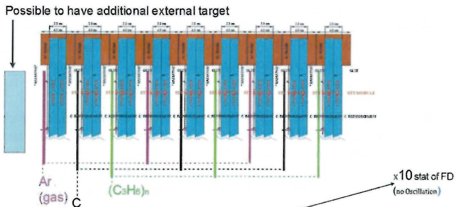
FIGURE 19: Schematic of nuclear targets (Ar, Ca, C, etc.) placed at the upstream end of the FGT. Note that pressurized Ar gas will be placed in aluminum tubes.
