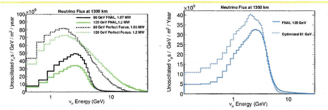
FIGURE 5: Unoscillated \nu_\mu flux at 1,300 km in units of neutrinos per GeV per square meter per year. The left panel shows the flux for the four beams described in the text: 120-GeV FNAL (solid green), 80-GeV FNAL (solid black), 120-GeV perfect focus (dashed green), and 60-GeV perfect focus (dashed black). The right panel shows the flux resulting from a preliminary attempt at further beam optimization (dashed) compared to the 120-GeV FNAL beam (solid). In all cases, the variation in beam power with proton beam energy is considered in the normalization.
