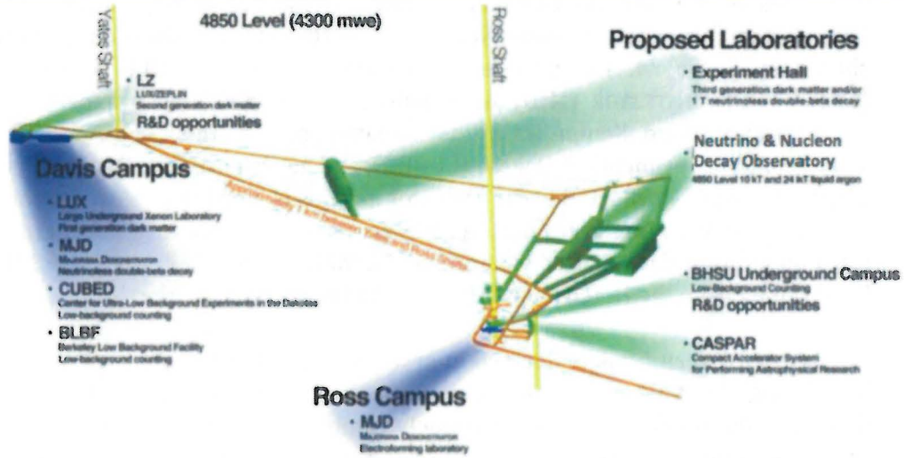
FIGURE 24. The 4850 level (4,300 mwe) of SURF, highlighting the existing and proposed experiments.
