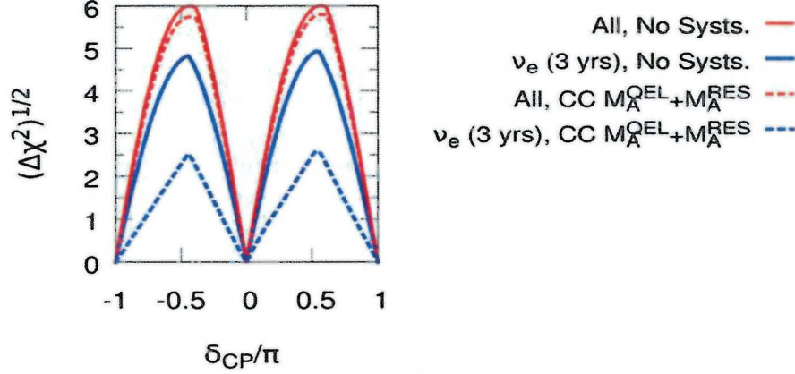
FIGURE 9: An example CP violation sensitivity calculated using inputs from the FastMC in a fit to all four ( \nu_e , \bar{\nu}_e , \nu_\mu , \bar{\nu}_\mu ) samples (red) and a fit to the \nu_e appearance sample only (blue), for the case of no systematic uncertainty (solid) and the case in which both M_A^{QE,CC} and M_A^{RES,CC} are allowed to vary with a 1\sigma uncertainty of 20% (dashed). This example was taken from an earlier LBNE study, so the absolute sensitivity cannot be compared with the sensitivities presented in this document.
