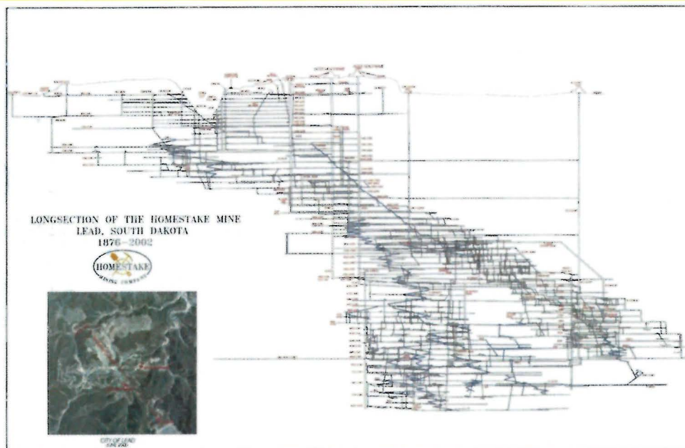
FIGURE 23. The long section of the former Homestake Gold Mine. This figure illustrates the 60 underground levels extending to greater than 8,000 feet below
