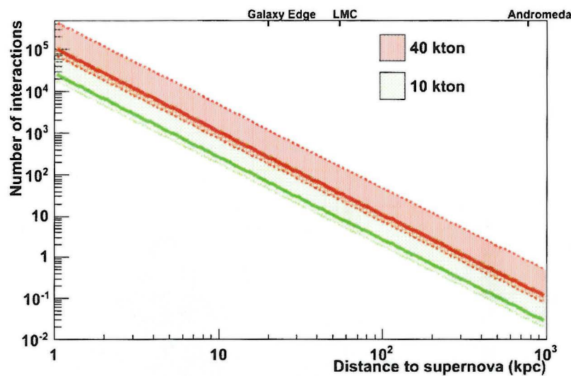
FIGURE 12: Estimated numbers of supernova neutrino interactions in the experiment as a function of distance to the supernova, for different detector masses ( \nu_e events dominate). The red dashed lines represent expected events for a 40-kt detector and the green dotted lines represent expected events for a 10-kt detector. The lines limit a fairly wide range of possibilities for “Garching-parameterized” supernova flux spectra (e.g [18]) with luminosity 0.5 \times 10^{52} ergs over ten seconds. The optimistic upper line of a pair gives the number of events for average \nu_e energy of \langle E_{\nu_e} \rangle = 12 MeV, and “pinching” parameter \alpha=2 ; the pessimistic lower line of a pair gives the number of events for \langle E_{\nu_e} \rangle = 8 MeV and \alpha=6 . (Note that the luminosity, average energy, and pinching parameters will vary over the time frame of the burst, and these estimates assume a constant spectrum. Oscillations will also affect the spectrum.) The solid lines represent the integrated number of events for the specific time-dependent neutrino flux model in [19]. (See Figure 13; this model has relatively cool spectra and low event rates). Core collapses are expected to occur a few times per century in this galaxy, at a most-likely distance of about 10-15 kpc.
