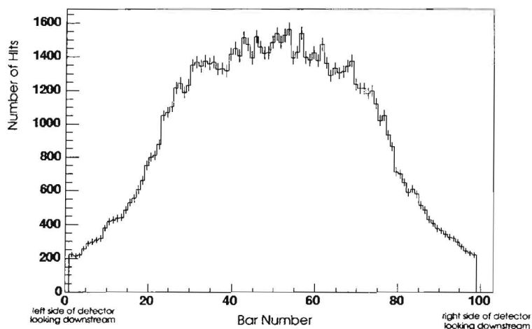
Figure 5.11: Number of hits in scintillator strips in the Muon Rangestack from CCQE muons that originate in the Vertex Detector fiducial volume. The “Bar Number” measures the hit coordinate transverse to the beam direction.
