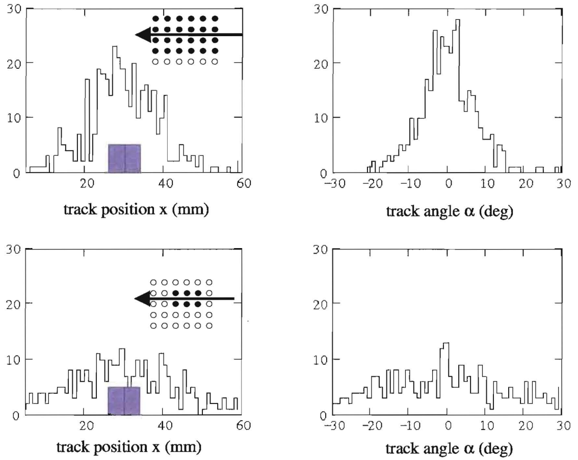
Figure 4.8: Reconstructed position and angle of tracks for two rows of fibers on either side of the beam (top plots) and for only three fibers on either side of the beam (bottom plots). The rectangular box in the left panels indicates the nominal beam position and width.
