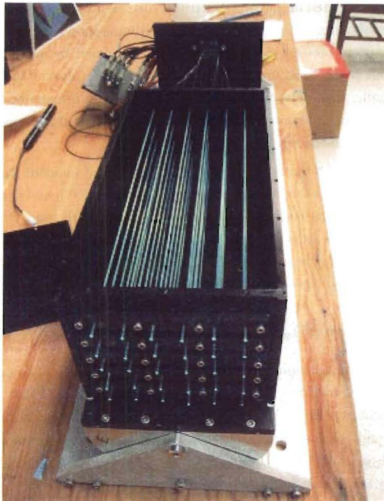
Figure 4.4: Photograph of the prototype detector with the mounted WLS fibers. The protruding fiber ends were covered with a light shield. The photomultipliers were mounted on the plate at the far end. The box could be pivoted to study beams that intercept the fiber matrix at an angle.
