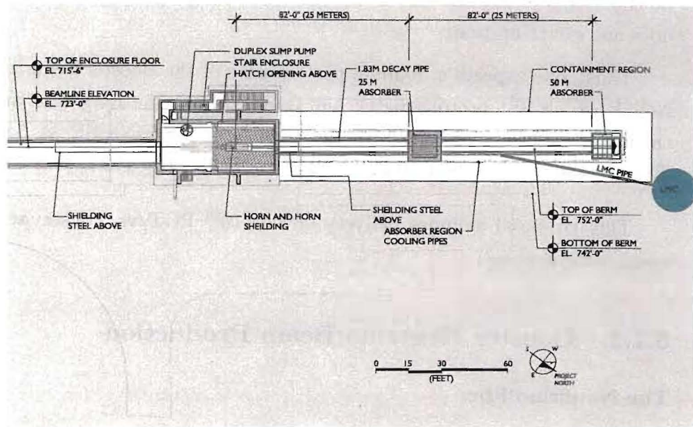
Figure 3.1: Schematic of the MiniBooNE target hall and decay region. The 25 m and 50 m absorber locations are indicated.
