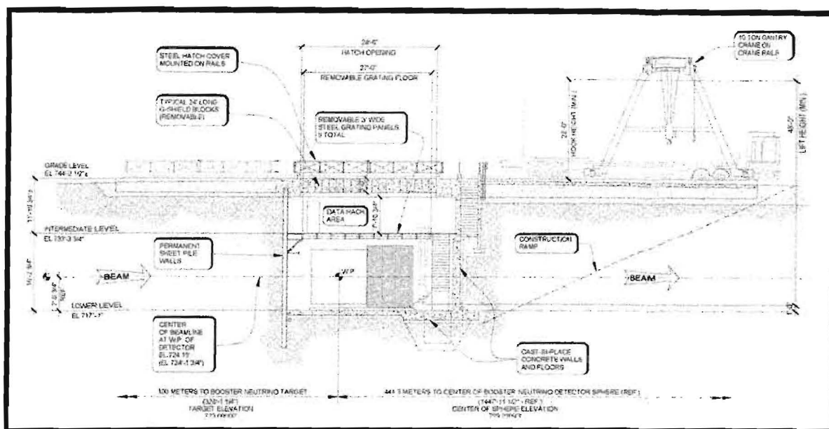
Figure 4.14: Side view of the 25 ft below grade detector enclosure to house the FI-NeSSE detector.
