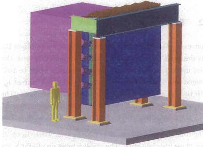
Figure 4.10: An isometric rendering of the Muon Rangestack in front of a box bounding the envelope of the Vertex Detector.
