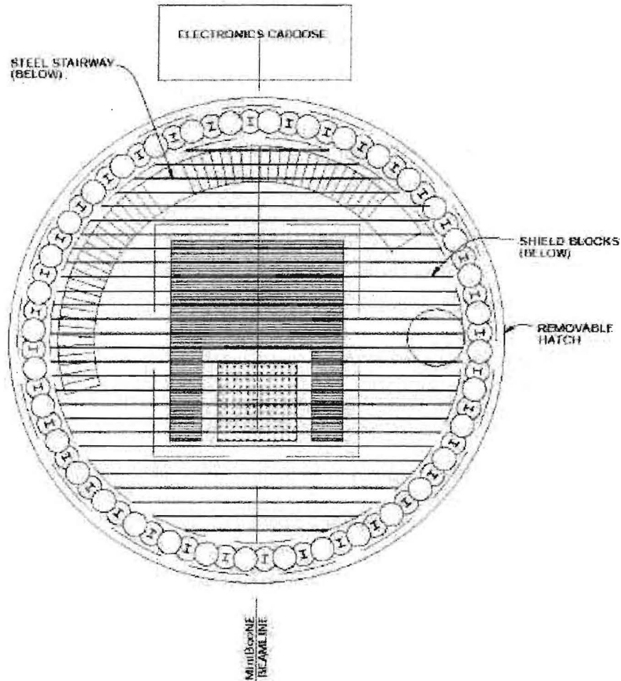
Enclosure Plan
