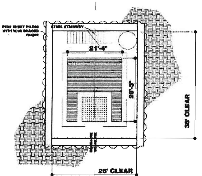
Enclosure Plan
