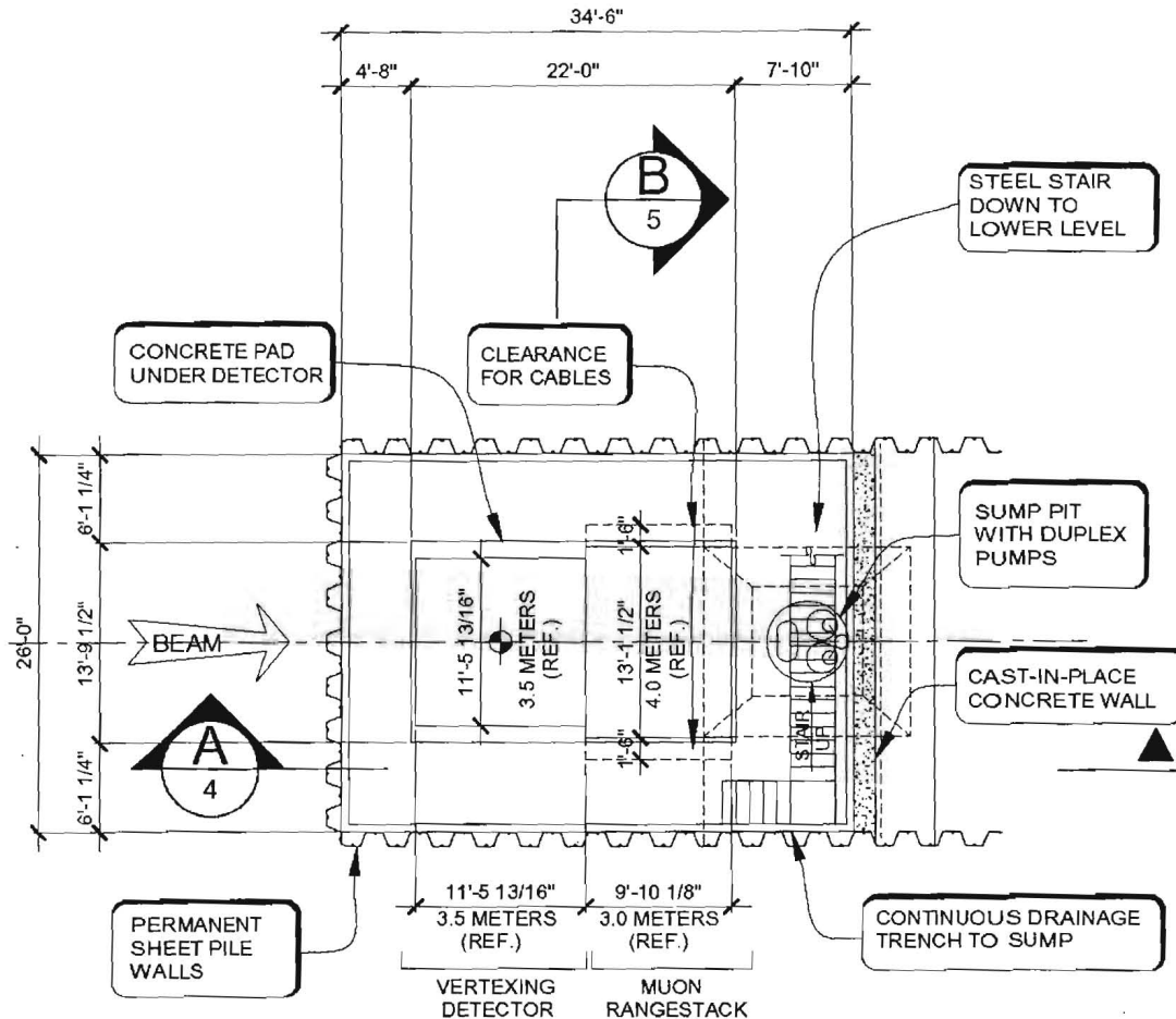
Figure 4.15: Top view of the detector enclosure.
