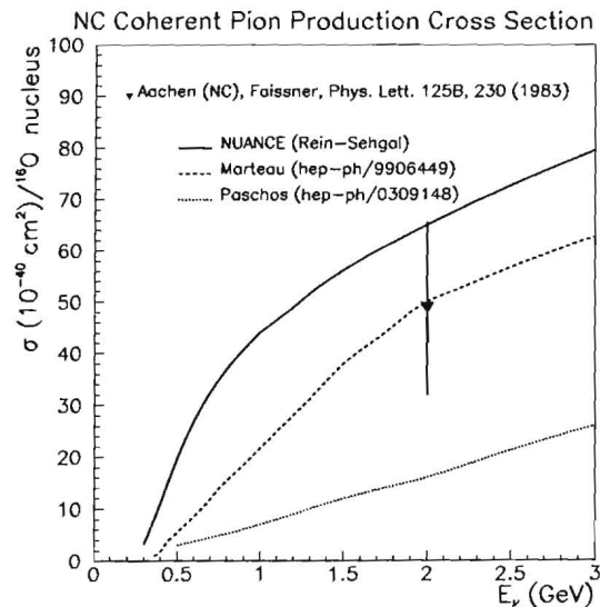
Figure 6.4: Experimental measurement of the NC coherent \pi^0 production cross section at low energy compared to current model predictions [86],[87].
