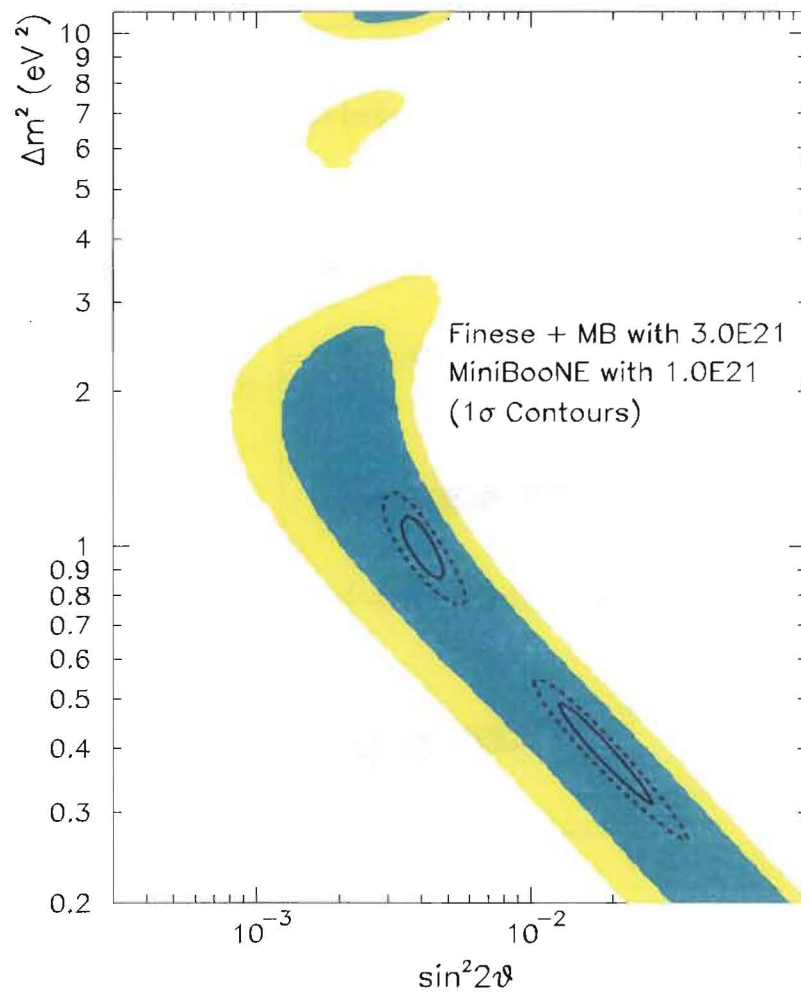
Figure 6.14: The solid ellipse shows the 1\sigma measurement capability for two sets of oscillation parameters for FINEsSE+MiniBooNE for 3 \times 10^{21} POT. The dashed ellipse shows the MiniBooNE Phase I capability. The colored segments indicate the LSND-allowed regions.
