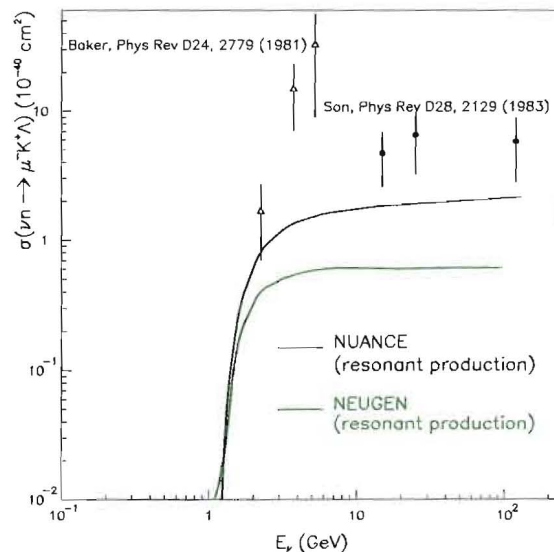
Figure 6.9: Experimental measurements of the \nu_\mu n \rightarrow \mu^- K^+ \Lambda cross section. Also shown are the predictions from two publicly available Monte Carlo generators [82].
