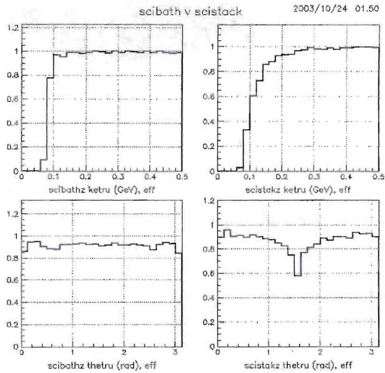
Figure A.3: Reconstructible events versus true angle and energy in Scistack versus Scibath. Upper left corresponds to true kinetic energy of Scibath event; upper right to true kinetic energy of Scistack protons. Bottom left and right are true angle for Scibath and Scistack respectively.
