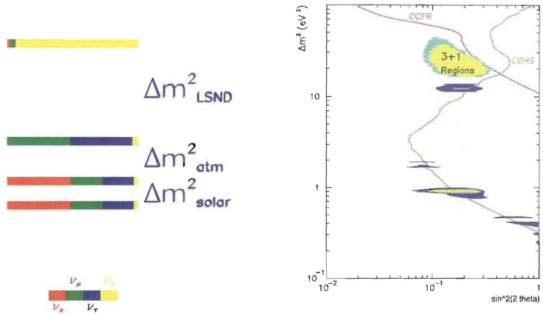
Figure 2.6: Left: an example of a 3+1 mass spectrum. Right: allowed region for \nu_\mu \rightarrow \nu_s in 3+1 models. The exclusion regions for CDHS and CCFR are also shown.
