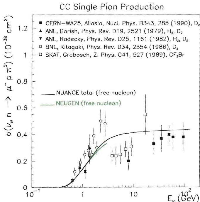
Figure 6.2: Measurements of the CC resonant single \pi^0 cross section, \sigma(\nu_\mu n \rightarrow \mu^- p \pi^0) . Also shown are the Rein and Sehgal-based predictions from two publicly available Monte Carlo generators [82].
