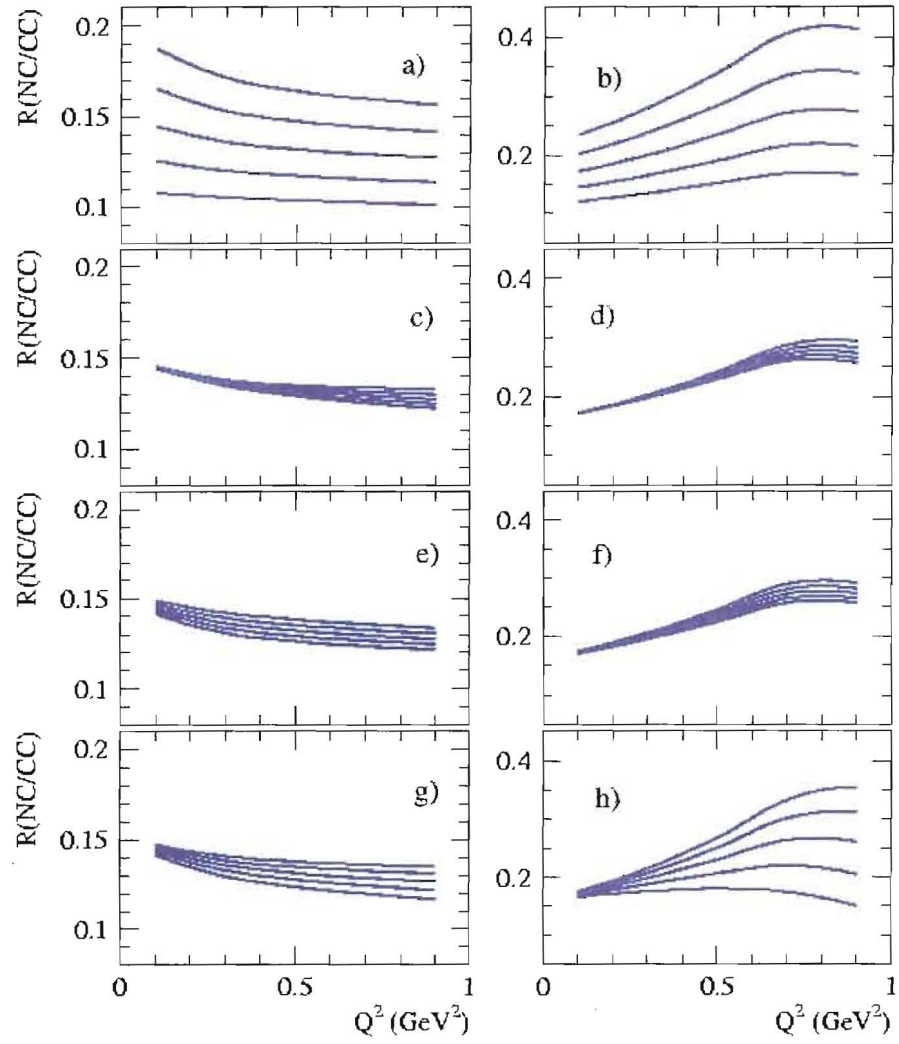
Figure 6.13: The ratio of NC to CC scattering for neutrinos (left column of plots) and antineutrinos (right column) as a function of Q^2 . In each of the 4 rows one of the form factors is varied. In a-b) -0.2 < \Delta s < +0.2 , c-d) -0.2 < F_1^s < +0.2 , e-f) 0.95 < M_A < 1.15 \text{ GeV}/c^2 .
