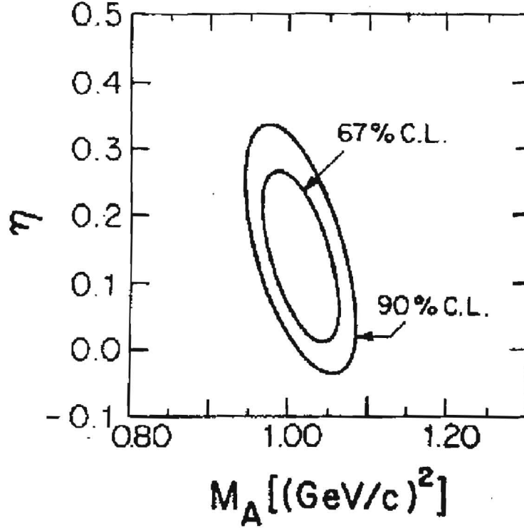
Figure 2.2: Results from a fit of the BNL E734 \nu p \rightarrow \nu p and \bar{\nu} p \rightarrow \bar{\nu} p scattering data [20] indicating the preferred values of \eta ( = -\Delta s ) and M_A . In this fit, M_A was constrained to the world-average value at the time M_A = 1.032 \pm 0.036 GeV.
