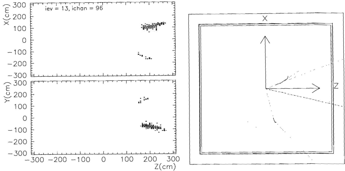
Figure 6.8: A NC coherent \pi^0 interaction in the FINeSSE detector, \nu_\mu {}^{12}\text{C} \rightarrow \nu_\mu {}^{12}\text{C} \pi^0 . The figure on the right shows the true GEANT particle trajectories in the XZ plane for the same event. As can be seen, the hit clusters correspond to the two photons from the \pi^0 decay.
