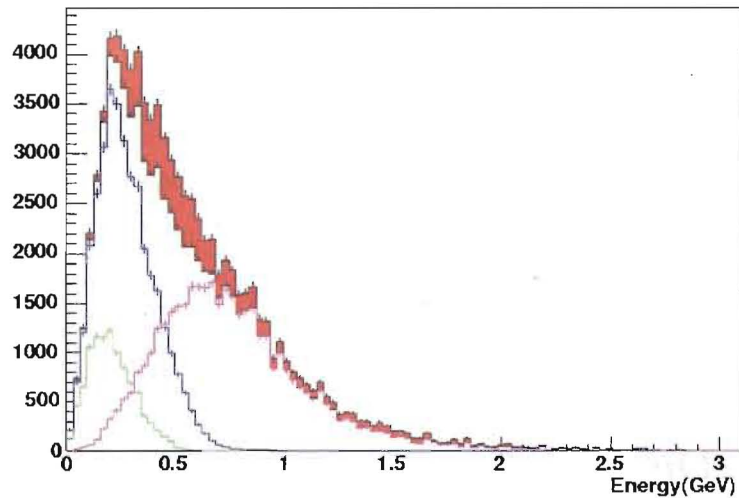
Figure 5.16: True kinetic energy distribution for all muons from CCQE interactions in the Vertex Detector fiducial volume shown in red. Overlaid in white is the sample of those with a contained muon. Also shown are contributions corresponding to muons stopping in the Vertex Detector (green), the Vertex Detector veto (blue), and the Muon Rangestack (purple).
