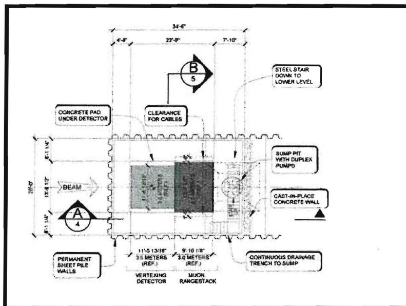
Figure 3 - Enclosure Plan
