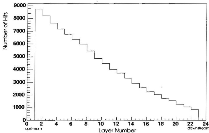
Figure 5.12: Number of hits in each scintillator layer in the Muon Rangestack from CCQE muons that originate in the Vertex Detector fiducial volume. The “Layer Number” measures the coordinate along the beam direction.
