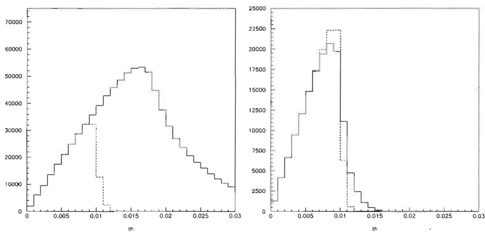
Figure 5.18: Left, solid: Angular acceptance of the FINeSSE detector with the 50 m absorber in radians; Right, solid: Acceptance with the 25 m absorber in radians. Dashed (both plots): acceptance of the MiniBooNE detector in radians.
