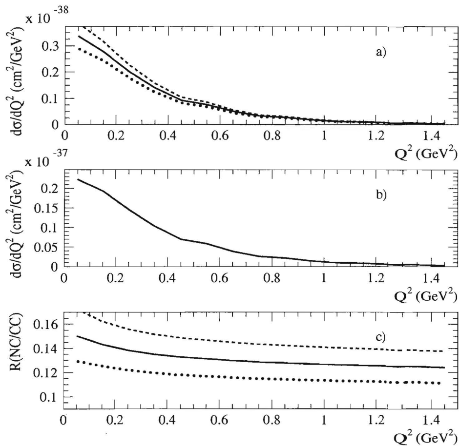
Figure 2.3: Flux-weighted differential cross section as a function of Q^2 for \nu p \rightarrow \nu p (a) and \nu n \rightarrow \mu^- p (b) scattering together with the cross section ratio of these two processes (c). These quantities are shown for G_A^s = 0 (solid), -0.1 (dashed), and +0.1 (dotted). The \nu n \rightarrow \mu^- p process does not depend upon G_A^s .
