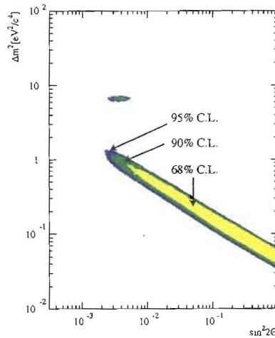
Figure 2.5: LSND and Karmen joint analysis allowed region.
