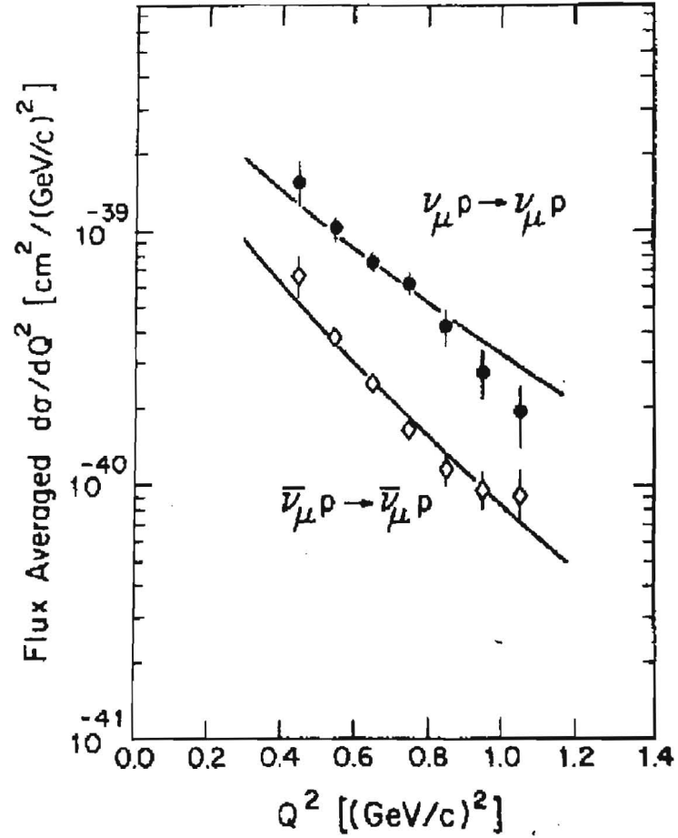
Figure 2.1: BNL E734 results on \nu p \rightarrow \nu p and \bar{\nu} p \rightarrow \bar{\nu} p [20]. The solid lines are fits to the data.
