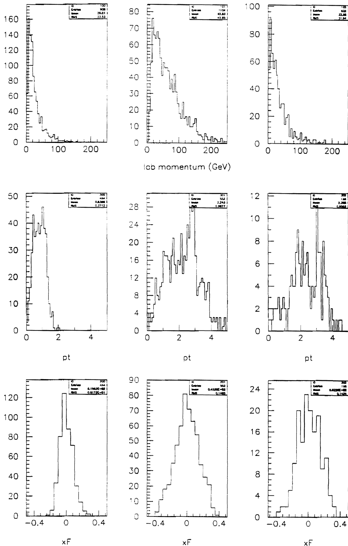
Figure I.1 - The single-particle momentum spectra, x_F , and p_t distributions of accepted charm and beauty decays: left D^0 \rightarrow K^-\pi^+ , middle B^0 \rightarrow \pi^+\pi^- , right B^0 \rightarrow J/\psi K_s .
