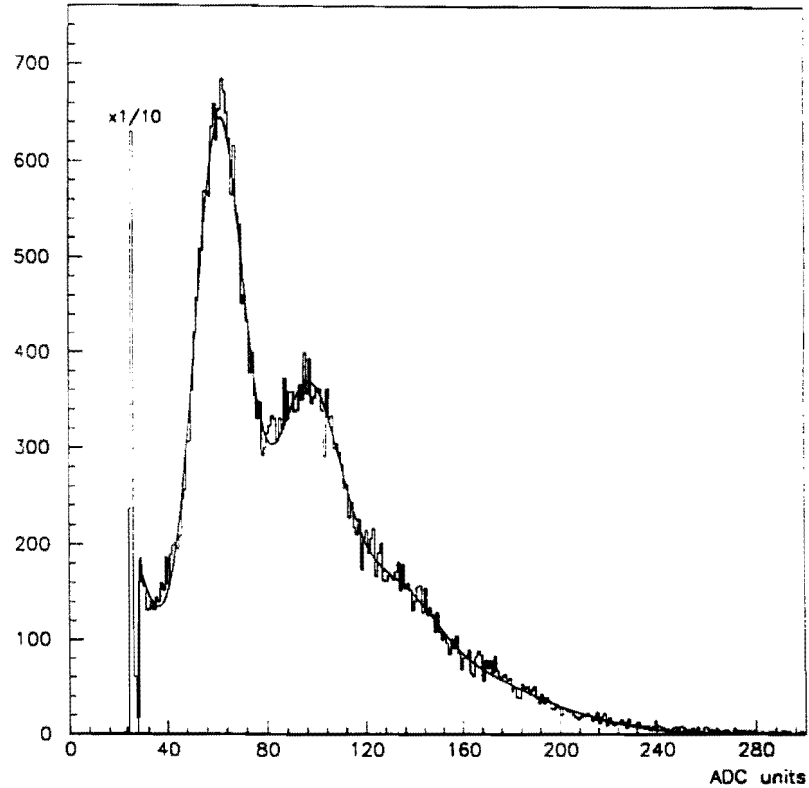
Figure 6: The Pulse-height distribution from the UV lamp. The peak at zero photoelectrons is divided by 10.
