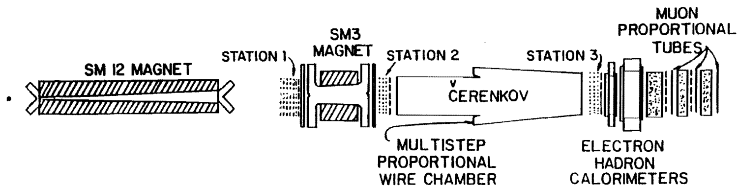
PLAN VIEW E-605
