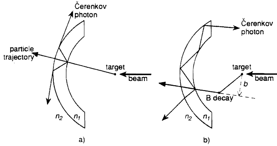
Figure 1: The principle of the optical discriminator: a particle with zero impact parameter (a) produces Cherenkov light refracted through the outer surface of the crystal, whereas for a particle with a non-zero impact parameter (b), part of the Cherenkov light is internally reflected and trapped.
