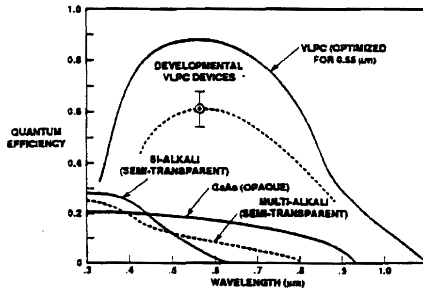
Quantum efficiencies for VLPCs compared to several common photocathodes. Improvements over current developmental VLPCs are expected to yield peak QEs near 0.9 for wavelengths near 0.55 micron.
