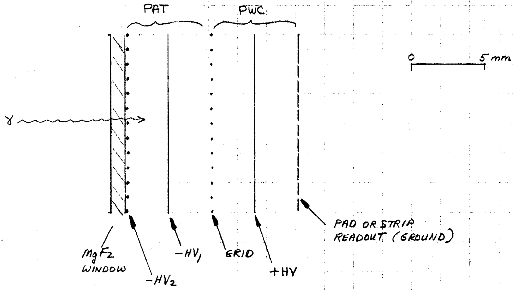
SCHEMATIC OF AVALANCHE DETECTOR GAS FILL ARGON + BENZENE
