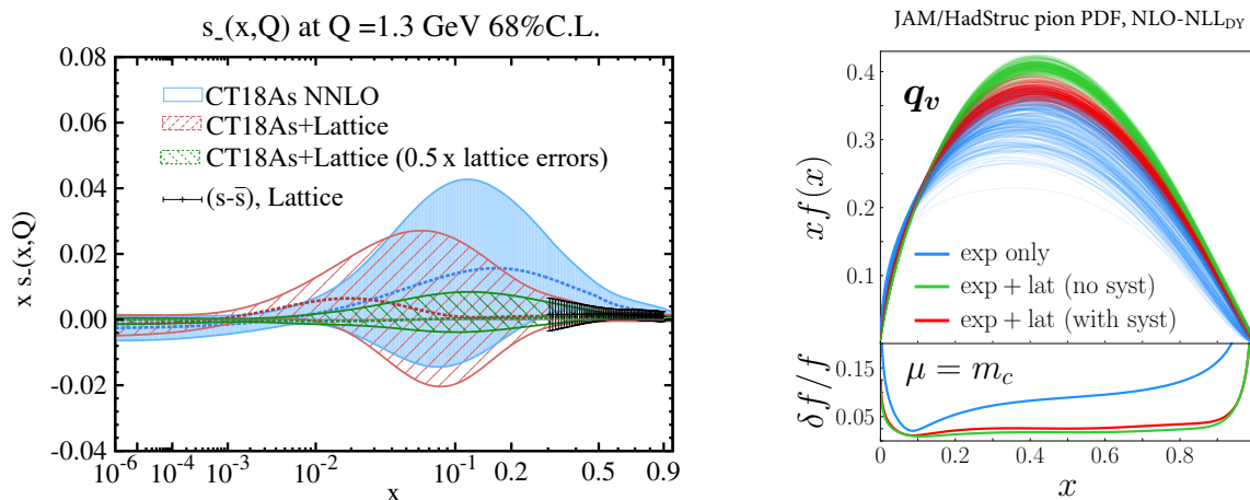
Figure 1-26. Left: Impact of constraints from lattice QCD (black dashed area) on the difference between strange quark and antiquark PDFs in a CT18As N 2 LO fit [237]. The red (green) error bands correspond to the current (reduced by 50%) lattice QCD errors. Right: determination of a quark PDF in a pion using a combination of experimental and lattice QCD data, and including threshold resummation [238].
