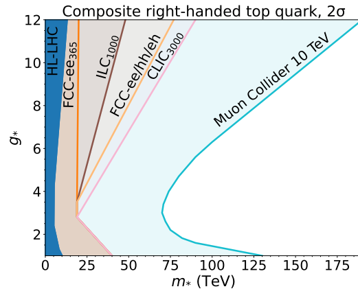
Figure 1-19. Exclusion ( 2\sigma ) sensitivity projections for compositeness models at future colliders as labeled, for models where both the Higgs boson and the top quark with right-handed couplings are composite. Plot based on Refs. [81, 82].
