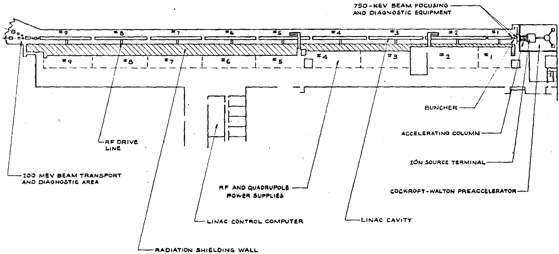
Fig. 2. Simplified plan view of linac.
