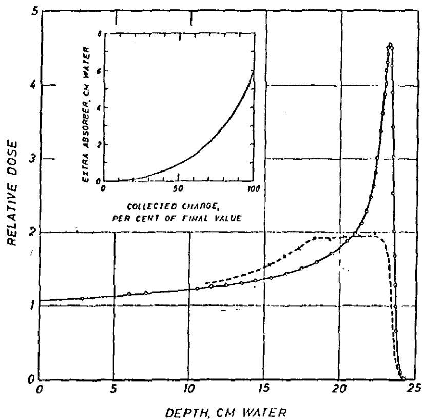
Fig. 1. Example of transformation of the Bragg peak. Variation of the thickness of the absorber was performed according to the curve in the inset diagram. The large diagram shows the original (—) and the calculated transformed (-----) depth-dose curves. The crosses give the results of measurement of points on a depth-dose curve obtained by use of a ridge filter of the type described in the text. The profile of the ridges was determined by the shape of the curve in the inset diagram, one cm water being equivalent to 0.18 cm brass.
