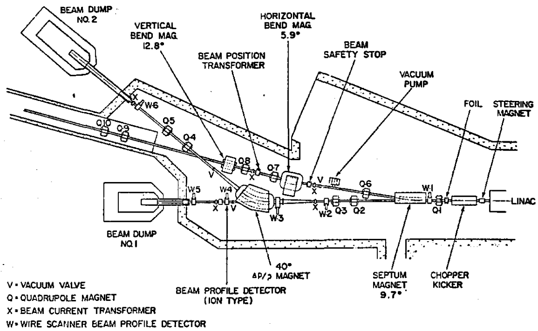
Fig. 6. Layout of the system for measuring the emittance and the momentum spread of the beam from the 200-MeV linac.
