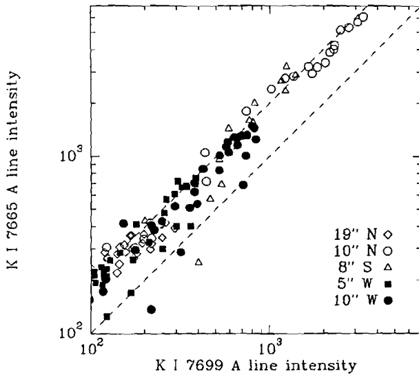
Fig. 6. Intensity of the two K I lines. The upper dashed line indicates a ratio of 2, corresponding to the optically thin case. Only the data with a good signal-to-noise ratio are plotted.
