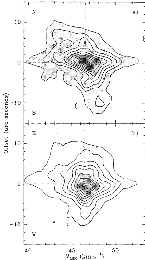
Fig. 4. Velocity-position diagrams in the ^{12}\text{CO}(2-1) line obtained from cuts at declination offset = 0 (bottom panel) and R.A. offset = 0 (top panel).
