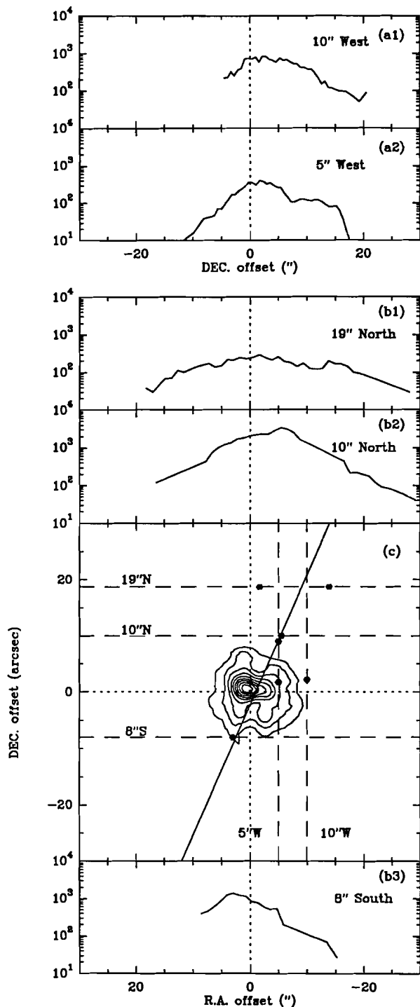
Fig. 5. Intensity distribution of the 7699 Å KI line along 5 slits. Panels (a1) and (a2): the two western slits observed at CFHT. Panels (b1), (b2) and (b3): northern and southern slits observed at OHP. Panel (c): location of the slits (dashed lines) superimposed on the CO(2-1) map; the black dots on each slit indicate the positions of the maxima of KI emission. The full line emphasizes the apparent alignment of some maxima with the center (see text for details).
