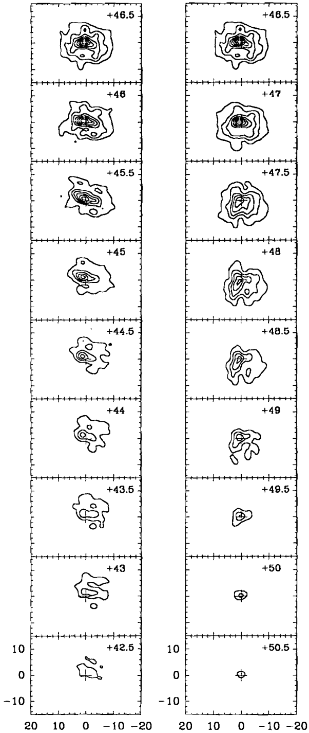
Fig. 3. Contour map of the ^{12}\text{CO}(2-1) emission integrated over equally spaced velocity channels with width of 0.5 \text{ km s}^{-1} . The left column corresponds to the blue-shifted emission and the right column to the red-shifted emission. In each column the top panel displays the emission at the adopted stellar velocity ( 46.5 \text{ km s}^{-1} ). The lower level contour and the contour spacing are 1 \text{ Jy beam}^{-1} \text{ km s}^{-1} . The central LSR velocity for each panel is indicated in the top right corner.
