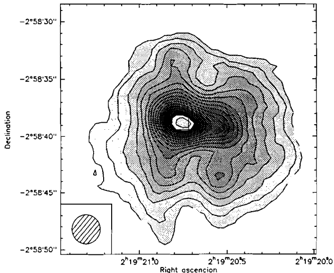
Fig. 1. Contour map of the integrated ^{12}\text{CO}(2-1) emission from o Ceti over the whole velocity range of emission. The lower level contour and the contour spacing are 2 \text{ Jy beam}^{-1} \text{ km s}^{-1} . The beam after cleaning is shown in the box in the lower left corner.
