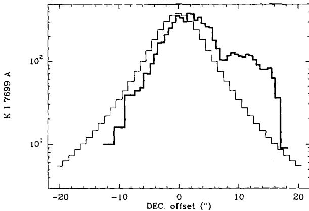
Fig. 7. Comparison between an optically thin model of K I emission in a spherical envelope (thin line) and the observations from the 5'' W slit (thick line).
