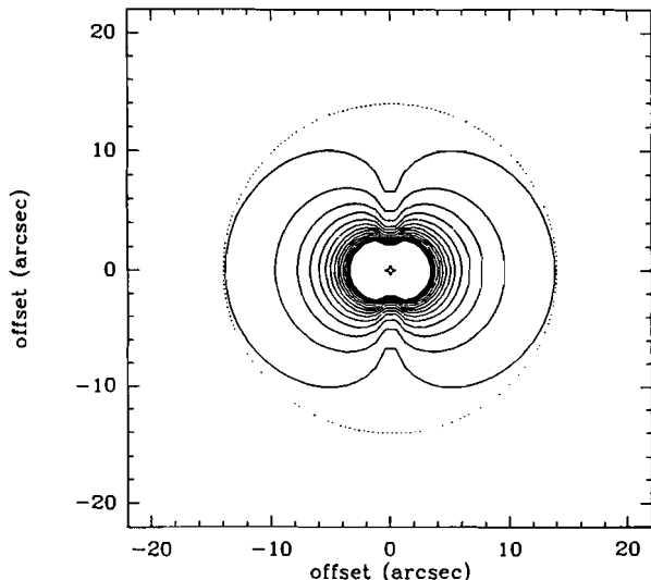
Fig. 2. Intensity map for a density distribution n(r) \propto \cos^{1/2}(\theta) r^{-2} , assuming optically thin emission and constant excitation conditions. A dashed circle has been drawn to emphasize the resulting departure from sphericity.
