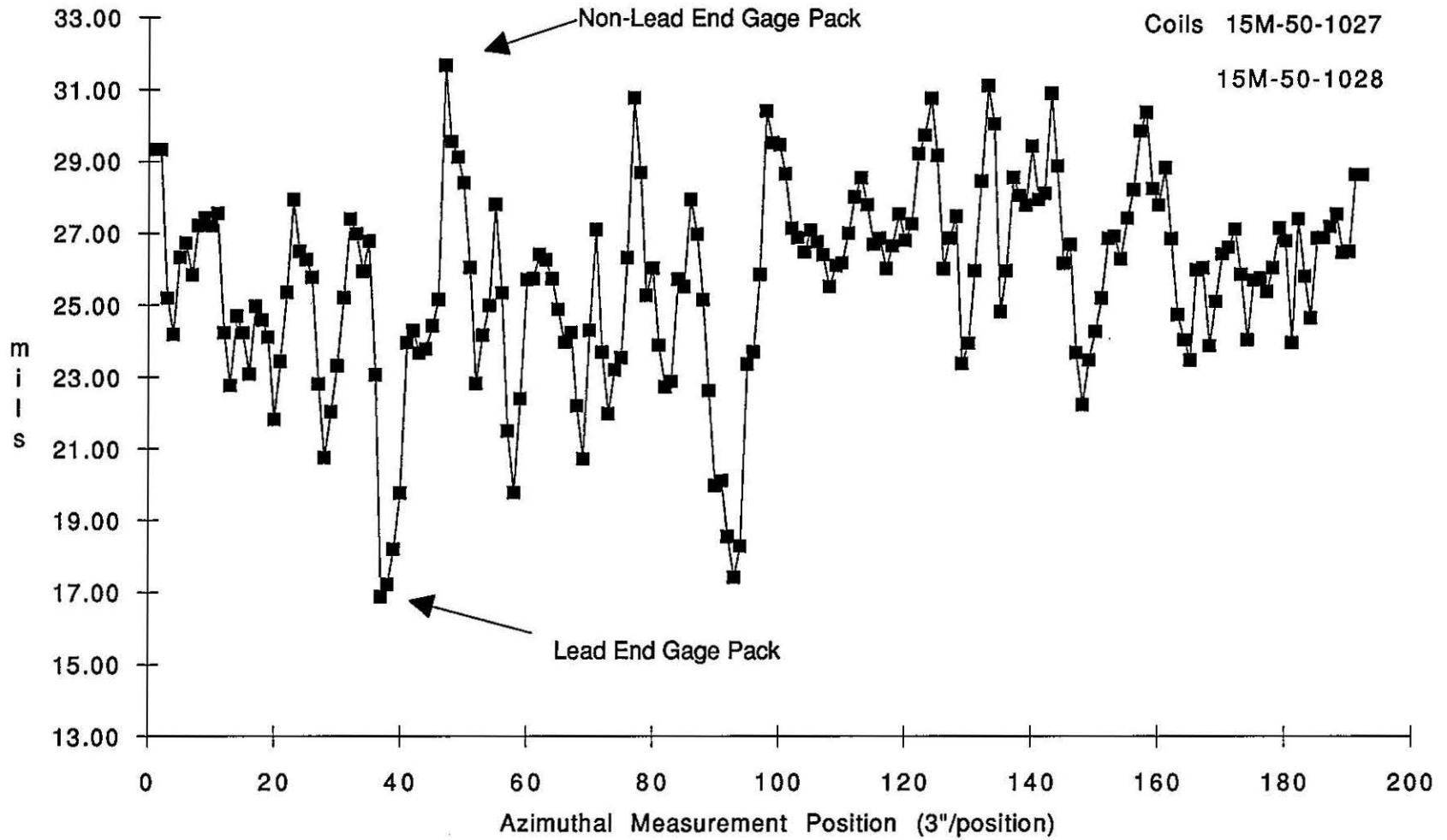
Summed Azimuthal Measurements vs. Longitudinal Position for DCA323
