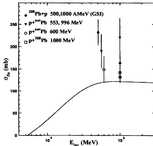
Figure 15. Total fission cross-section as a function of incident energies: Symbols are experimental data given in table 3 and the full line corresponds to the Prokofiev's systematic for the ^{208}Pb .
