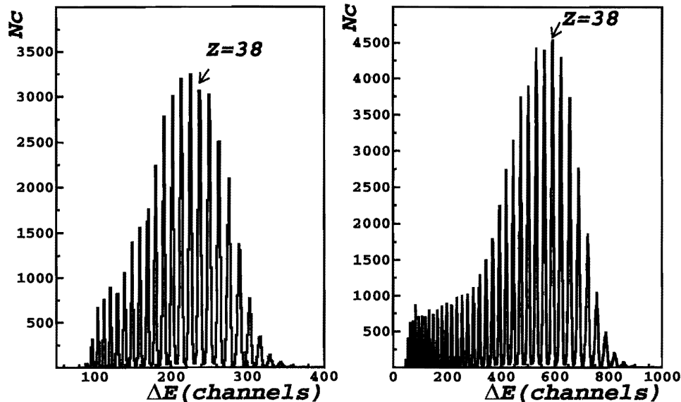
Figure 3. Left: The energy-loss spectrum for a setting centered on ^{61}\text{Ni} before the change of the electronics. Right: The same spectrum after the change of the electronics (see text).
