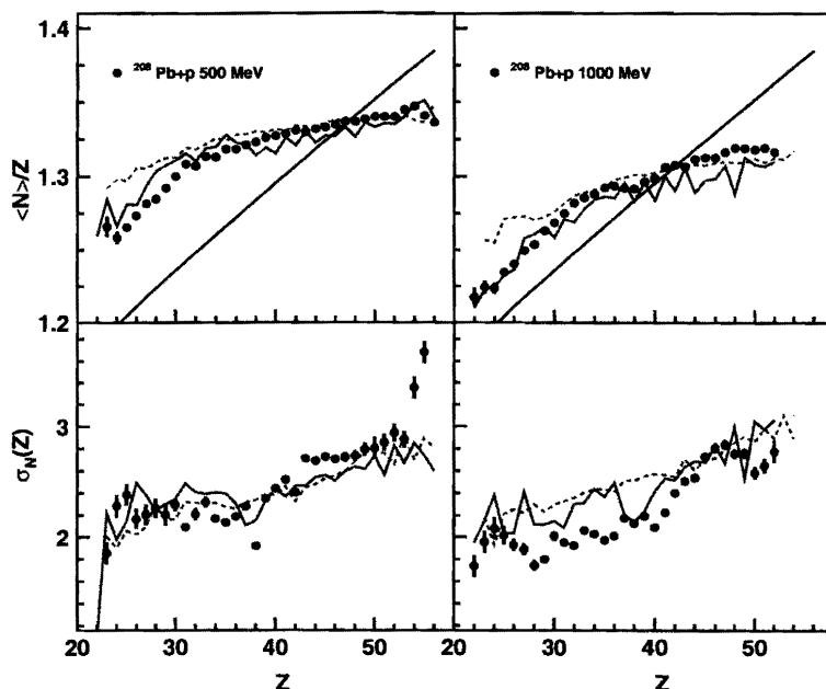
Figure 22. Points are data at 500 MeV (left) and 1000 MeV (right). Dashed curves are results of INCL4/ABLA and full curves of INCL4/GEM calculations. Upper panels: Ratio between the mean neutron number and the charge as a function of the nuclear charge. The full line corresponds to the stable isotopes [53]. Lower panels: Standard deviations of the isotopic distribution as a function of the nuclear charge.
