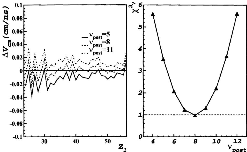
Figure 20. Left: differences \Delta V_{cm} between the experimental average velocities in the center-of-mass system (see table 11) and calculations assuming different numbers of post-fission neutrons, as a function of the nuclear charge. The different lines correspond to the different velocity values calculated with \bar{v}_{post} = 5 (full line), \bar{v}_{post} = 8 (dashed line), \bar{v}_{post} = 11 (dashed-dotted line). Right: Variation of the \chi^2 by degree of freedom as a function of the number of evaporated neutrons.
