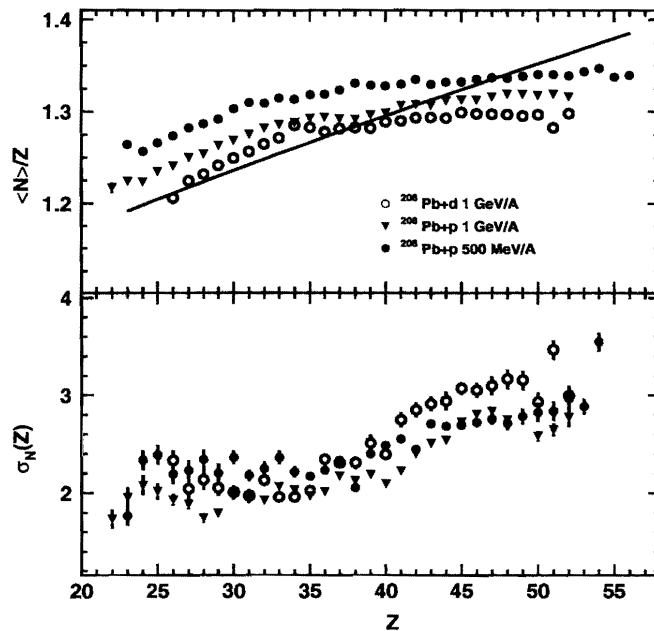
Figure 16. Upper panel: Ratio between the mean neutron number and the charge as a function of the atomic number. The black line corresponds to the stable isotopes [53]. Bottom panel: standard deviation of the isotopic distribution as a function of the atomic number. The error bars are given by the uncertainty of the fit.
