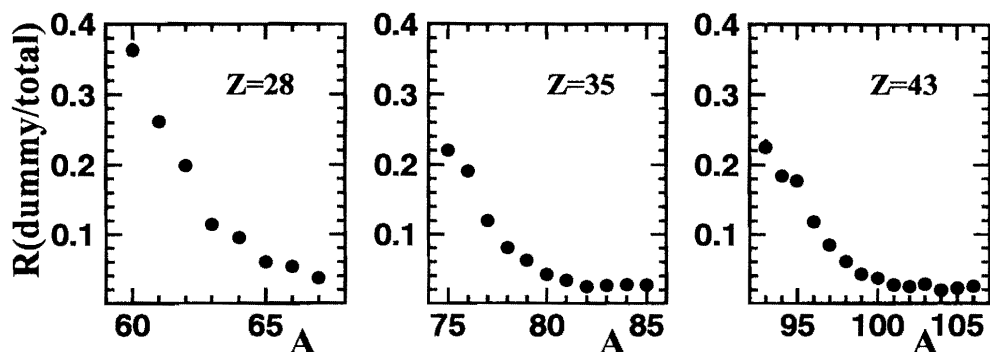
Figure 9. Ratio between the contribution due to the dummy target and the one of the total target as a function of the mass, for three elements of Z=28, 35, 43 .
