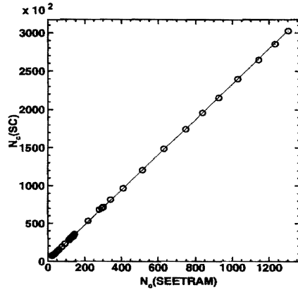
Figure 7. Linear fit between the number of the particles detected by the scintillator and the number of counts measured with the SEETRAM. Errors are smaller than the symbol size.
