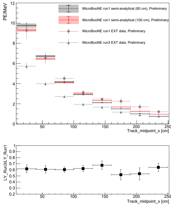
Figure 11: Top: total light yield with regard to different drift distances with the hexagonal cut. Data is compared with simulations from semi-analytical model with the different Rayleigh scattering lengths. Bottom: the ratio of total light yield in run 3 data to these in run 1 data with the hexagonal cut.
