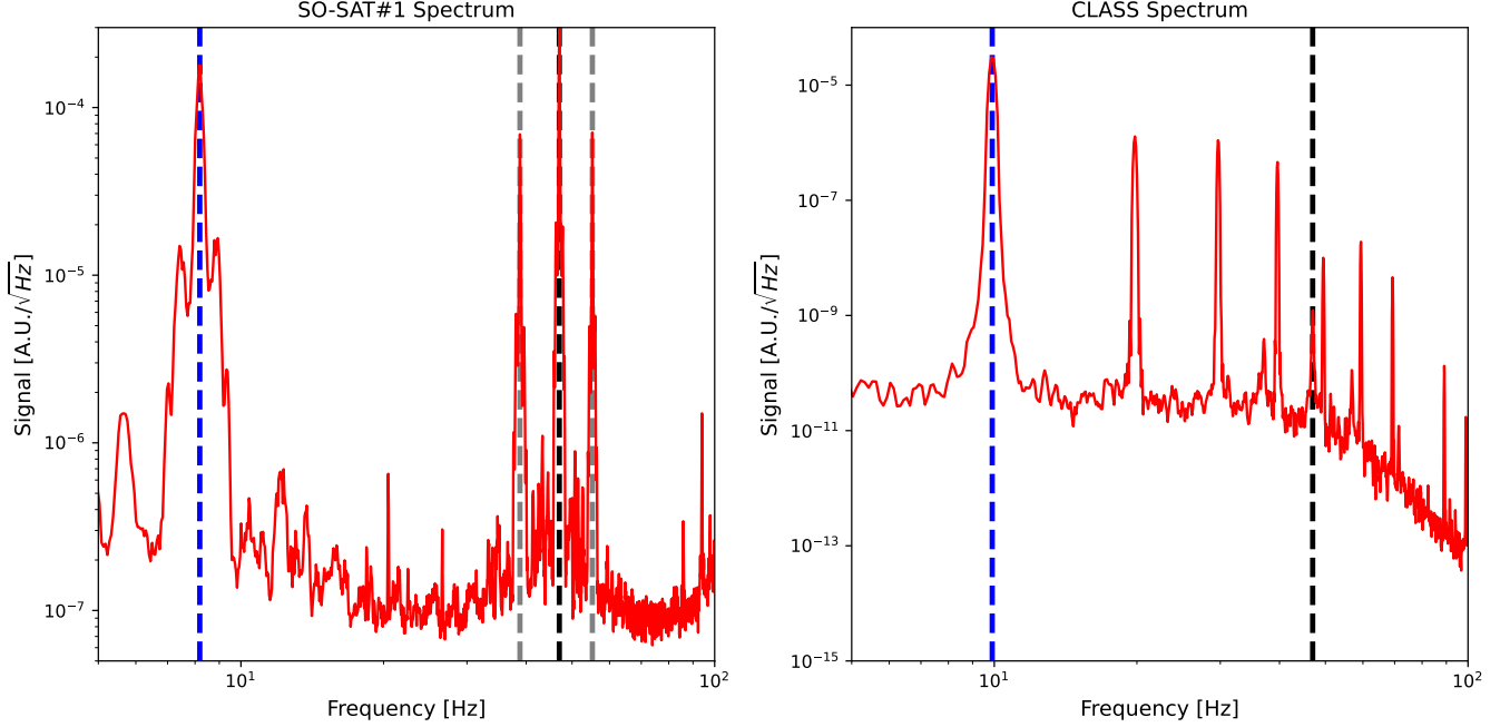
Figure 8. Signal seen by a single detector throughout an entire flight for both Simons Observatory and CLASS. For the SO power spectrum, we highlight both the 8 Hz modulation frequency of the HWP in blue and the 47-8 Hz and 47+8 Hz in gray. Instead, for CLASS the VPM signal is in blue. For both power spectra, we also highlight in black the 47 Hz signal coming from the source.
