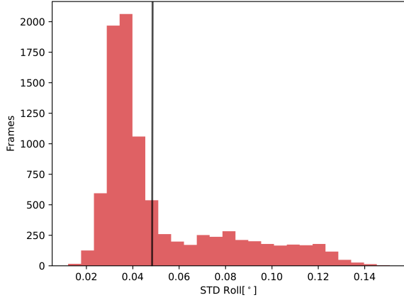
Figure 9. Histogram presenting the uncertainty of on the roll angle of the camera estimated using the Jackknife re-sampling for each frame. The black vertical line represents the average value of the uncertainty.
