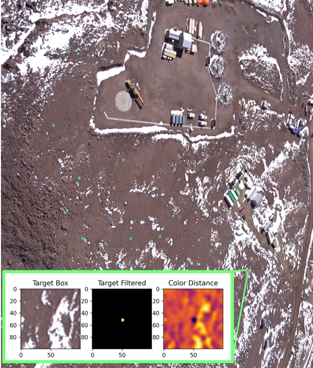
Figure 10. View of the site as seen by the Photogrammetry camera. The recognized targets are enclosed in light green square and a zoom of one of them is presented. Here, we show the process to recognize the target from the image.
