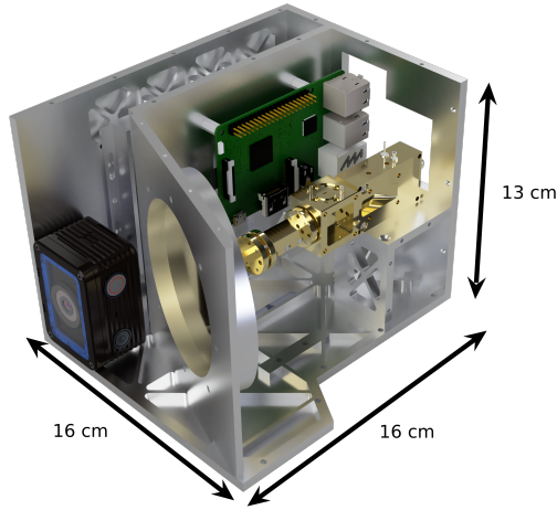
Figure 3. Render of the payload with all the components.
