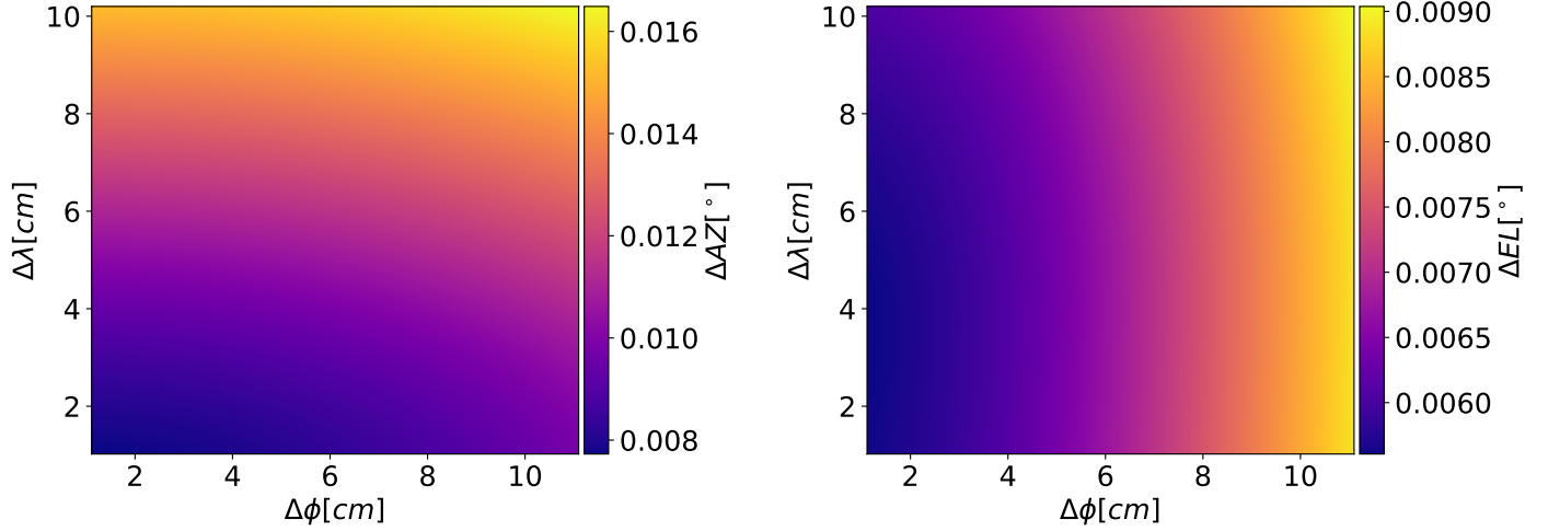
Figure 2. Error in azimuth and elevation coordinates of the drone at a distance of 500 m and 45^\circ elevation. The error in vertical position is considered to be constant at 10 cm.
