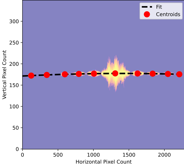
Figure 6. Fitted parabola on the diffraction pattern. The centroids of each diffraction maxima are plotted as red dots.
