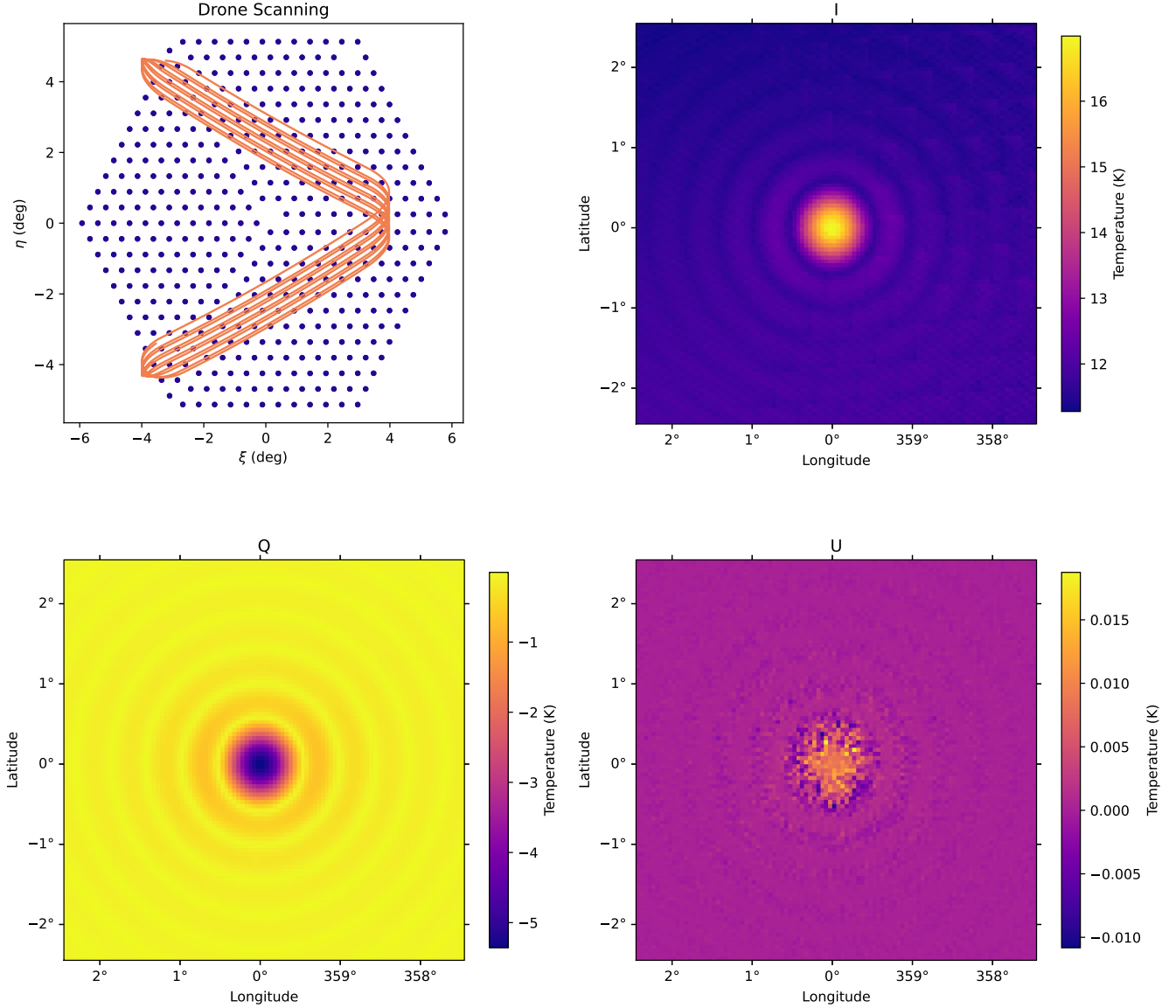
Figure 7. Scanning pattern of the drone over a single array and the resulting maps from this simulated flight. The pattern replicates the programmed flight plan that we have during a typical calibration campaign.
