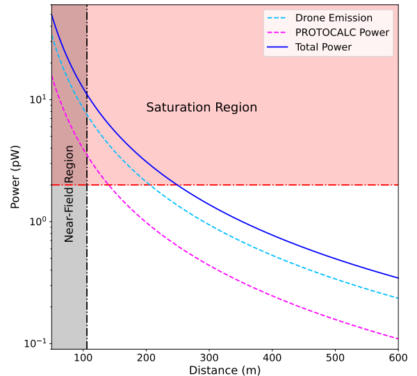
Figure 1. Emission of the drone modeled as a blackbody in the 90 GHz band with a bandwidth of 30%, for a small aperture-type (like SO-SAT or CLASS) telescope with 50 cm aperture. We included also the power emitted by the PROTOCALC source considering a diffraction-limited single mode telescope. The vertical dotted line represents the far-field distance, while the horizontal represents the 2 pW power which is a conservative saturation power for TES detectors.
