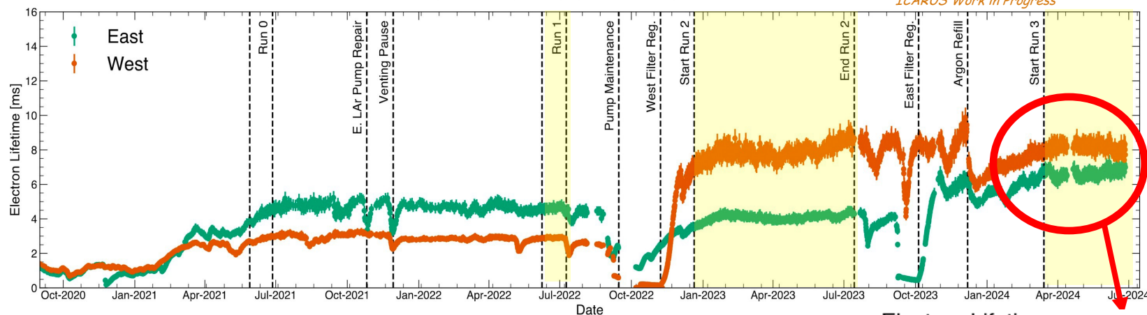
ICARUS Electron Lifetime
