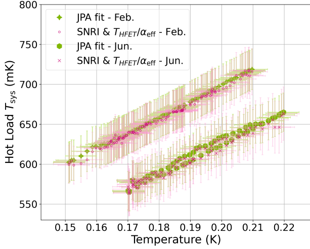
FIG. 8. Hot Load T_{\text{sys}} comparison at 1280 MHz. Here we show the comparison between the two methods, using SNRI (pink points) and using JPA fit (green points), over the course of both hot load measurements done at 1280 MHz. It is clear that for both the February and June data the system noise temperature we calculate is consistent between the two methods within error bars.
