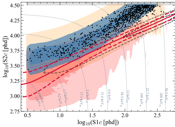
FIG. 2. The final high energy WIMP-search data after all cuts in \{\log_{10}(S1c), \log_{10}(S2c)\} space. The contours that enclose 1\sigma (dark) and 2.5\sigma (light) regions represent the following models: the shaded red region indicates neutrons originating from detector materials, the shaded orange region indicates Compton scatters from detector components, the blue region is the combined representation of all other ER models ( ^{214}\text{Pb} , ^{212}\text{Pb} , ^{85}\text{Kr} , ^{37}\text{Ar} , ^{125}\text{I} , ^{124}\text{Xe} , ^{127}\text{Xe} , ^{136}\text{Xe} , and \nu ER) and the black dashed lines show a 1000 \text{ GeV}/c^2 \mathcal{L}_6 isoscalar signal model. The solid red line corresponds to the NR median, while the red dotted lines represent the 10% – 90% percentiles. The model contours are produced with a linear scale for S1c prior to being plotted on a log-scale and take into account all the efficiencies used in the analysis. Contours of constant recoil energy have been included as thin gray lines. Grayed regions at the left and top of the plot indicate parameter space outside the energy ROI.
