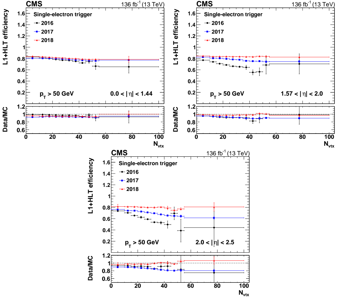
Figure 10: The L1+HLT efficiency of the single-electron HLT path with p_T > 27 (32) GeV in 2016 (2017 and 2018) with respect to an offline-reconstructed electron as a function of N_{\text{vtx}} obtained for 0 < |\eta| < 1.44 (upper left), 1.57 < |\eta| < 2.0 (upper right), and 2.0 < |\eta| < 2.5 (lower). The electron p_T is required to be above 50 GeV. The lower panel of each plot shows the ratio of data to MC simulation. The vertical bars on the markers represent combined statistical and systematic uncertainties.
