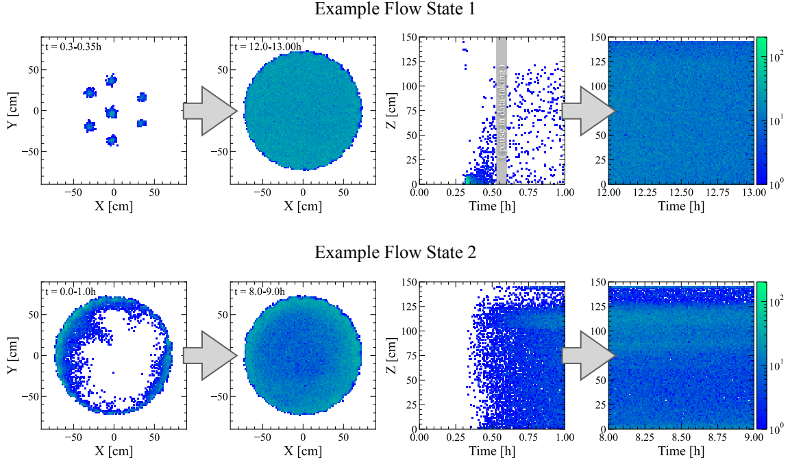
Figure 6: Examples of studying LXe flow in the TPC using injected ^{83\text{m}}\text{Kr} . Example Flow State 1 shows the first ^{83\text{m}}\text{Kr} injection taken in LZ, which required tuning of the data acquisition (DAQ) settings to optimize data rates. The grey band represents a gap in data taking to change the DAQ settings. The second flow state “Flow state 2” is purposefully optimized to increase the calibration source convective mixing efficiency.
