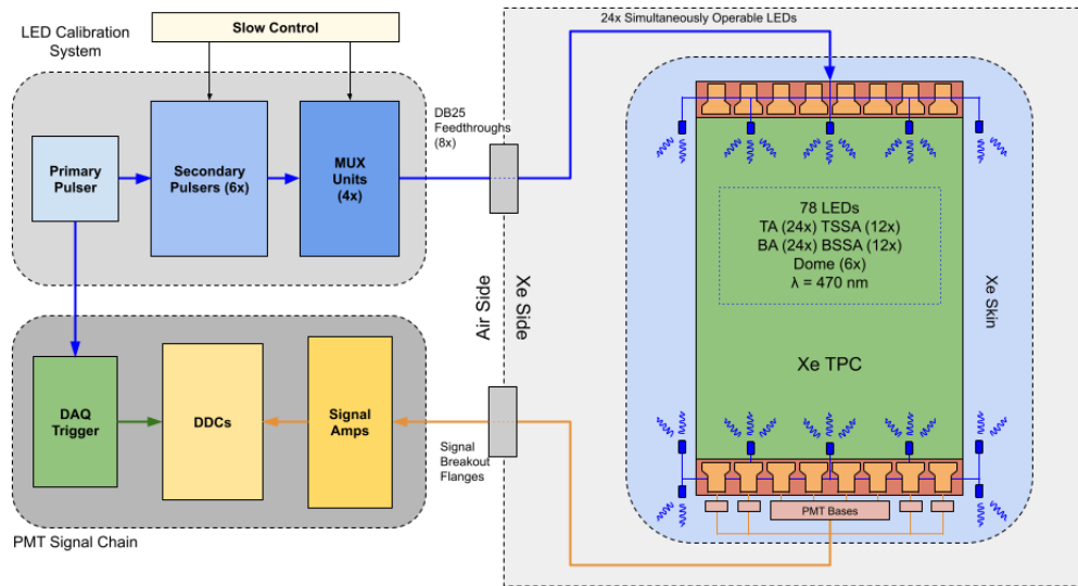
Figure 23: A diagram showing the full Xe LED Calibration System. Signal from a primary pulser can simultaneously drive up to 24 of the 78 LEDs installed throughout the TPC and Xe skin. The primary pulser also acts as an event trigger for the digital data collectors (DDCs) via the LZ data acquisition (DAQ) system. Note that the LEDs do not protrude into the TPC, and that skin and dome PMTs are excluded from this diagram.
