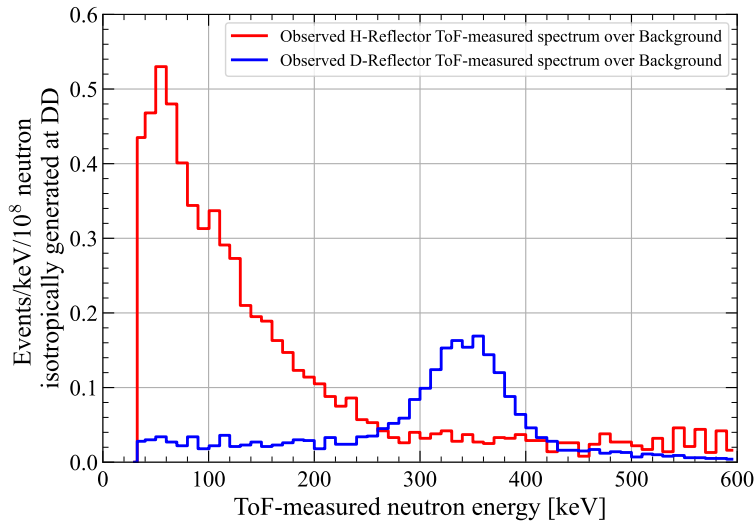
Figure 18: Measured time of flight (ToF) neutron energy of the D- (blue) and H- (red) Reflector modes in a test setup before their use in LZ. The energy spectrum of each Reflector mode can be tuned by the geometric configuration.
