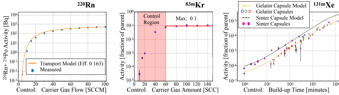
Figure 5: Results of dosing control studies performed on a system test version of the source injection panel. In each panel, the x-axis represents the ‘control parameter’ used during injection to set the injected activity. A ^{220}\text{Rn} injection proceeds by a continuous flow of the Xe carrier gas through the generator, with the carrier gas flow rate setting the ^{220}\text{Rn} fraction which escapes the injection panel and reaches the getter before decaying. The ^{220}\text{Rn} figure shows the equilibrium activity increases exponentially with the carrier gas flow rate, which can be described by a transport model from reference [49]. This allows us to control the total number of ^{220}\text{Rn} events by adjusting the duration of the injection. For ^{131\text{m}}\text{Xe} and ^{83\text{m}}\text{Kr} , the injected activity is measured as a fraction of the parent material’s activity at the time of the injection. In both cases, there is a maximum-possible activity to inject: approximately 10% for ^{83\text{m}}\text{Kr} and 0.1% for ^{131\text{m}}\text{Xe} (a product of the branching fraction and the gas emanation efficiency). The ^{83\text{m}}\text{Kr} injected activity is controlled by pushing only a small fraction of the generator activity out of the generator assembly, with carrier gas flow quantity measured in standard cc. The comparatively long half-life of ^{131\text{m}}\text{Xe} (and the shorter half-life of its parent ^{131}\text{I} ) motivates a dose control strategy based on pumping out the generator contents and then waiting a build-up time specific to the desired ^{131\text{m}}\text{Xe} activity.
