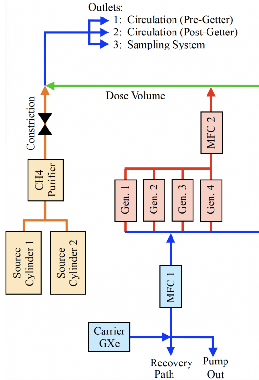
Figure 4: Simplified diagram of the source injection panel, highlighting various regions with corresponding colors. The green region is used for dosing 83m Kr and CH 4 -based sources, and serves as a flow through path for the other gaseous sources. Gas flow through the panel is at the scale of a few to several hundred standard cc per minute, set either by a fixed flow restriction or by variable mass flow controllers (MFCs). Numerous pneumatic valves (not indicated in the schematic) set the source and flow path.
