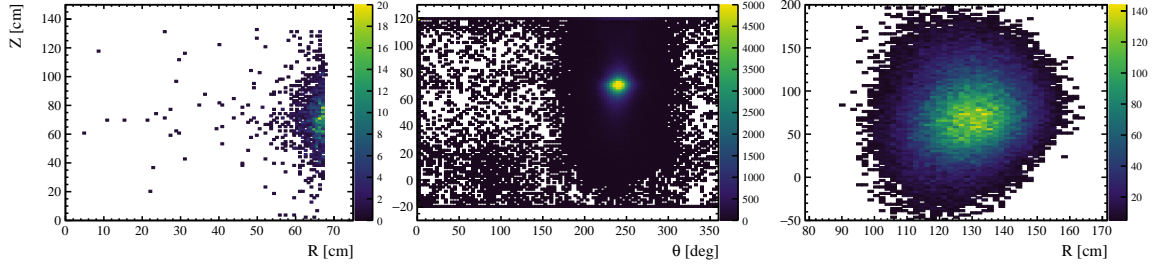
Figure 11: Reconstructed positions of events in the TPC (left), Skin (middle) and OD (right) induced by a ^{228}\text{Th} source deployed to a position of 70 cm above the TPC cathode level in the CSD tube. The x- and y-axes have different scales for the three plots to accommodate the varying dimensions of the three detectors. The x-axis of the middle plot represents the angle ( \theta ), not the radius (R), because the Skin’s width in the radial direction is much narrower compared to that of the TPC and the OD.
