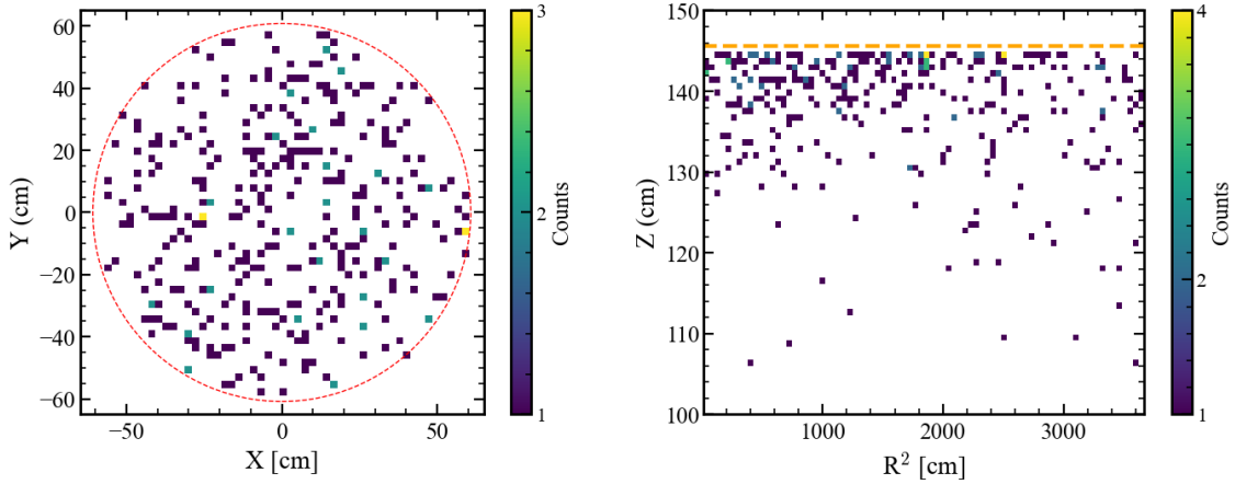
Figure 22: Reconstructed positions of 200 events from the YBe calibration data in the Cartesian coordinates of the TPC. Left: x vs. y distribution. The red contour in the left plot represents the radial selection cut applied to the data. Right: z vs. R^2 distribution. The majority of YBe events appear in the top few cm underneath the liquid-gas interface (marked by the orange line in the right plot) since neutrons from the YBe source located on top of the OCV can only penetrate a few centimeters into the liquid xenon. The gap between the liquid-gas surface and the events is the result of the drift time selection.
