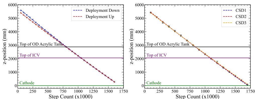
Figure 10: Left: Relationship between the physical measurement of steps from the stepper motor and the laser's z -position reading for a deployment of a non-radioactive dummy source down and up the calibration tube. A discrepancy between the two deployments is observed when the source is first installed, due to the filament adjusting to the new weight. Right: Deployment alignment curves for three CSDs when the filament is fully stretched, showing achieved deployment positions for a full range of desired heights for calibrations. The positions of the TPC cathode, ICV and top OD acrylic tanks are marked on both plots.
