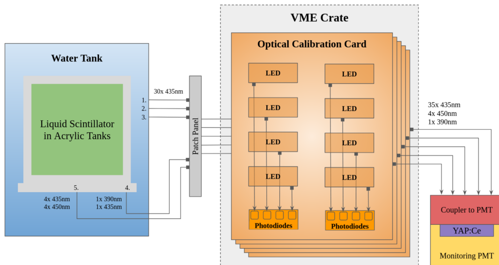
Figure 26: An overview of the OD Optical Calibration System, with eight LED pulsers on one Optical Calibration Card (OCC) and five OCCs in the VME crate. Lines with arrows show fibre routes with labels representing numbers of fibers from LEDs with corresponding wavelengths [91]. Labels 1-3 represent the three heights for the ten azimuthal positions, while Label 4-5 denote the injection points to monitor the bottom acrylic tanks, as shown in Figure 25.
