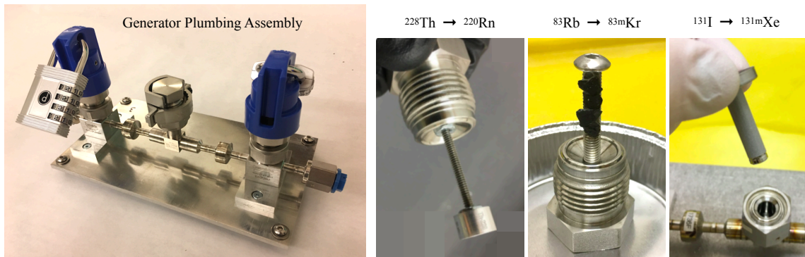
Figure 3: An example generator plumbing assembly along with three sets of parent material. The plumbing assembly is standardized such that any assembly can be mounted in any generator bay on the source injection panel shown in Figure 4. The assembly is welded as one piece to the extent possible, including the 3 nm pore-size sinter filters on either side of the 1/2-inch VCR access port. Various active parent materials can be installed via this access port: a platinum disk with electroplated ^{228}\text{Th} for ^{220}\text{Rn} generation, several charcoal pieces dosed with ^{83}\text{Rb} for ^{83\text{m}}\text{Kr} generation, and a VCR gasket combined with a sintered “cup” which retains ^{131}\text{I} -dosed \text{NaH}_2\text{PO}_4 grains for ^{131\text{m}}\text{Xe} generation.
