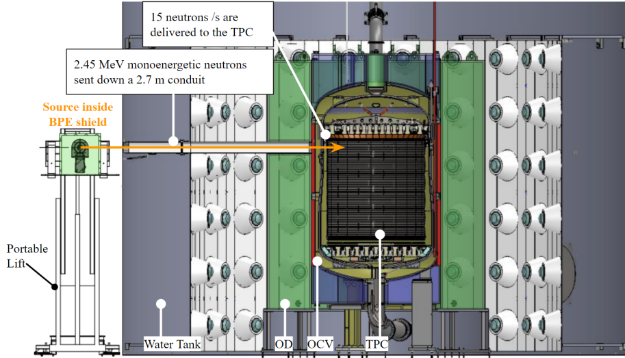
Figure 16: A CAD drawing of DD neutron generator deployment in the LZ experiment with respect to the horizontal conduit. In the Direct mode, monoenergetic 2.45 MeV neutrons are directly sent down the conduit. The angled conduit is 90^\circ off from the horizontal conduit, which is presented in Figure 2 but not shown here. During calibration, the generator surrounded by borated polyethylene (BPE) is positioned outside the water tank on a portable lift. The neutron beam is collimated by the nitrogen-purged conduits which traverses the water tank and the OD.
