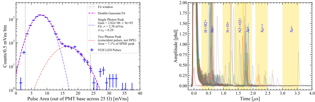
Figure 24: Left: A regular calibration of the Xe PMT system includes the per-PMT measurements of gain. PMT gain is determined through a double-Gaussian fit to the PhE pulse area spectrum from LED generated light. Right: Calibration of the afterpulsing ratio (APR). High intensity LED pulses are used to induce afterpulses in each PMT. Traces from many LED pulses (shown above) are co-added. APR is then measured as the ratio of the total area of each ion population to the combined area of the primary LED pulses. The timing of a single afterpulse for a particular ion is given by its mass, and shown by the yellow shaded bands.
