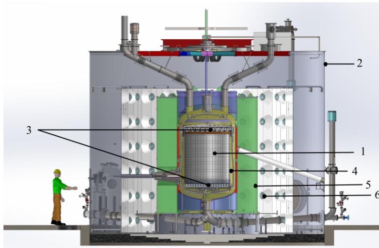
Figure 1: Overview of LZ detectors consisting of the central TPC detector (1) surrounded by the Skin detector (4) and the OD (5) volumes. The OD is filled with gadolinium-loaded liquid scintillator and viewed by OD PMTs (6). All three detectors are enclosed in a water tank (2) filled with high purity water. The PMT arrays (3) monitoring the TPC xenon volume are also shown.
