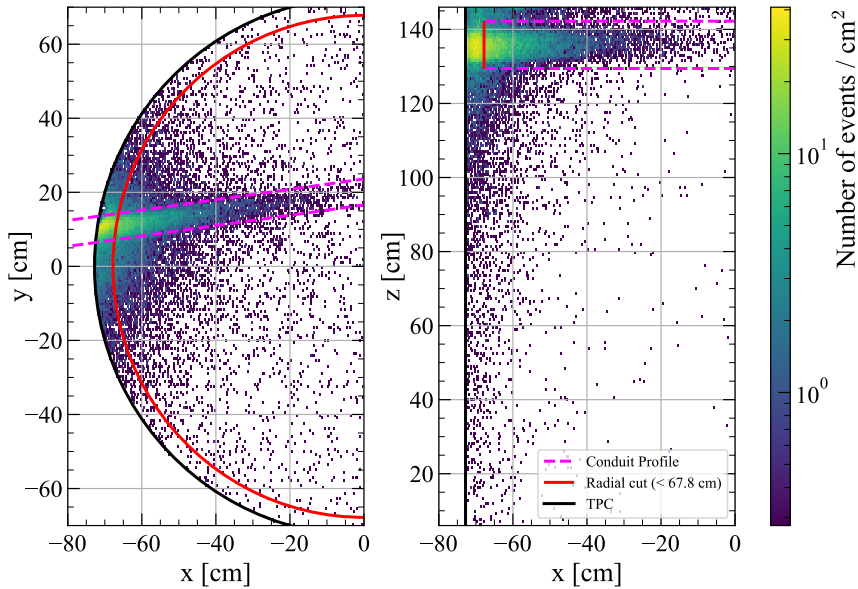
Figure 17: Reconstructed positions of events from the Direct mode DD calibration data in the Cartesian x , y , z coordinates of the TPC. Events that are more than 5 cm away (dotted red line) from the TPC wall and between 129 cm and 142 cm above the cathode are used for DD neutron analysis. The neutron beam is collimated by a 4.9 cm diameter conduit and its profile is shown as the dashed purple line.
