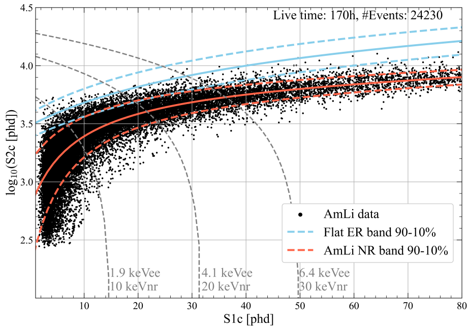
Figure 13: Detector response to the AmLi source in LZ. The solid (dashed) blue line is the median (90-10% quantiles) of a flat ER distribution modelled using NEST 2.3.7 [57]. The solid (dashed) red line is the median (90-10% quantiles) of an NR band fitted to the AmLi data using a skewed Gaussian distribution [58]. The dashed grey lines are contours of constant energies. Only data points within 5-sigma of the fitted AmLi distribution are shown.
