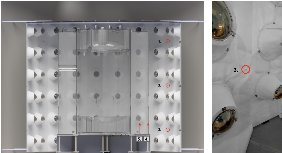
Figure 25: Left: A CAD drawing of the cross-section of the OD, showing the side acrylic tanks and the OD PMTs mounted on their ladders. The three nominal heights of the 10 azimuthal positions of the optical fiber injection points are labeled 1-3. Additionally, two injection points under the bottom acrylic tank are labeled 4 and 5. Right: A photo of the bottom OD PMT array showing one of the injection points.
