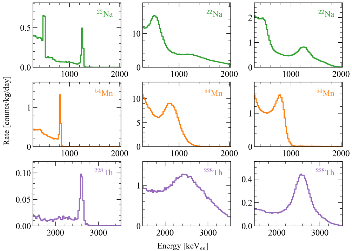
Figure 15: Measured energy spectra from ^{22}\text{Na} (511 keV from positron-electron annihilation and 1274 keV gammas), ^{54}\text{Mn} (835 keV), and ^{228}\text{Th} (2615 keV) in the TPC (left), Skin (middle) and OD (right). Only single scatter events are plotted. The energy range for the ^{228}\text{Th} data is different from the range used for the ^{22}\text{Na} and ^{54}\text{Mn} data. Data are taken using the above three gamma sources positioned at z=70 cm above the TPC cathode. Spectral peaks from these sources are reconstructed at their expected values.
