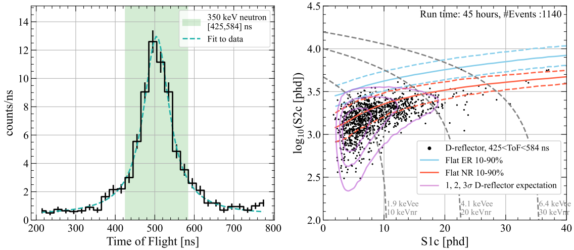
Figure 19: Left: Time of flight (ToF) distribution of neutron events from the D-Reflector calibration in the LZ experiment. The peak is at 505 \pm 2 ns, which corresponds to a neutron kinetic energy of 349 \pm 3 keV. This is close to the desired 350 keV neutrons with a ToF of \sim 500 ns given the distance between the generator and the TPC. Events within the green box are selected for the analysis based on expected ToF of neutron events from the D-Reflector. Right: Detector response to D-Reflector events with ToF between 425 and 584 ns as indicated by the green box on the left plot. The solid red (blue) line is the median of a flat NR (ER) distribution and the dashed red (blue) lines are the 10-90% quantiles modelled using NEST 2.3.7 [57]. The dashed grey lines are contours of constant energies. Purple contours are the expected S1 and S2 distribution of neutrons from the D-reflector. Most events are within the contours as expected.
