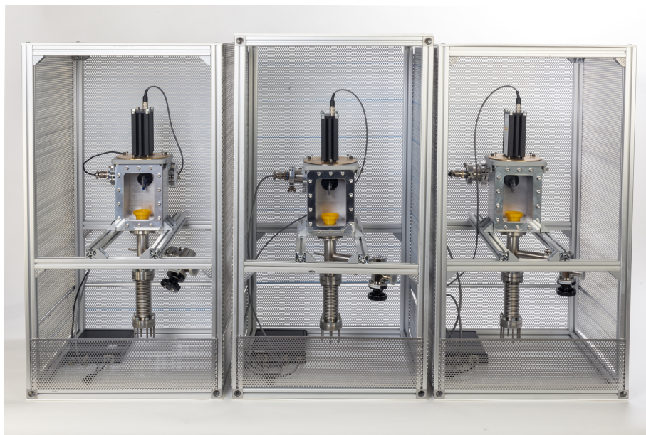
Figure 9: The three CSD units fully assembled before their installation at SURF.
