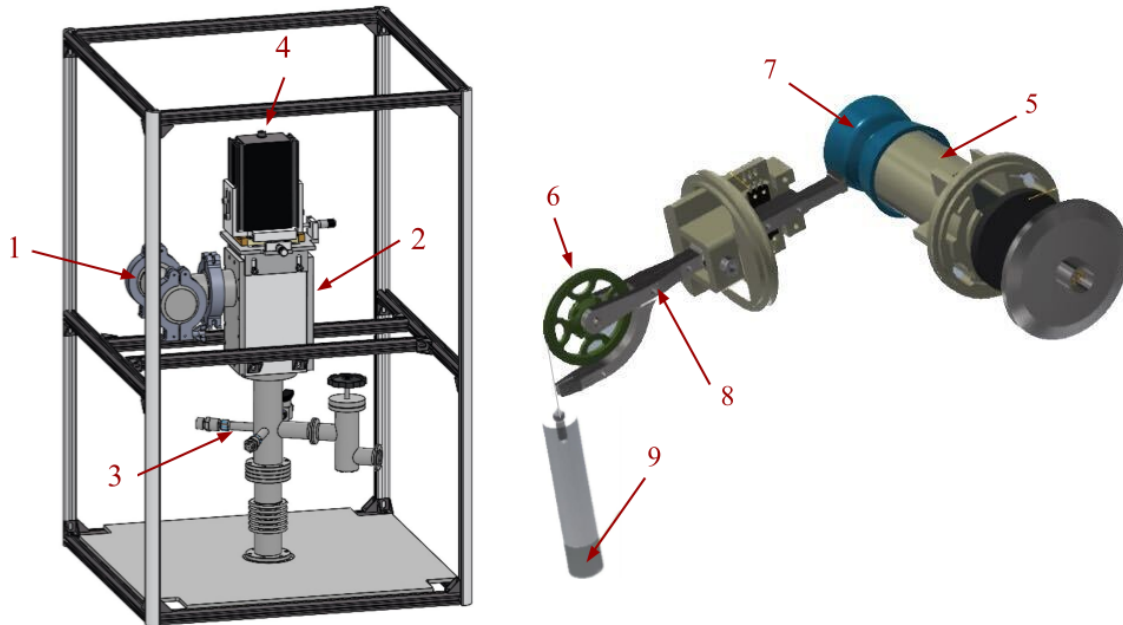
Figure 8: Left: CAD drawing of the main components of the CSD system caged in its protective frame: (1) Tee-Piece containing the deployment mechanics; (2) Source connection chamber with deployment wheel and filament lever; (3) 6-way connection piece with \text{N}_2 purge, pressure relief, and vacuum valves; (4) Laser position feedback system. Right: the internal deployment system concealed within the T-piece (1) including a stepper motor (5), a deployment wheel (6), a filament drum (7), a lever (8) and a calibration source (9).
