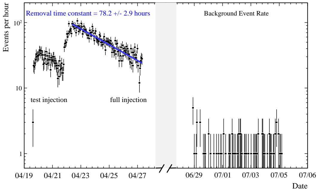
Figure 7: A low-activity test injection of tritiated methane ( \text{CH}_3\text{T} ) followed by the main injection for an ER calibration in 2022. The removal time constant for \text{CH}_3\text{T} is 78.2 \pm 2.9 hours, measured by fitting an exponential to the time profile of the measured \text{CH}_3\text{T} event rate in the TPC. The exponential fit to the data is represented by the blue line in the plot. The right half shows the normal background event rate during the science run when all the tritium has been removed. The grey band represents the time gap between the tritium calibration and the science run.
