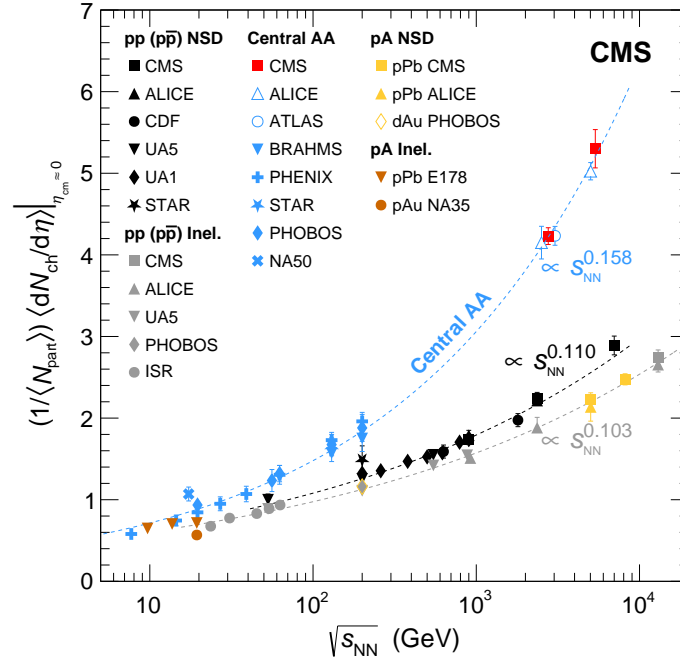
Figure 4: Comparison of average dN_{\text{ch}}/d\eta at midrapidity, scaled by \langle N_{\text{part}} \rangle in pPb [22, 43], pAu [44], dAu [45–47] (pA) and central heavy ion collisions [8, 12, 41, 42, 46, 48–56], as well as non-single-diffractive (NSD) [17, 18, 56–59] and inelastic [21, 42, 60, 61] pp collisions. The data points for nucleus-nucleus (AA) collisions at \sqrt{s_{\text{NN}}} = 2.76 TeV have been shifted horizontally for visibility. The dashed curves, reproduced from Ref. [22], are included to guide the eye, and correspond to a power law functional form.
