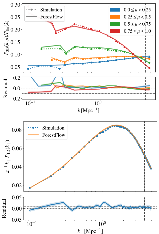
Fig. 4. Accuracy of the emulator in recovering P_{3\text{D}} and P_{1\text{D}} measurements from the CENTRAL simulation at z = 3 . Dotted lines show measurements from simulations, solid lines and shaded areas display the average and 68% credible interval of FORESTFLOW predictions, respectively, and vertical dashed lines indicate the minimum scales considered for computing the training data of the emulator. The overall performance of the emulator in recovering P_{3\text{D}} is 2.0% on scales not strongly affected by cosmic variance and 0.6% for P_{1\text{D}} .
