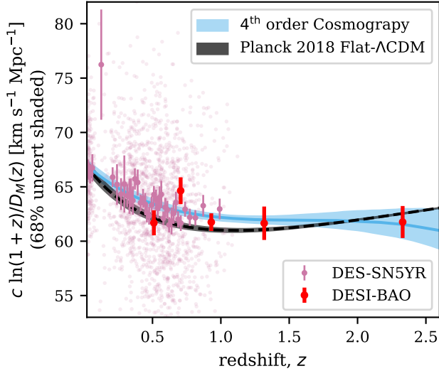
Figure 2. Illustration of the inverse distance ladder method. The pink supernova data points from DES-SN5YR have been calibrated to the red data points from DESI-BAO, and the resulting y-intercept gives H_0 . For DESI-BAO we plot only the five D_M(z)/r_d points and their statistical uncertainties. For the DES-SN5YR sample we show both the individual SN events (transparent) and the redshift-binned SN distance moduli (opaque with redshift-binned statistical uncertainties) after calibration. The blue line represents the best fit 4 th order cosmographic model determined with the DES-SN5YR + DESI-BAO datasets. The black dashed line shows the best fit from Planck (Aghanim et al. 2020), determined by analysing the CMB and assuming Flat- \Lambda CDM.
