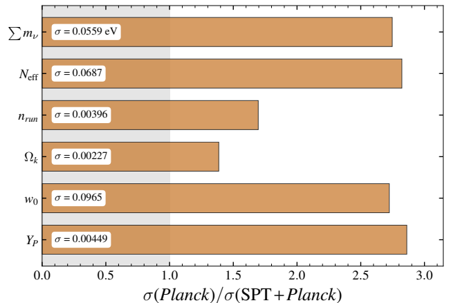
Figure 9. Ratio of 1\sigma constraints on single-parameter extensions from Planck to those forecasted from the combination of Ext-10k and Planck . The gray shaded region corresponds to the current best constraints from Planck alone. The actual errors are expressed in the text boxes.
