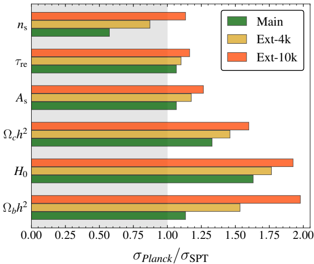
Figure 8. Constraints on the standard \Lambda CDM parameters expected from combinations of the three SPT-3G surveys (SPT-3G Main in green, Ext-4k in yellow, and Ext-10k in red) compared to Planck (grey shaded region). We expect significant improvements on all the parameters except n_s and \tau_{\text{re}} which depend on the largest scales that ground-based surveys cannot easily measure.
