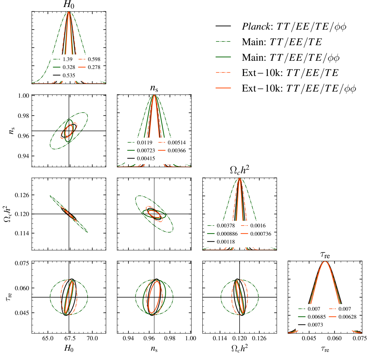
Figure 13. Marginalized 1-dimensional and 2-dimensional 68% contours for Hubble constant ( H_0 ), scalar spectral index ( n_s ), Cold dark matter density ( \Omega_c h^2 ), and optical depth ( \tau_{re} ) with (solid) and without (dashed) lensing for SPT-3G Main (dark green), Ext-10k (dark red) and Planck (black). The inclusion of the lensing spectra significantly helps to break the degeneracies especially for the SPT-3G Main survey. The 1\sigma errors are listed in the legend.
