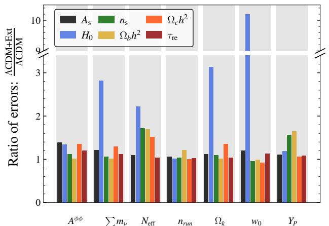
Figure 10. Degradation in the \Lambda CDM constraints due to single-parameter extensions compared to the original constraints reported in Fig. 8 for the Ext-10k+ Planck dataset. The horizontal axis shows the parameter that is varied in our extensions. Except for H_0 , which is affected by a geometric parameter degeneracy, the degradation in constraints for other \Lambda CDM parameters is quite mild.
