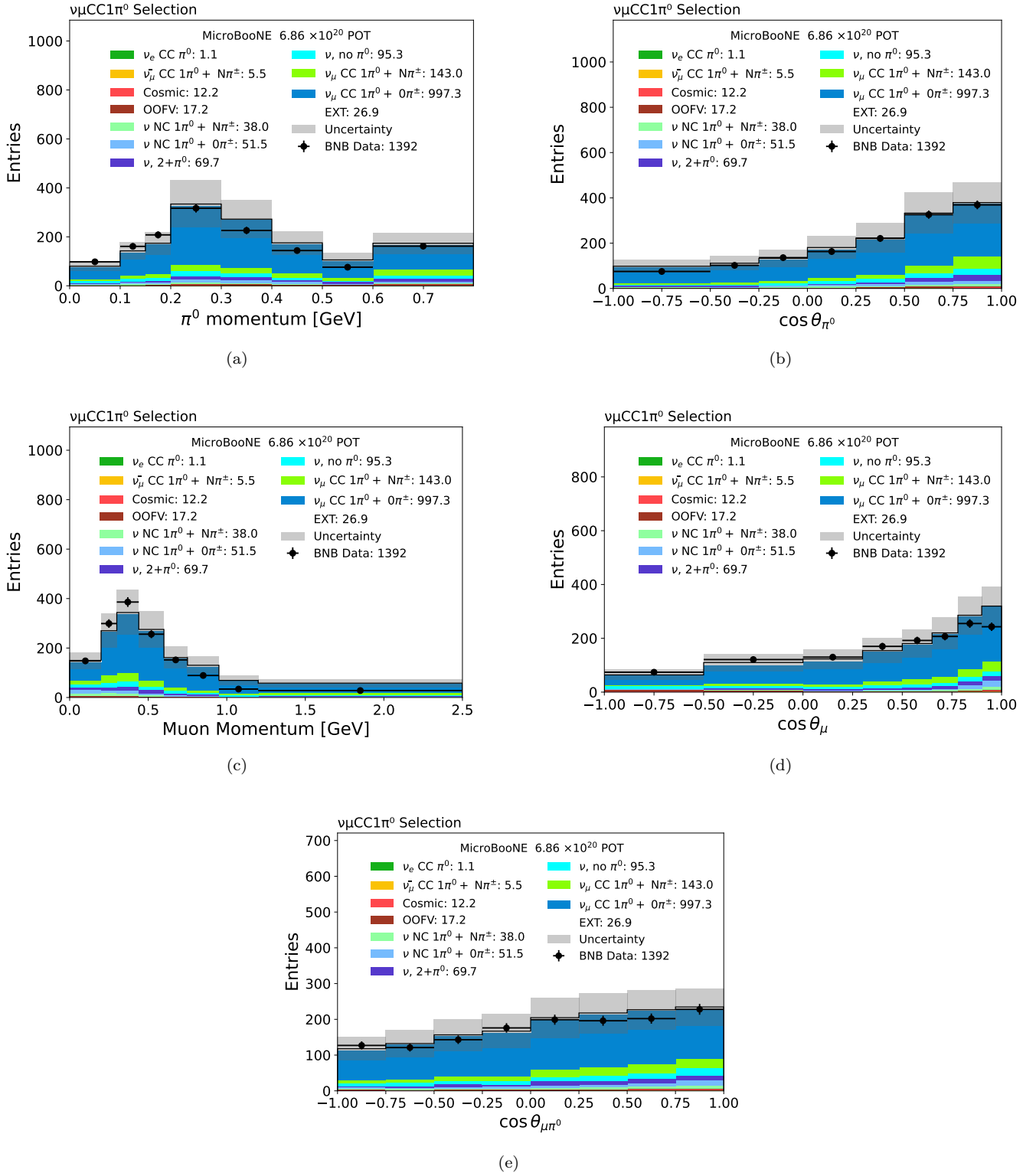
FIG. 1. Comparison of the distribution of the number of events observed in data and the prediction of the MicroBooNE tuned version of GENIE v3 satisfying the \nu_{\mu}\text{CC}1\pi^0 selection requirements for (a) the \pi^0 momentum, (b) the scattering angle between the neutrino beam and outgoing \pi^0 direction, (c) the muon momentum, (d) the scattering angle between the neutrino beam and outgoing muon direction, and (e) the opening angle between the muon and pion are shown. The last bin in the momentum distributions acts as an overflow bin. The shaded gray band indicates the total (includes both statistical and systematic) uncertainty on the simulation prediction. The event categories are described in the legend. The OOFV category includes background events in which the true neutrino vertex is located outside the fiducial volume.
