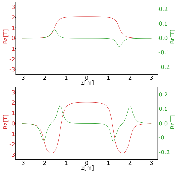
Figure 1: Longitudinal (red) and radial (green) magnetic fields along the 15 mrad axis in the two compensation schemes (standard proposed here on the top, baseline on the bottom).
