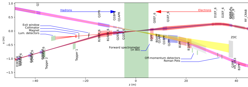
Figure 1: Layout of the interaction region. The IP is located at the origin. Shown in green is the central detector. Dipole and quadrupole magnet apertures are shown in pink and blue, respectively. The neutron cone is shown in yellow. Beam envelopes ( 13.5\sigma and 10\sigma for electrons and protons, respectively) are shown for 275 GeV protons and 18 GeV electrons.
