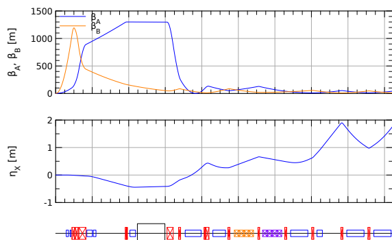
Figure 2: Lattice functions for the hadron forward side, 275 GeV protons, from the IP to the RHIC arc.
