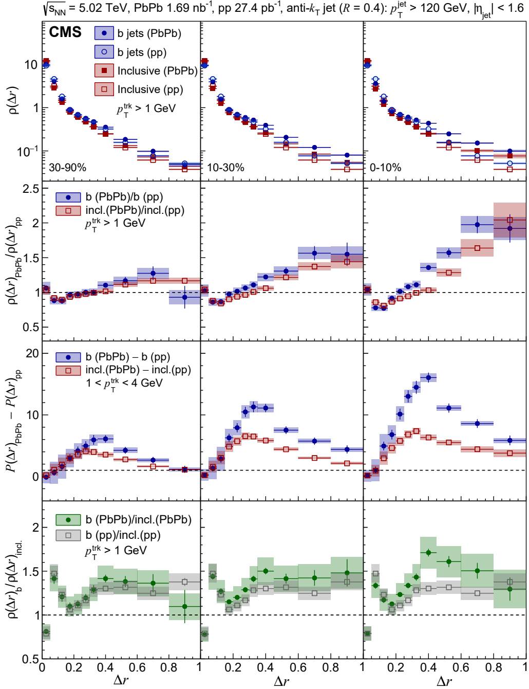
Figure 1: Upper row: jet shape distributions \rho(\Delta r) for inclusive (solid red squares) and b jets (solid blue circles) with p_T > 120 \text{ GeV} in three centrality bins (left to right) for PbPb collisions at \sqrt{s_{\text{NN}}} = 5.02 \text{ TeV} , as well as in pp collisions (open red and blue symbols) from Ref. [16], which are identical in all three panels. Second row: ratio of PbPb to pp jet shape results for inclusive (red) and b jets (blue). Third row: the difference between the charged-particle transverse momentum profile, defined by Eq. 1, between PbPb and pp collisions for 1 < p_T^{\text{trk}} < 4 \text{ GeV} for inclusive (red) and b jets (blue). Lower row: ratio of b to inclusive jet shapes for several PbPb centrality bins (green), as well as pp collisions from Ref. [16] (grey), which are identical in all three panels. In all panels, the vertical bars and shaded boxes represent the statistical and systematic uncertainties, respectively.
