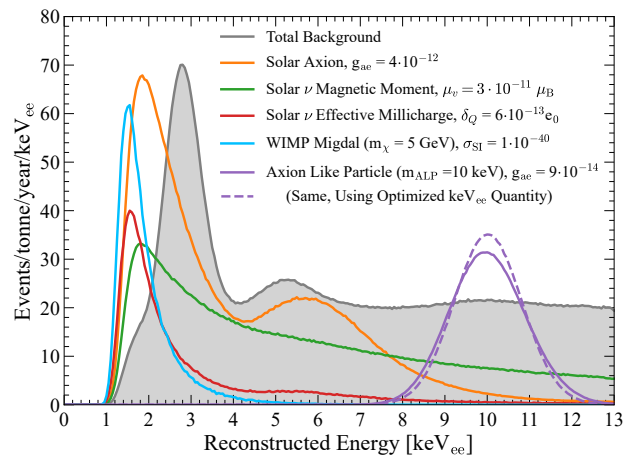
Figure 3: Reconstructed energy ( \text{keV}_{ee} ) spectra for the background-only model (grey) and representative signal models: solar axion (orange), solar neutrino magnetic moment (green), solar neutrino millicharge (red), spin independent WIMPs undergoing Migdal effect (blue), and axion like particles (ALPs) (purple). To produce these spectra, the detector S1 and S2 response is simulated and then all data selections, thresholds, and data quality acceptances are applied. This standard reconstructed energy quantity can be improved by applying an unequal weighting to the sum of S1c and S2c (see text for details), and we illustrate the advantage of an unequal weighting by showing an alternative reconstruction of the example ALP signal.
