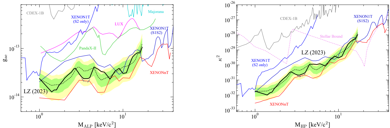
Figure 7: The 90% C.L. upper limit (black line) on ALP coupling constant, g_{ae} (left panel), and the HP coupling constant squared, \kappa^2 (right panel). Selected limits from other experiments are also shown [4, 66, 75, 77, 79, 84–86] along with astrophysical bounds in Ref. [87].
