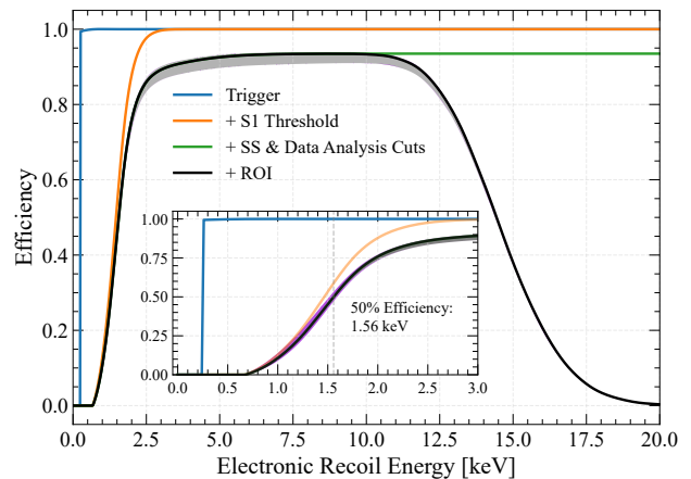
Figure 2: Signal efficiency as a function of true ER energy for the trigger (blue), the \geq 3 -fold coincidence and >3 phd threshold on S1c (orange), single-scatter (SS) reconstruction and analysis cuts (green), and the search ROI in S1 and S2 (black). The inset shows the low energy behavior, with the dotted line at 1.56 \text{ keV} marking 50% efficiency. The data quality acceptance error band (gray) is assessed using AmLi and tritium data. The NEST model uncertainties (purple) are discussed in Appendix A.
