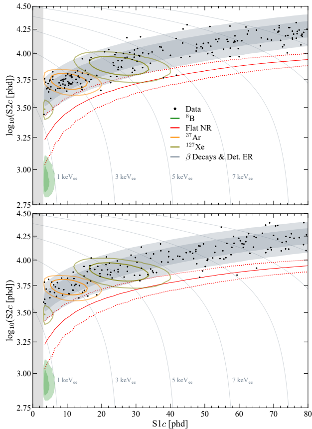
Figure 1: The SR1 search data (black points) is plotted in the \{S1c, \log_{10}S2c\} space, after all cuts and selections are applied. For illustration purposes, the exposure is shown separated into two periods of equal livetime (top panel is the first half of SR1, bottom panel is the second half). In both panels, the 1\sigma and 2\sigma regions are indicated for various background model components: ^{37}\text{Ar} (orange contours), ^{127}\text{Xe} (green contours), ^8\text{B} (filled green), and the broad-spectrum ER background encompassing ^{212}\text{Pb} , ^{214}\text{Pb} , ^{85}\text{Kr} , and external gammas (filled gray). The solid red line indicates the median, the dashed the 10% and 90% quantiles of a flat NR background. Thin gray lines indicate contours of constant ER energy, with a spacing of 2 \text{ keV}_{ee} . A reduction in ^{37}\text{Ar} rate is the dominant change between the two time periods.
