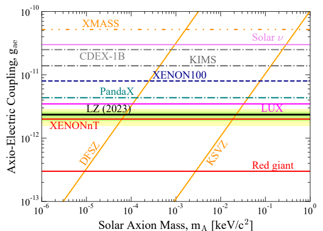
Figure 6: The 90% C.L. upper limit (black line) on solar axion g_{ae} coupling constant. Selected limits from other experiments and astrophysical observations are also shown [4, 62, 74–79]. The shaded orange region corresponds to predicted values from the benchmark QCD axion models DFSZ [80, 81] and KSVZ [82, 83]. The LZ median sensitivity is not displayed due to close overlap with the observed limit.
