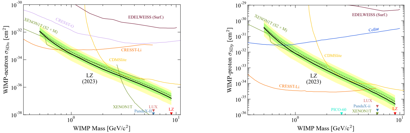
Figure 9: The 90% C.L. upper limit (black line) for the spin dependent WIMP cross-section versus WIMP mass for coupling on neutrons (left) and protons (right) undergoing the Migdal effect. The SD proton and neutron modes use the mean nuclear structure functions from [64]. Also shown are limits from other experiments [40, 41, 84, 89, 90, 96–98].
