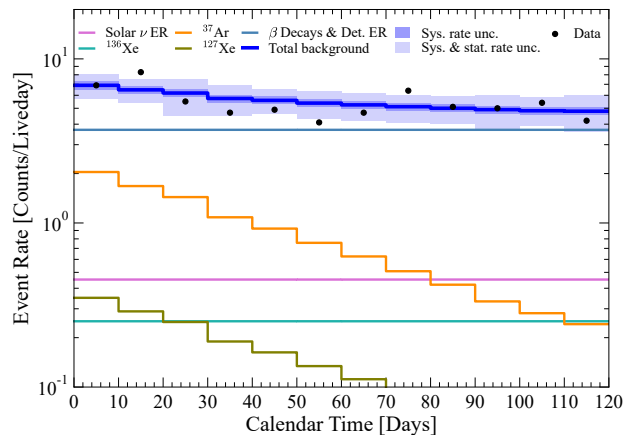
Figure 4: Time dependence of the data and the best-fit model. Statistical tests are performed on observed and expected counts, while in this plot counts are converted to rates by normalizing by the livetime fraction of each 10-day bin. Data is shown in black. The blue line shows total summed background. The darker blue band shows the 1\sigma model uncertainty and the lighter blue band the combined model and statistical uncertainty. Background components are shown in colors as given in the legend. All background components are included in the fit, but those appearing exclusively below the y-axis bound are not listed in the legend.
