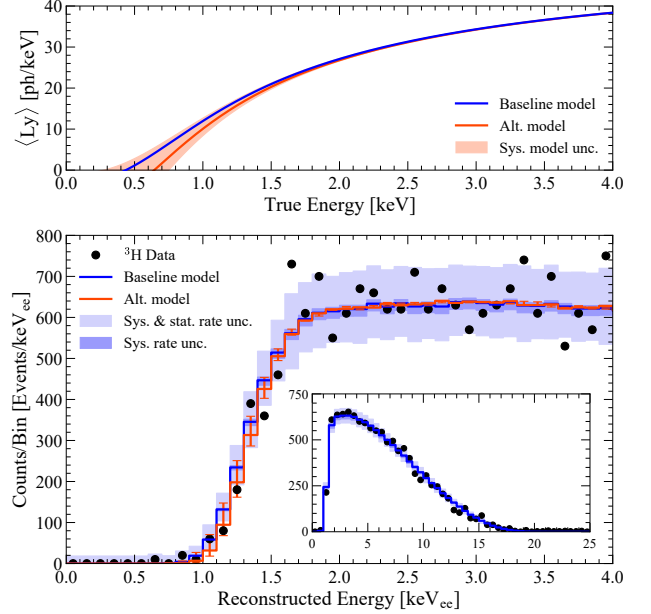
Figure 10: Top panel: The ‘baseline’ (global fit) LXe response model and the ‘alternative’ (LZ tritium-fitted) response models, as referred to in this section, both illustrated as light yields L_y . The fit uncertainty on the alternative model is also shown. Lower panel:
