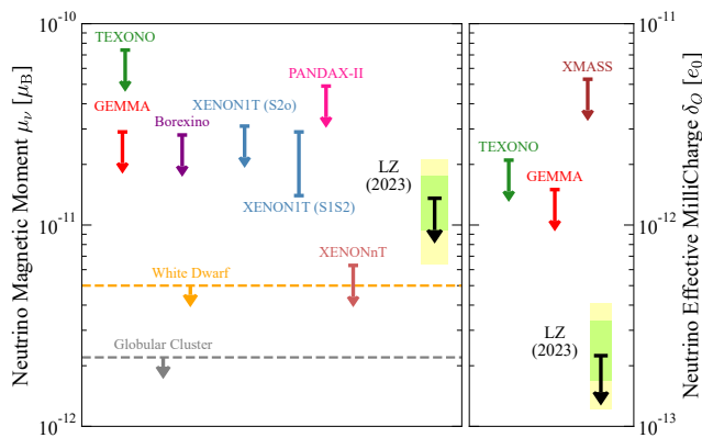
Figure 5: The 90% C.L. upper limit on effective neutrino magnetic moment (left) and neutrino effective millicharge (right). Selected limits from other experiments are also shown [4, 66–71] and astrophysical observations [59, 60].
