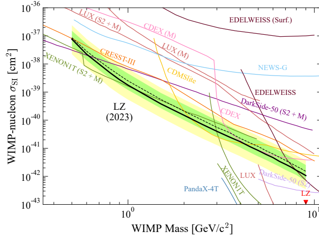
Figure 8: The 90% C.L. upper limit (black line) for the Spin Independent WIMP cross-section vs. WIMP mass, using the Migdal signal pathway. Also shown are limits from other experiments [1–3, 39–43, 84, 88–95].
