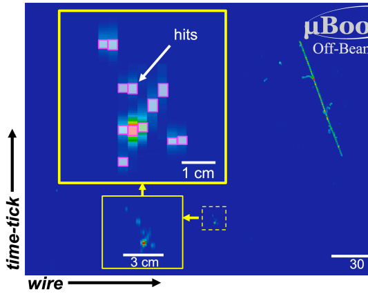
FIG. 2. A section of a MicroBooNE LArTPC eve from data. Each vertical column of pixels represent wire. The rainbow color spectrum denotes charge per 500 ns ADC time tick, with redder colors indicate charge densities. A grouping of hits across 10 wire randomly-selected area of interest spanning about 3 cm is represented in the zoomed inset as a set of pink boxes. The extent of each box along the vertical (time) axis is the hit's RMS width. A cosmic muon track can be seen on the right.
