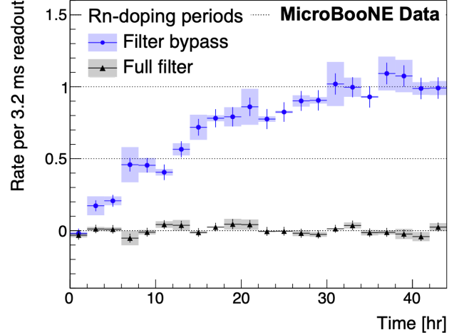
FIG. 11. Measured rate of BiPo decays per readout within the fiducial volume, plotted against the time of the event relative to the start of each Rn-doping data-taking period. Statistical errors are represented by solid lines, while systematic errors from uncertainties in the fit methodology as described in the text are represented by shaded regions.
