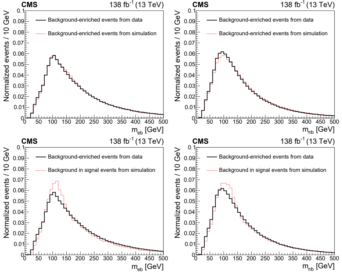
Figure 3: The normalized m_{\ell b} distributions for the electron (left) and muon (right) channels. The upper two plots compare the background-enriched distributions from data (solid line) to the MC predictions (dotted-red line). The lower two plots give the background-enriched distributions from data (solid line) and the MC predictions for the distributions from the background in the signal events.
