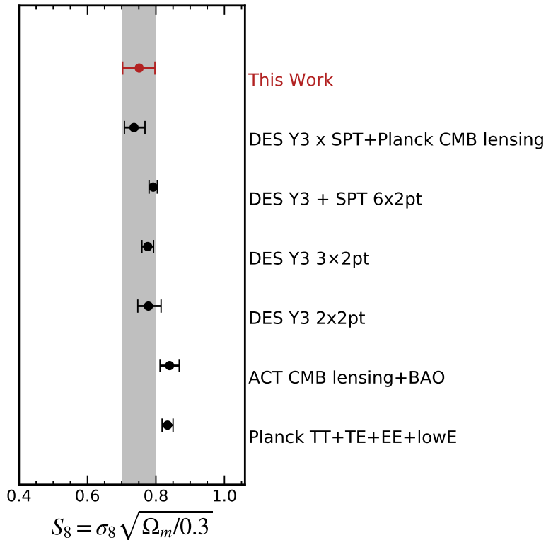
Figure 17: Comparison of measurement of S_8 from our analysis with other measurements using DES Y3 data [6, 36, 62, 107], ACT CMB lensing + BAO [19], and primordial CMB from Planck [1], though note that the DES points here include marginalization over the sum of neutrino masses.
