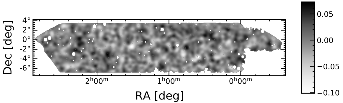
Figure 1: CMB convergence map of the d56 region, reconstructed from the combination of tSZ-cleaned ACT and Planck data [42]. The map is smoothed with a Gaussian beam with 20 arcmin for visualization purposes only. Data in the white regions are masked out regions.
