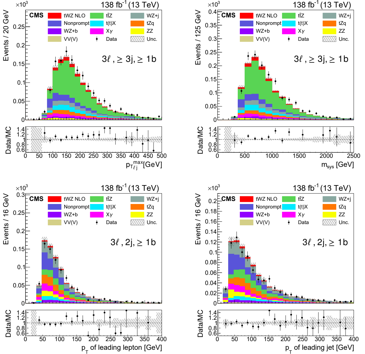
Figure 2: Pre-fit examples of the input features for the two DNN trainings: the p_{T\ell_j}^{\max} (upper left) and m_{\text{sys}} (upper right) observables in \text{SR}_{3\ell, \ge 3j} , as well as the p_T of the leading lepton (lower left) and leading jet (lower right) in \text{SR}_{3\ell, 2j} . The VV(V) group in the legend denotes the VVV, WW, and W in association with jets backgrounds. The dashed band shows the total uncertainty (statistical and systematic) before the fit.
