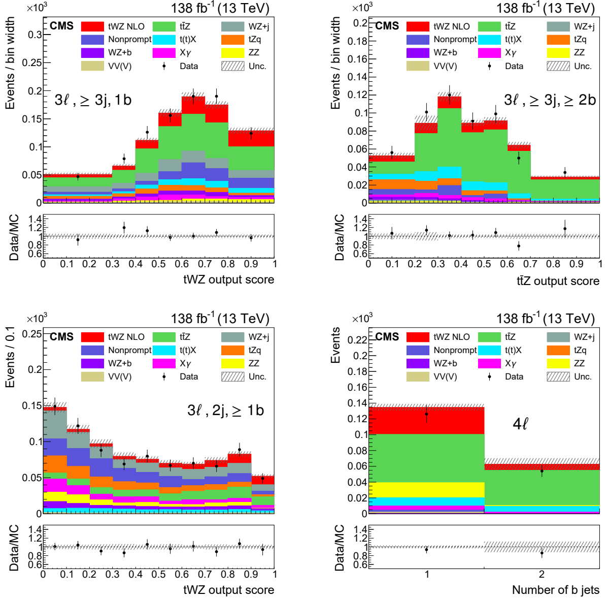
Figure 3: Score of the tWZ output node from the multiclass classifier in SR 3ℓ,3j for events with exactly one b jet (upper left), and of the t̄tZ output node in SR 3ℓ,3j for events with more than one b jet (upper right); score of the tWZ output node of the binary classifier in SR 3ℓ,2j (lower left), and the b jet multiplicity in SR 4ℓ (lower right). The VV(V) group in the legend denotes the VVV, WW, and W in association with jets backgrounds. The dashed band shows the total uncertainty (statistical and systematic) after the fit.
