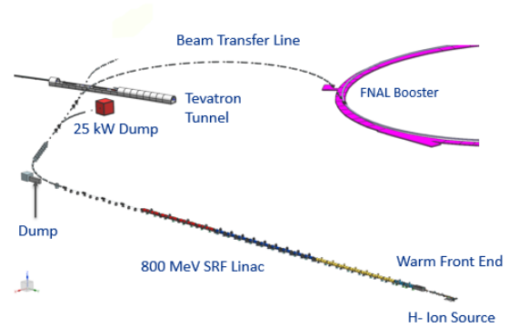
Figure 2: PIP-II scope: new LINAC and beam transfer line to Booster
