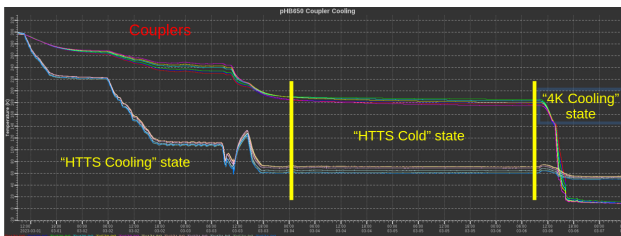
Figure 5: Archived data of the RF coupler cooldown of a prototype HB650 CM
