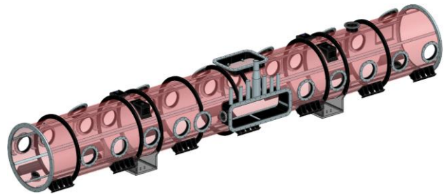
Figure 16: Skeleton on the inside of the vacuum vessel.
