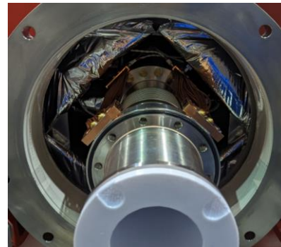
Figure 5: Warm part of the coupler going through the thermal shield.
