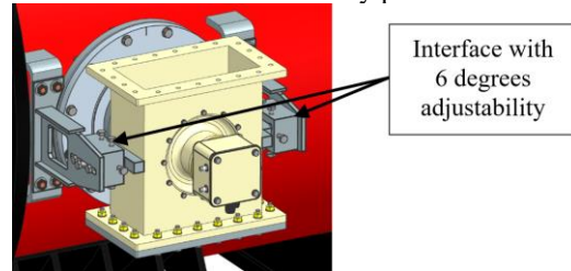
Figure 15: Production coupler / vacuum vessel interface.
