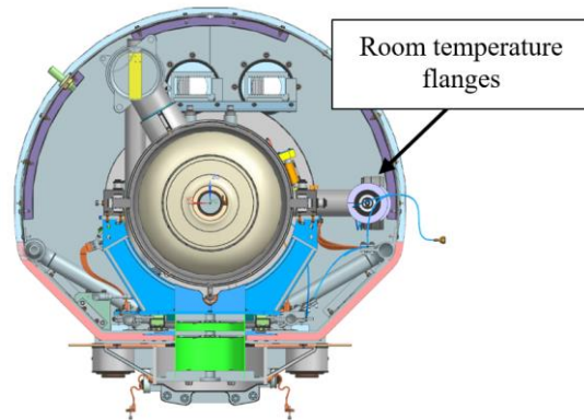
Figure 4: Coldmass cross section.
