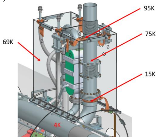
Figure 8: Temperature values with cavities at 4K.
