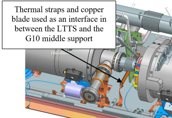
Figure 10: LTTS / G10 middle support interface.
