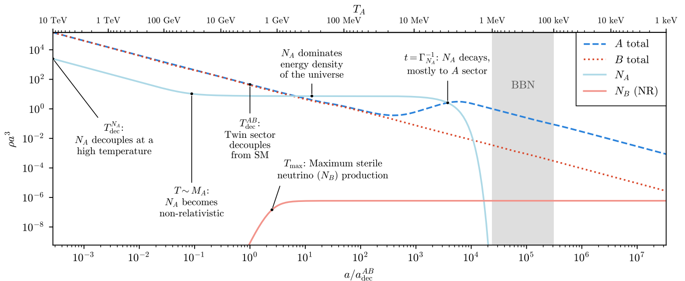
FIG. 1. Timeline of events in one realization of our scenario. The curves indicate the comoving energy densities of radiation in the SM ( A ) and twin ( B ) sectors, and of the sterile neutrinos, N_A and N_B , as a function of scale factor, a , or the temperature of the SM bath, T_A . The y -axis is normalized by the comoving energy density of the SM sector at T_A = 1 MeV. Only the non-relativistic portion of \rho_{N_B} = M_{N_B} n_{N_B} is shown. This example takes the parameters M_{N_A} = 100 GeV, m_{\nu_A} = 10^{-9} eV, M_{N_B} = 100 keV, and m_{\nu_B} = 4 \times 10^{-4} eV, for which we find \Delta N_{\text{eff}} \approx 0.02 and \Omega_{N_B} \approx 0.26 , consistent with observations.
