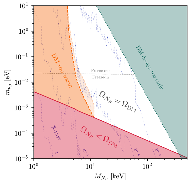
FIG. 3. Constraints on the masses of our dark matter candidate, N_B , and the twin sector active neutrino, \nu_B . Shaded regions indicate constraints on the DM abundance (red), temperature (orange), and lifetime (green). Throughout the white region labeled “ \Omega_{N_B} = \Omega_{\text{DM}} ” our model can produce the observed DM abundance while remaining consistent with the constraints on \Delta N_{\text{eff}} . The dotted blue lines represent constraints on DM decay to X-ray lines for several values of the branching ratio \Gamma_{N_B \rightarrow \nu_A \gamma_A} / \Gamma_{N_B \rightarrow \nu_B \gamma_B} ; for each choice of this ratio, the parameter space to the right is excluded.
