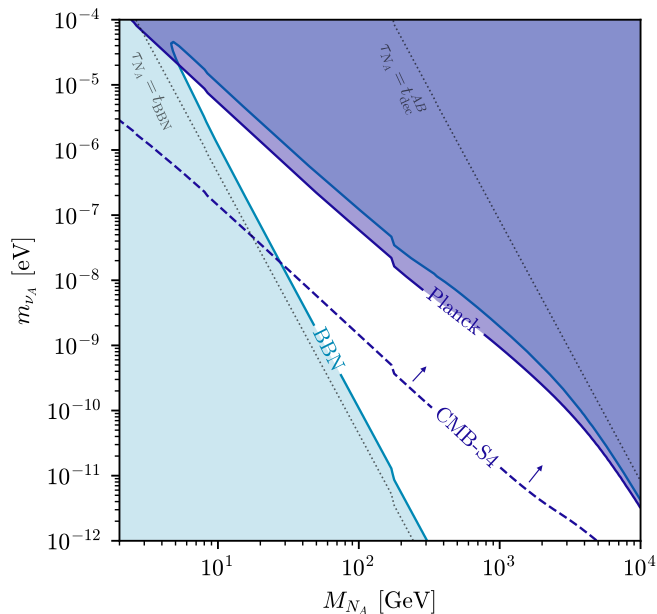
FIG. 2. Constraints on the masses of the decaying sterile neutrino, N_A , and the corresponding active neutrino, \nu_A , from measurements of N_{\text{eff}} . The shaded regions represent the parameter space that is ruled out by measurements of the light element abundances [76] (light blue) and the cosmic microwave background (dark blue). Current \Delta N_{\text{eff}}^{\text{CMB}} constraints are shown from Planck [77] as well as the projected sensitivity of Stage 4 CMB experiments [78]. In the unshaded regions, the decays of the N_A dilute the energy density of the twin sector to acceptable levels. Dotted gray lines represent curves of constant \tau_{N_A} .
