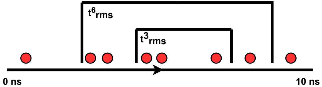
Figure 9. The selection of t_{rms} hit clusters. Optimal selections for clusters of 3-6 hits are shown for an example candidate where t_{rms} = 8 . Possible background hits on the fringes of the candidate time are ignored.
