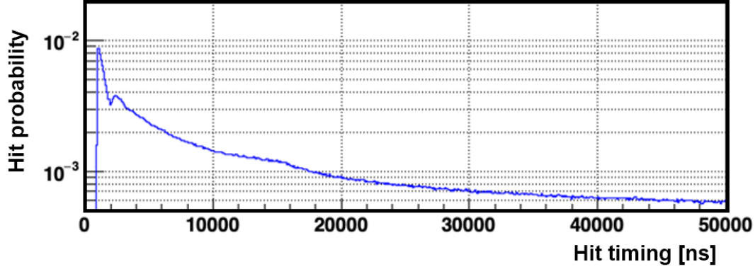
Figure 19. Timing distribution of repeated hits (noise rate) following a signal pulse above the discriminator threshold (0.25 p.e.) of a 20-inch PMT. The X axis shows the timing difference of a repeated hit from the initial hit and the Y axis shows the probability of the secondary hit. The gap between 0 to 1 \mu s is due to the channel dead time of the readout electronics and the peak around 1.5 \mu s is due to the reflection of the PMT signal. The repeat noise rate decreases exponentially in time and the feature around 12 to 18 \mu s is due to PMT after-pulsing.
