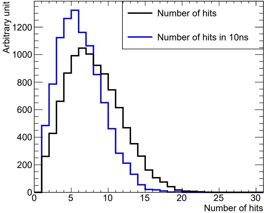
Figure 4. Number of hit PMTs in SK for 2.2 MeV \bar{\nu}_0 using the SK detector simulation program. No noise are simulated and only the Cherenkov photons from the 2.2 MeV \bar{\nu}_0 are recorded. The black histogram shows the total number of PMT hits. The blue histogram shows the largest number of hit PMTs in 10 ns obtained by using the 10 ns sliding window. In searching for the largest number of hit PMTs, the time-of-flight (ToF) from the generated point of 2.2 MeV \bar{\nu}_0 is subtracted from each timing of PMT hit.
