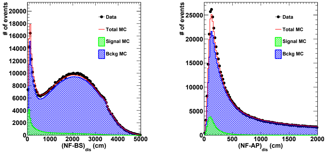
Figure 27. Distributions of the distance between the reconstructed vertices of Neut-Fit and BONSAI, _{dis} (left), and the distance between Neut-Fit the reconstructed vertices of Neut-Fit and APFit, _{dis} (right). These two values are expected to have a peak close to 0 because the vertices from the two different reconstructions are expected to be similar for signal but this is not necessarily true for the background.
