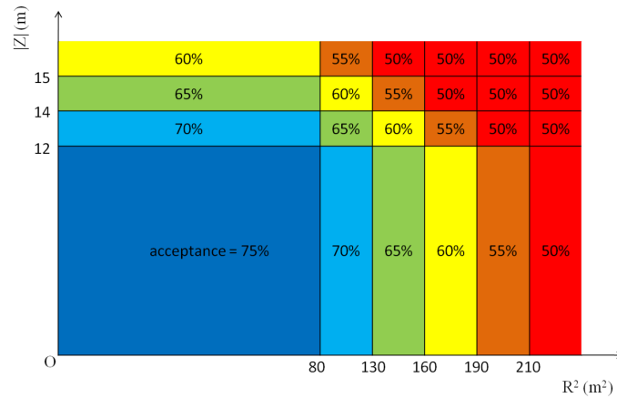
Figure 29. Varying acceptance requirements for the _{low} cut as a function of tank coordinates.
