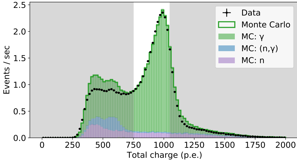
Figure 15. Total photo-electrons from 4.43 MeV scintillation events with the Am-Be source positioned at the center of the tank. The black points show the data. The histogram shows the distribution obtained by the Monte-Carlo simulation. The green shaded area corresponds to the events originated by \gamma , the blue shaded area corresponds to the events originated by neutron and \gamma , and the purple shaded area corresponds to the events originated by neutron. Events with 750 p.e. < 1050 were selected to trigger 4.43 MeV events. The Monte-Carlo histogram is normalized to the number of events of the data, whose total charge is 750 p.e. < 1050. The events in the gray shaded area are not used for the analysis.
