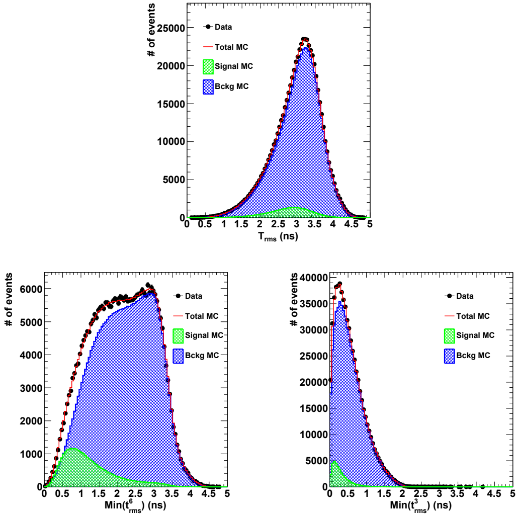
Figure 21. Distributions of the root-mean-square of the ToF-subtracted timing of candidate hits, T_{rms} (top), the minimum root-mean-square of hit timing ( min_{rms} ) of clusters of 6 hits, min(t_{rms}^6) (bottom left), and 3 hits, min(t_{rms}^3) (bottom right). The hits from the signal are expected to be concentrated in time and thus T_{rms} , min(t_{rms}^6) , and min(t_{rms}^3) are smaller compared to the background.
