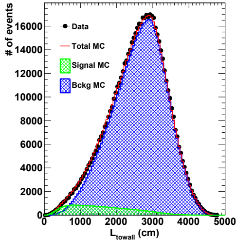
Figure 28. Distribution of the distance from Neut-Fit's reconstructed vertex to the ID wall in the direction of the particle, _{towall} . The background events tend to have larger value compared to the signal.
