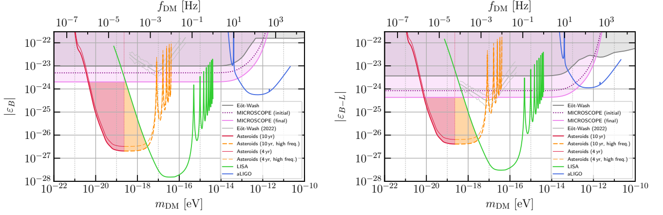
FIG. 1. Projected |\varepsilon_B| [left panel] and |\varepsilon_{B-L}| [right panel] sensitivity of various GW facilities/missions as labeled in the legends, assuming that the relevant dark photon is all of the local DM, \rho_{\text{DM}} = 0.3 \text{ GeV/cm}^3 . Mission parameters and sensitivities are given in Tab. I. Our main result is the sensitivity of the asteroid-ranging proposal [26], shown (for SNR of 1) as a combination of solid red and dashed orange lines. The solid red part of the curves is for f \lesssim 1/(5 \text{ hr}) , where asteroid rotational motion should not be inhibiting; the dashed orange part of the curves is for frequencies where asteroid rotational motion likely severely inhibits that proposal (see discussion in Ref. [26]). The red shaded region of parameter space could thus be accessed with the asteroid-ranging proposal (at SNR of 1), while the orange shaded region could only be accessed if noise issues associated with asteroid rotational motion could be overcome. We also show by the cognate thinner lines the sensitivity projections for a shorter, 4-year mission duration. The sensitivities we show for the LISA mission and the aLIGO facility (for comparative purposes and both also at SNR of 1) are in reasonable agreement with previous analyses [19, 21, 23–25], up to differences in assumed sensitivities and other mission/facility parameters. Also shown by solid medium-gray and violet lines and shaded regions, respectively, are the 95%-confidence static EP-test constraints (which do not depend on assuming the dark photon is all, or any, of the local dark matter) from the Eöt-Wash experiments [6–8] and from the final results of the MICROSCOPE mission [13] (re-cast using the method detailed in Ref. [12]; see discussion in text). The dotted purple line is the cognate limit obtained from the initial MICROSCOPE results [10]; see also Refs. [11, 24]. Recent Eöt-Wash results [labeled ‘Eöt-Wash (2022)’] from Ref. [9] (‘field along Z’ limits) are shown as light-gray lines, with the thick line representing the approximate exclusion limit averaged over nearby masses, and the limit at any specific mass fluctuating sharply within approximately the envelope denoted by the thin lines.
