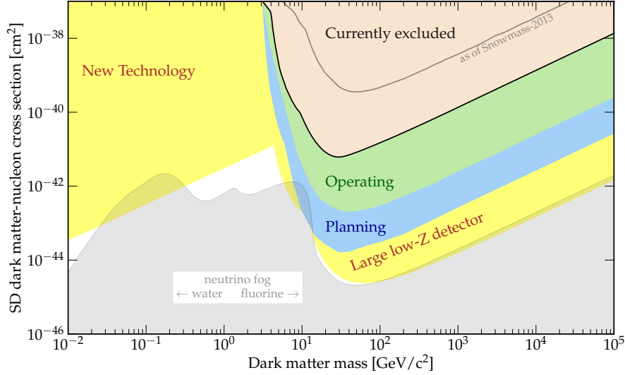
Figure 8: Combined Spin-dependent dark-matter nucleon scattering cross section space for scattering with neutrons or protons. Currently 90% c.l. constraints are shown in shaded beige [243, 257–267] (data points taken from [239]) while the reach of currently operating experiments are shown in green (LZ, XENONnT). The limits from 2013 are shown as a gray line [256]. Future experiments are shown in blue (PICO-500, 1000 ton year Xenon) and yellow (Snowball, PICO-100 ton). The neutrino fog for a water or fluorine target is presented in gray, as described in Sec. 4.3.2. Plot reproduced from Ref. [2].
