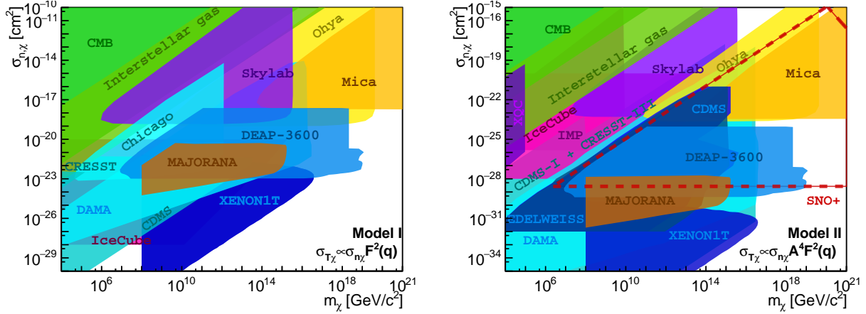
Figure 10: Current and projected experimental regions of ultraheavy parameter space excluded by cosmological/astrophysical constraints (green), direct detection DM detectors (blue), neutrino experiments (red/orange), space-based experiments (purple), and terrestrial track-based observations (yellow). Both models considered here assume different relations for the cross section scaling from a single nucleon to a nucleus with mass number A . In the left plot, we assume no scaling with A ; in the right plot, we assume the cross section scales like A^4 (e.g., with two powers coming from nuclear coherence, and two from kinematic factors). Limits are shown from DEAP-3600 [268], DAMA [269, 270], interstellar gas clouds [271, 272], a recast of CRESST and CDMS-I [273], a recast of CDMS and EDELWEISS [274, 275], a detector in U. Chicago [276], a XENON1T single-scatter analysis [277], tracks in the Skylab and Ohya plastic etch detectors [270], in ancient mica [278], the MAJORANA demonstrator [277], IceCube with 22 strings [279], XQC [280], CMB measurements [281, 282], and IMP [283]. Also shown is the future reach of the liquid scintillator detector SNO+ as estimated in [230, 284]. Reproduced from Ref. [9].
