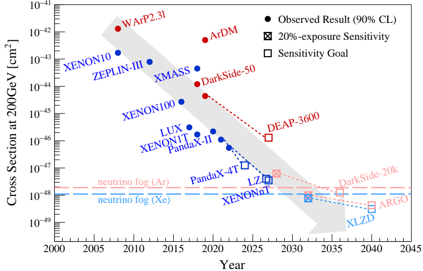
Figure 11: Figure adapted from [304]. Improvement in sensitivity to spin independent WIMP-nucleon coupling for a DM mass of 200 \text{ GeV}/c^2 achieved by LXe (blue) and LAr (red) experiments of increasing target masses with sensitivities (squares) and the best achieved limits (filled circles), for both past (dark color) and future (light color). Open squares correspond to the sensitivity at the goal exposure while the crossed squares correspond to the sensitivity at 20% of goal exposure. Cross section values and background rates are extracted from Ref. [213, 246, 254, 305–320].
