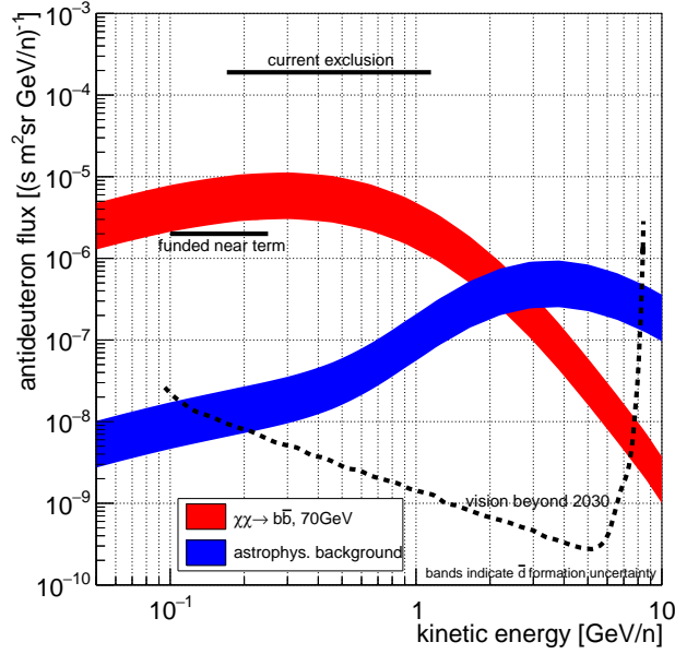
Figure 5: Antideuteron flux from a generic dark matter particle with a mass of 70 GeV annihilating into b\bar{b} compared to the astrophysical background flux prediction, which is orders of magnitude smaller. See Ref. [6] for more details.
