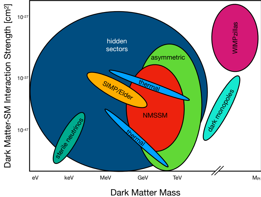
Figure 6: Cartoon figure of the model space for direct detection. Included are candidates of thermal dark matter, supersymmetry, asymmetric dark matter [16], SIMP/Elder [220–223], dark monopoles [226], WIMPzillas [18], and hidden sector dark matter [25]. Note that the interaction cross-section can be for either scattering with nucleons or electrons, depending on the specific model.
