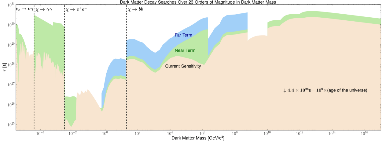
Figure 4: Current and expected sensitivity to DM decay, achieved by cosmic-ray and gamma-ray experiments, for both current (beige) and future (green, blue) searches. Over 23 orders of magnitude in DM mass can be searched, from sterile neutrino decays at keV energies to DM decaying to gamma rays (40 keV–MeV), electrons and positrons (MeV–10 GeV), and bottom quarks ( >10 GeV). Lifetime values are based on results in Refs. [71, 72, 157, 158, 163, 170, 194–207]. Note that the sharp edges of the curves at most masses are due limited mass ranges of published dark matter results, rather than being from instrumental thresholds.
