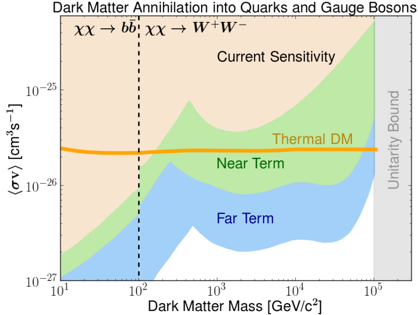
Figure 3: Current and expected sensitivity to s -wave DM annihilation to quarks and gauge bosons, achieved by space-based and ground-based high-energy gamma-ray experiments, for both current (beige) and future (green, blue) searches. Cross section values are extracted from Refs. [150, 157, 160–162], as well as far-future sensitivities as described above.
