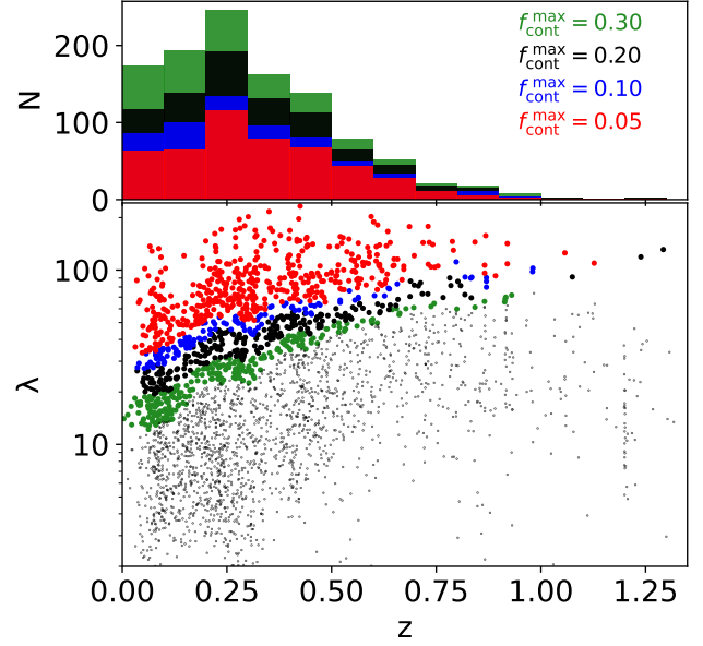
Figure 6. top: Redshift distribution of the 2,913 Planck candidates. The green, black, blue and red histograms show the distributions of candidates with f_{\text{cont}} below f_{\text{cont}}^{\text{max}} = 0.3, 0.2, 0.1 and 0.05 , respectively. bottom: Richness versus redshift for the best optical counterpart for each Planck candidate. Pairs with a probability of being random superpositions (contamination) f_{\text{cont}} > 0.3 are shown as small black dots. Bigger green, black, blue and red dots represent counterparts with 0.2 \leq f_{\text{cont}} < 0.3 , 0.1 \leq f_{\text{cont}} < 0.2 , 0.05 \leq f_{\text{cont}} < 0.1 and f_{\text{cont}} < 0.05 , respectively, corresponding to subsamples with decreasing contamination.
