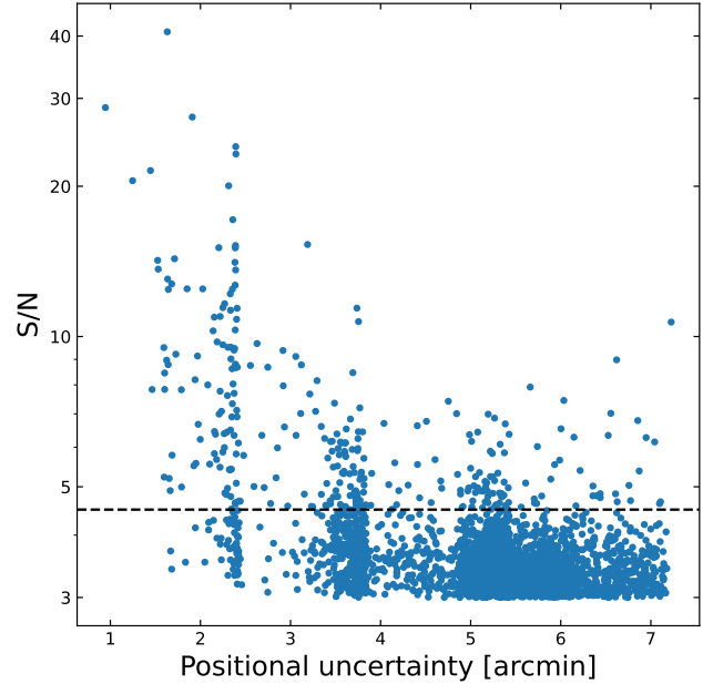
Figure 2. Positional uncertainty distribution in units of arcminutes versus Planck candidate S/N . The mean and median of the sources with S/N < 4.5 are 5.26 arcmin and 5.36 arcmin, respectively. The black dashed line represents the threshold at S/N=4.5 .
