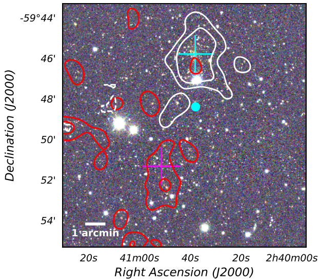
Figure D1. top: Richness as a function of redshift for the Planck source PSZ-SN3 J0240-5945, with the best fit peak at z_{\text{MCMF}} = 0.41 . bottom: pseudo-color image from DES g, r, i bands near the Planck candidate coordinates, which are marked with a cyan dot. Contours are from the galaxy density maps of the counterpart at z_{\text{MCMF}} = 0.41 (white) and at z_{\text{MCMF}} = 0.605 (red). The cyan cross marks the position of the optical counterpart found using MCMF, and the magenta cross marks the position of PSZ2 G280.76-52.30.
