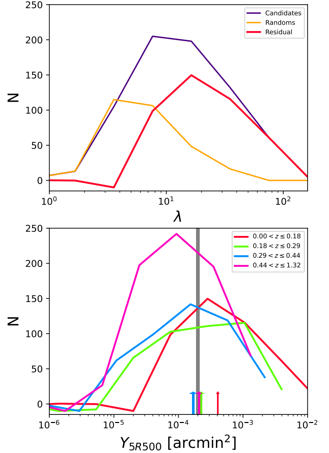
Figure E2. top: Richness distributions in the redshift range 0 < z_{\text{MCMF}} \leq 0.18 of candidates, rescaled randoms and excess candidates shown as purple, orange and red lines, respectively. bottom: Y_{5R500} distributions of excess candidates for different redshift bins. Y_{5R500} is determined from \lambda_{\text{MCMF}} using scaling relations. Colored arrows correspond to the richness derived Y_{5R500} a candidate would need to have for us to consider it a real cluster in our sample, estimated using the median redshift of all the candidates for each redshift bin. The gray line marks the Y_{5R500}^{\text{min}} used to estimate the purity in Section 2.2.
