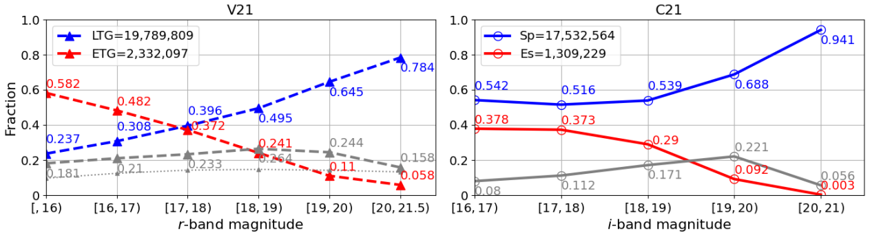
Figure 3. Fraction of Es/ETG (red), Sp/LTG (blue) and galaxies with uncertain classifications (grey) with respect to the total in r and i -band magnitude bins for the V21 (left) and C21 (right) catalogues. The grey dotted line in the left panel (V21) are uncertain galaxies excluding ‘secure intermediate’ classification (see Section 2.3 for the definition of each class).
