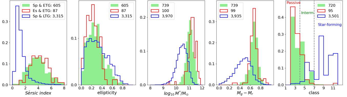
Figure 11. Normalised distributions of Sérsic index, ellipticity, stellar mass, absolute colour M_g - M_r (from VIPERS), and unsupervised spectral classification from Siudek et al. (2018b) are presented. The green shaded histograms show the distributions of Sp & ETG. The solid red and blue lines are the distributions of Es & ETG and Sp & LTG, respectively, for comparison.
