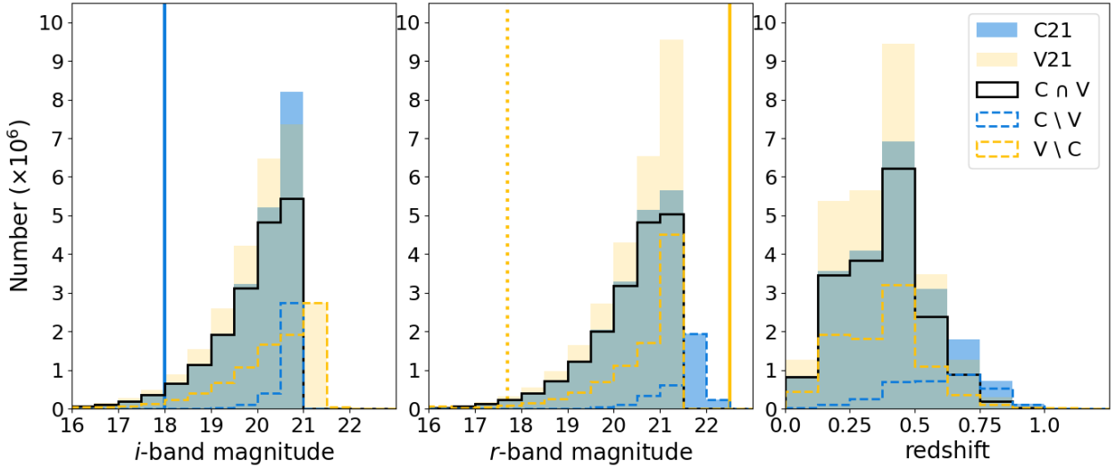
Figure 1. The magnitudes and redshift distributions of C21 (blue filled histogram), V21 (light yellow filled histogram), and different subsets of them presented by different lines. The overlapped area is represented as the mix of blue and yellow, i.e. slightly darker blue/green. For lines, the solid black lines show the intersection of both catalogues. The blue dashed lines and the yellow dashed lines are for samples only in C21 ( C \setminus V ) and only in V21 ( V \setminus C ), respectively. The vertical lines indicate the upper limit of magnitudes in the training samples such that the blue solid line is for the one of C21 ( i < 18 ), the yellow dotted line shows the upper magnitude limit of the initial bright galaxies used in V21 ( r < 17.7 ), and the yellow solid line represents the one of the final training samples in V21 including emulated faint galaxies ( r < 22.5 ).
