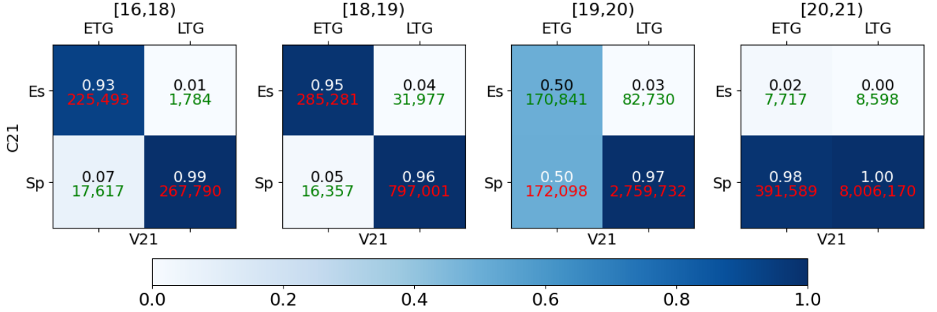
Figure 6. Confusion matrices of CNV samples in different magnitude bins. This uses V21 classification as the reference. Each quadrant shows a different combination of classifications provided by the two catalogues. The red or green text in each quadrant represent the number of galaxies that agrees with the classifications from C21 and V21 within each quadrant. The number above this text indicates the fraction of these galaxies within each certain type decided by V21 classification. Each quadrant is coloured using this fraction, according to the scalebar.
