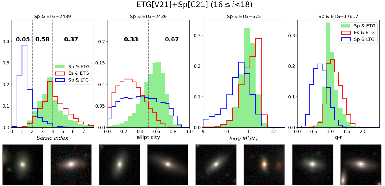
Figure 8. Top: the normalised distribution of Sérsic index, ellipticity, stellar mass, and apparent colour ( g-r ) from left to right. The light green histograms represent Sp & ETG while the red and blue lines show the case of Es & ETG and Sp & LTG, respectively, for comparison. The grey dashed vertical lines note Sérsic index = 2.0 and 4.0 and ellipticity = 0.5. The textual information within each area separated by the grey lines shows the fraction of samples with Sp & ETG in each range. Bottom: randomly selected example images of the mismatched case, Sp & ETG.
