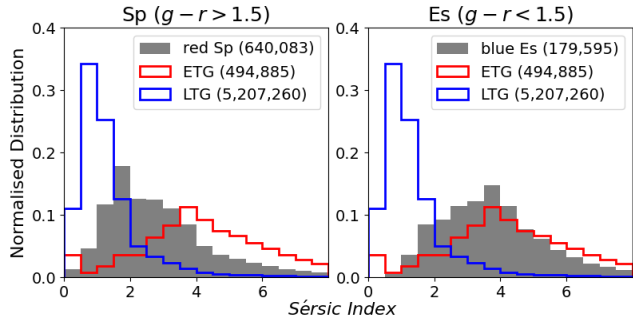
Figure 14. The shaded histograms show the normalised Sérsic index distributions of red Sp with g-r > 1.5 (left) and blue Es with g-r < 1.5 (right) from C21. The blue and red solid lines show the Sérsic index distributions of LTG and ETG from V21, respectively, for comparison. The number of data in each class that have Sérsic index measurements is shown within brackets in the legend.
