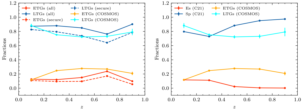
Figure 4. Fraction of morphological classes as a function of redshift for the V21 (left) and the C21 (right) catalogues. Es/ETG (red) are compared with the galaxies classified as ETG in COSMOS (orange) and Sp/LTG (blue) are compared to galaxies classified as Spirals and Irregulars in COSMOS (cyan). For the V21 sample the results are shown for the full (solid lines) and the secure (dashed lines) samples (defined in Section 2.3). COSMOS galaxies are selected in a similar way as the corresponding morphological catalogue: 6909 galaxies have r < 21.5 mag and R_e > 2.8 pixels when compared to V21, and 10350 galaxies have i < 21.5 mag and no cut in radius when compared to C21. Vertical error bars are computed assuming Poisson error (i.e., considering that the error in the number of galaxies is \sqrt{N} ).
