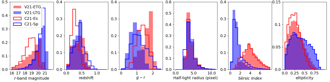
Figure 13. Normalised distributions of r -band magnitude, redshift, apparent colour ( g-r ), half-light radius, Sérsic index, and ellipticity. The shaded histograms show galaxies with robust classification from V21 while solid lines are for C21. Red and blue colour indicates Es/ETG and Sp/LTG, respectively.
