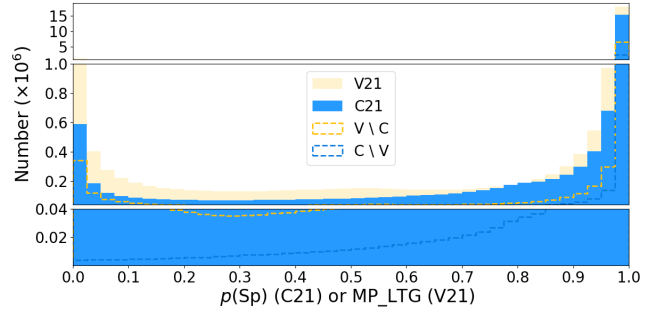
Figure 2. Distributions of mean/median probabilities of being Sp (C21; p(\text{Sp}) ) or LTG (V21; \text{MP\_LTG} = \text{median}(P_i) , where P_i is defined in Section 2.3). The light yellow and blue histograms represent all the galaxies in V21 and C21, respectively, while the dashed lines show the galaxies included in only one of the two catalogues (light yellow for V21 and blue for C21). The y -axis is truncated at different scales for optimal visualization.
