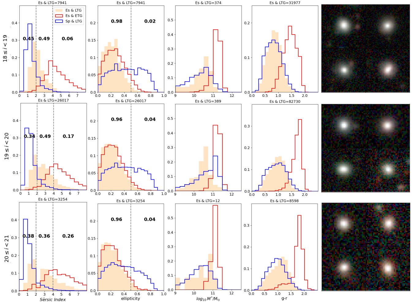
Figure 12. Normalised distributions of Sérsic index, ellipticity, stellar mass, and apparent colour, g - r , for Es & LTG are presented from left to right, and the last panel shows randomly selected examples of Es & LTG within each magnitude range. The orange shaded histograms show the distributions of Es & LTG. The number of Es & LTG used to plot the orange shaded histograms is shown above each graph. The solid red and blue lines are the distributions of Es & ETG and Sp & LTG, respectively, for comparison. The grey dashed lines note Sérsic index = 2.0 and 4.0 and ellipticity = 0.5. The textual information within each area separated by grey lines shows the fraction of samples with Es & LTG in each range.
