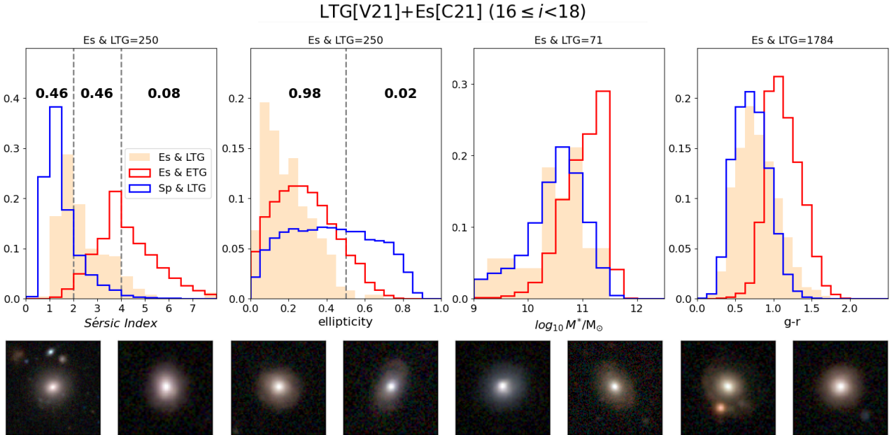
Figure 9. Top: the normalised distribution of Sérsic index, ellipticity, stellar mass, and apparent colour ( g-r ) from left to right. The light orange histograms represent Es & LTG while the red and blue lines show the case of Es & ETG and Sp & LTG, respectively, for comparison. The grey dashed lines note Sérsic index = 2.0 and 4.0 and ellipticity = 0.5. The textual information within each area separated by the grey lines shows the fraction of samples with Es & LTG in each range. Bottom: randomly selected example images of the mismatched case, Es & LTG.
