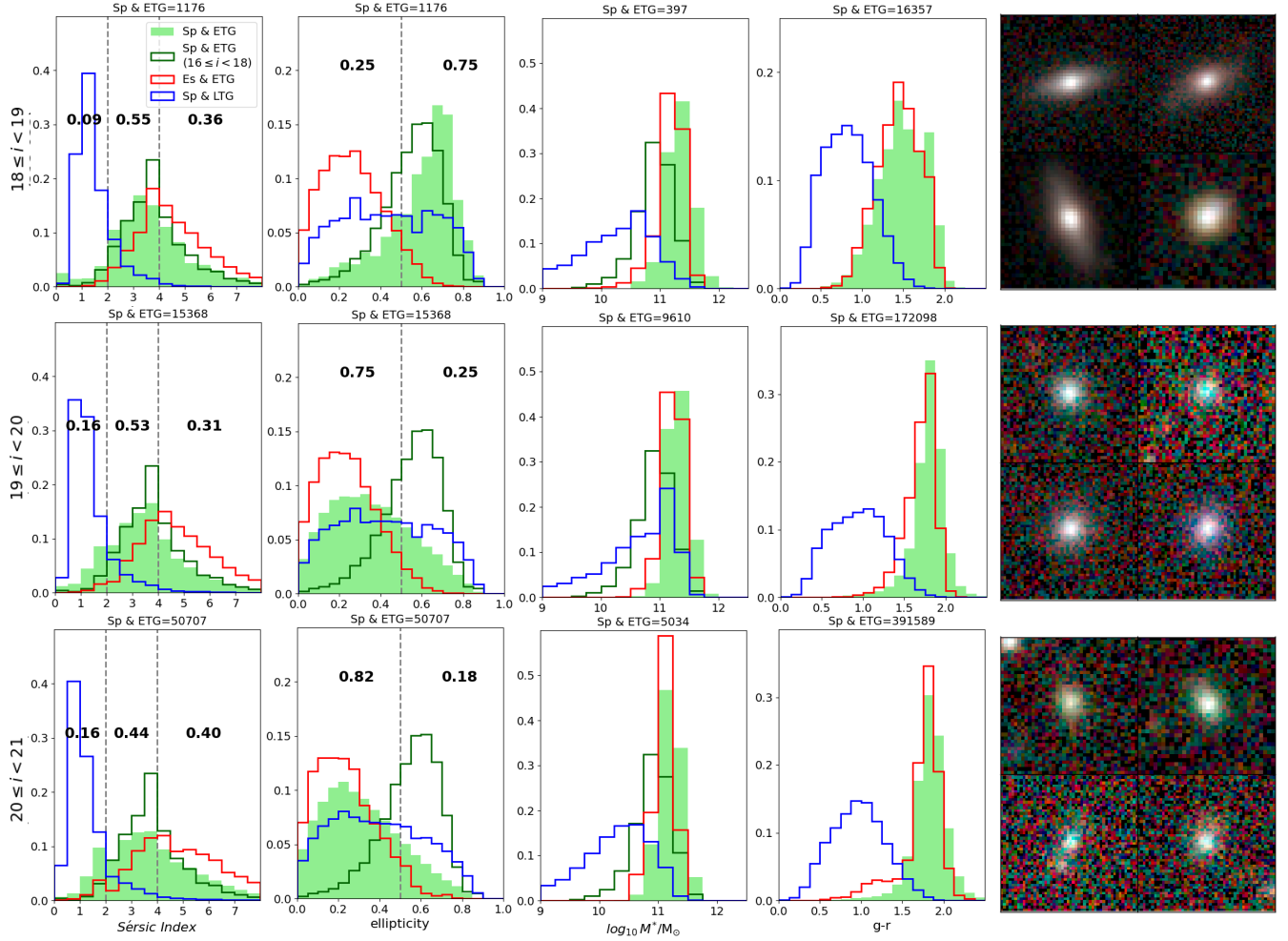
Figure 10. Normalised distributions of Sérsic index, ellipticity, stellar mass, and apparent colour, g - r , are presented from left to right, and the last panel shows randomly selected examples of Sp & ETG within each magnitude range. The green shaded histograms show the distribution of Sp & ETG within each magnitude range. The number of Sp & ETG galaxies that are used to construct the green shaded histograms is shown above each graph. Solid red and blue lines are the distribution of Es & ETG and Sp & LTG, respectively, for comparison. The solid dark green lines show the distributions of the Sp & ETG case with 16 \leq i < 18 for comparison. The grey vertical dashed lines note Sérsic index = 2.0 and 4.0 and ellipticity = 0.5. The textual information within each area separated by the grey lines shows the fraction of samples with Sp & ETG in each range.
