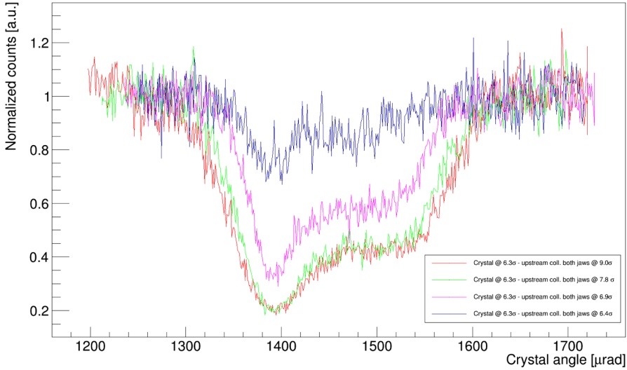
STF18 - angular scans at different apertures of upstream collimator
